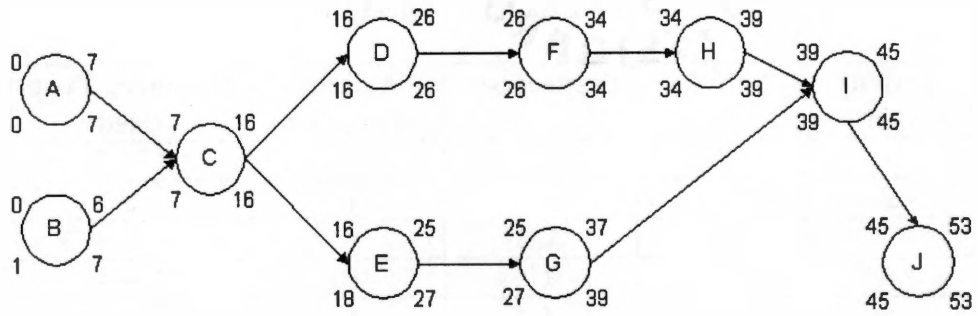
Figure 4.13 CPM Analysis
