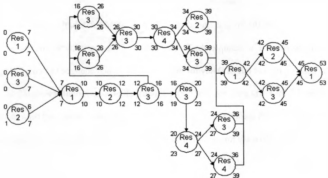
Figure 4.24 CRD Analysis
