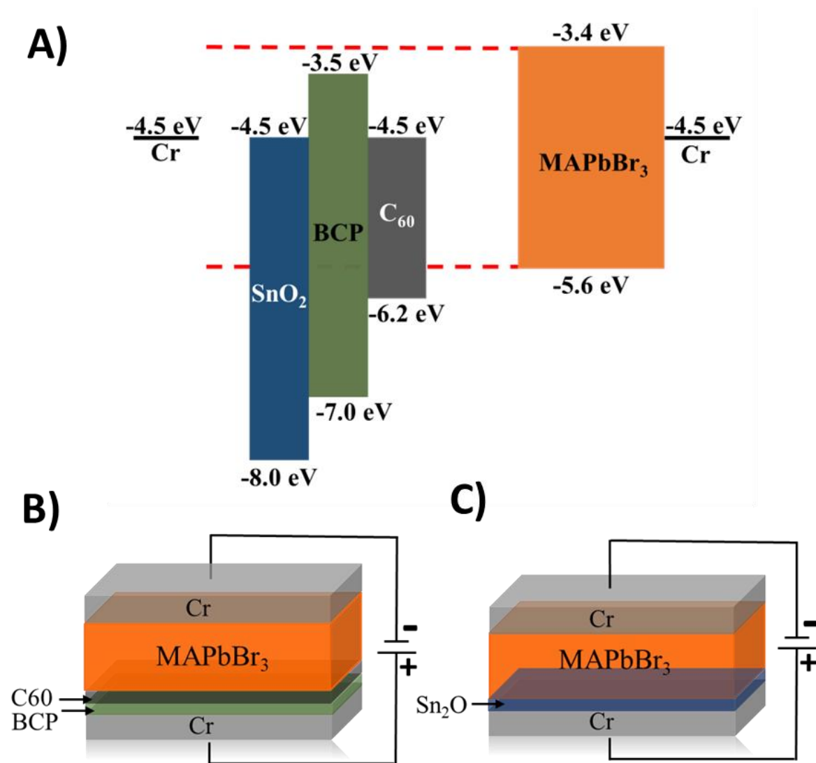
Figure 3.3.1. A) Band structure comparison between MAPB and several interfacial materials. Pictorial representation of the contact scheme B) E1 and C) E2
