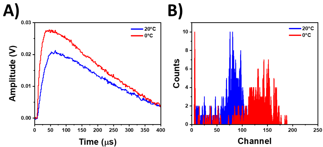
Figure 3.7.4. A) Preamplifier traces from LiMAPb detector exposed to ^{210}\text{Po} alpha particles at -60 V showing a faster rise time at 0°C compared to room temperature B) Alpha spectrum of the same experiment with ^{210}\text{Po} alpha source (Bias: -60 V, Gain: 50, Shaping Time: 10 μs, Count Time: 120 s)
