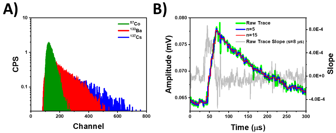
Figure 3.5.1. A) Background subtracted spectra from various gamma ray sources with a 5.1 \times 4.7 \times 1.2 mm LiMAPB detector biased at -120 V (Gain: 50, Shaping Time: 10 \mu\text{s} ), B) The effect of smoothing on a raw radiation induced trace, with the slope between two points on the signal spaced 8 \mu\text{s} shown in gray, which was used to set the threshold for determining the start of the rise
