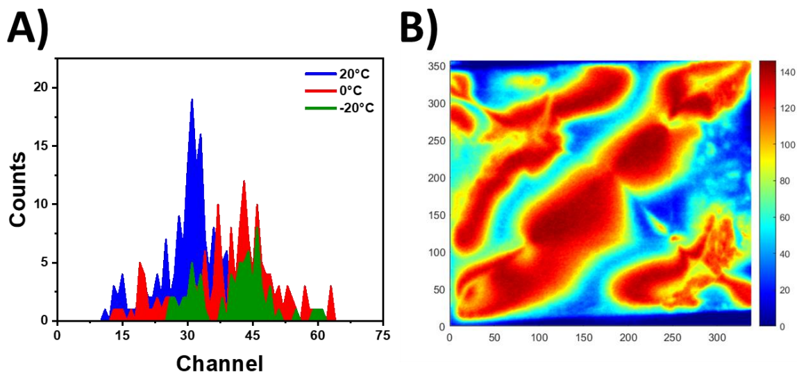
Figure 3.7.5. A) Alpha spectrum with noise floor removed at various temperatures in MAPbBr 2.85 Cl 0.15 with ^{210}\text{Po} alpha source (Bias: -50 V, Gain: 100, Shaping Time: 10 μs, Count Time: 120 s) B) Birefringence image of the MAPbBr 2.85 Cl 0.15 detector showing poor quality
