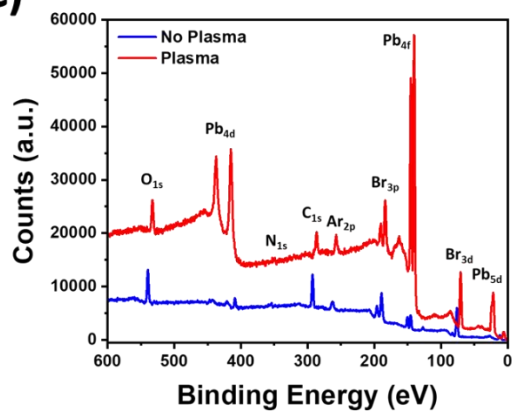
Figure 3.2.6. A) Image of a MAPB sample after 95% Ar/5% O 2 plasma cleaning in a Harrick Plasma Cleaner for several minutes, B) High resolution XPS scan of the Pb 4f region for MAPB with and without plasma cleaning, C) XPS survey scan of MAPB with and without plasma cleaning
