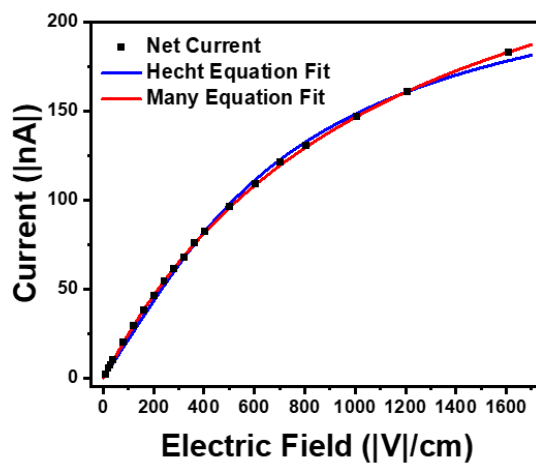
Figure 3.1.7. Hecht and Many fits for X-ray induced current as a function of electric field in 3D polycrystalline MAPB wafers A) MAPB A and B) MAPB B
