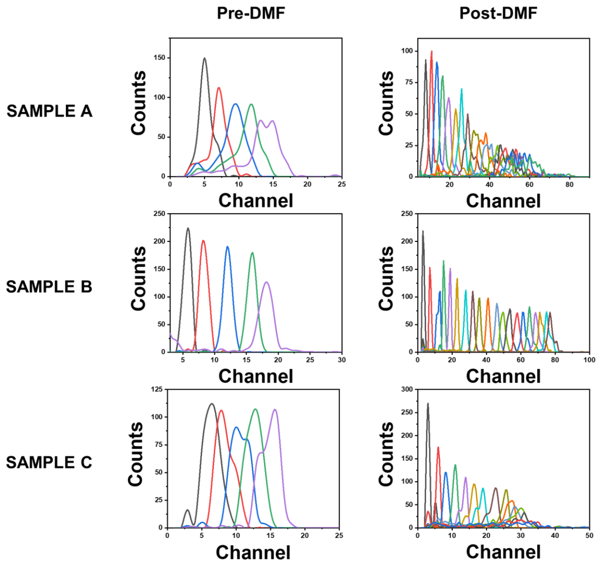
Figure 3.2.5. Spectral comparison between three MAPbBr 2.85 Cl 0.15 samples exposed to a 210 Po radiation source before and after DMF Polishing. The bias range used for each plot are provided in Table 3.2.1
