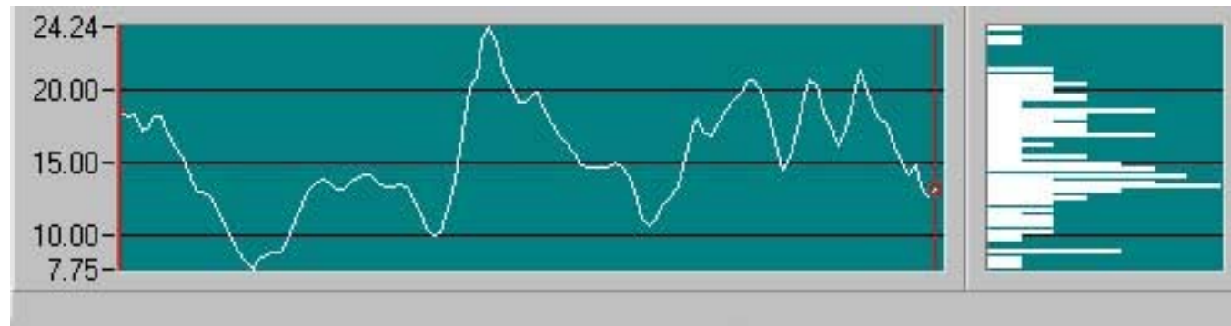
Figure A-23 Experimental Time Dependent Velocity at a Horizontal Centerline Position of 2 Inches (60 Degree Die – 2 psig Back Pressure)
