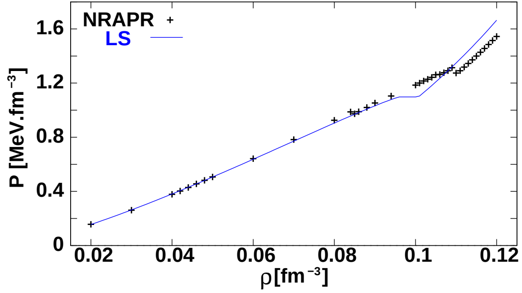
Figure 4.5: Pressure versus density for the NRAPR interaction and the Lattimer-Swesty EoS. The transition to uniform matter happens at different densities since they are two different models.
