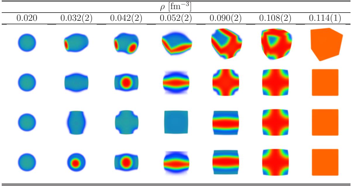
Figure 4.1: First row: Pasta phases calculated using the SQMC700 Skyrme interaction, T = 2 MeV and y_p = 0.3 . Rows 2, 3, 4: 2D projection of the pasta phases on the (y,x), (x,z) and (y,z) planes, respectively. The neutron density distribution is shown at the density corresponding to the onset of each phase, known with the uncertainty given in brackets. Blue (red) color indicates the bottom (top) of the density scale: 0.001 (dark blue) - 0.02475 (light blue) - 0.0485 (green) - 0.07225 (light orange) - 0.095 (red) \text{fm}^{-3} . The pasta formation shown here appears for all the Skyrme models, but the threshold density changes somewhat, see Fig. 4.4.
