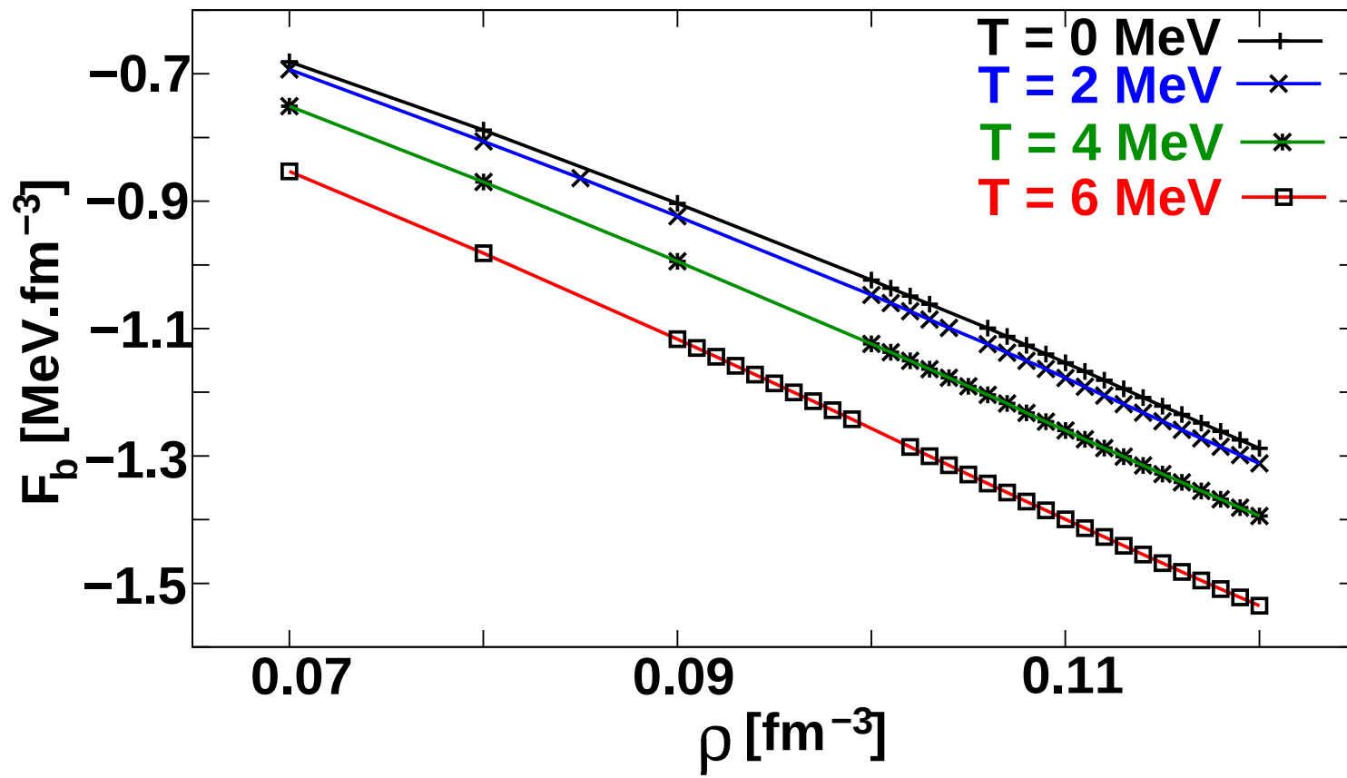
Figure 4.8: Baryonic free energy density as a function of the number density for the NRAPR Skyrme interaction and T = 0, 2, 4 and 6 MeV.
