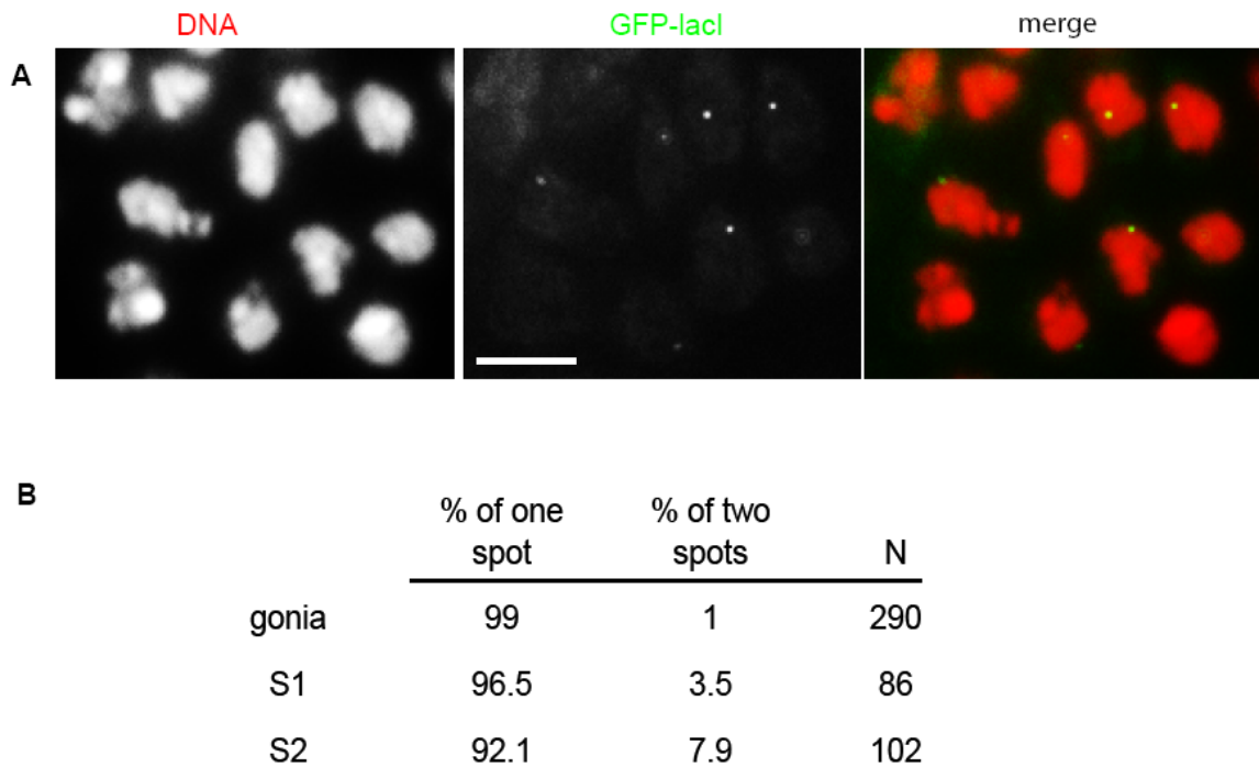
Figure 2-5. Arm cohesion in spermatogonia and early prophase I spermatocytes in solo males hemizygous for an inserted lacO array on chromosome 2.
