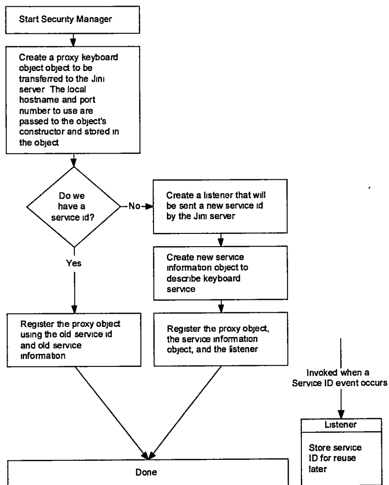
Figure 5 7 Service flowchart
