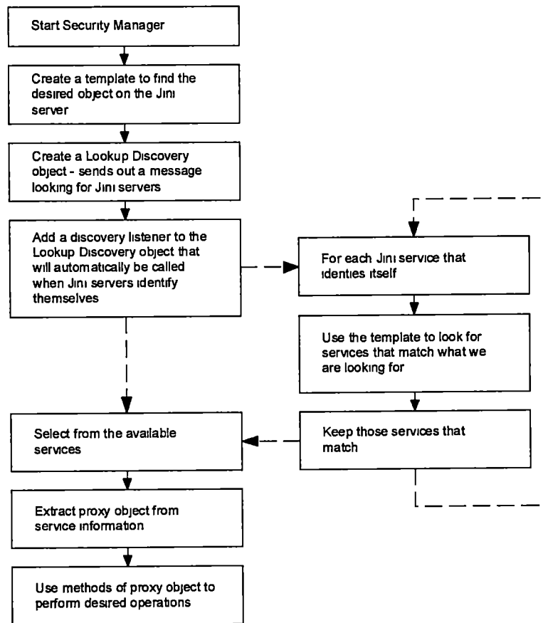
Figure 5 8 Client flowchart
