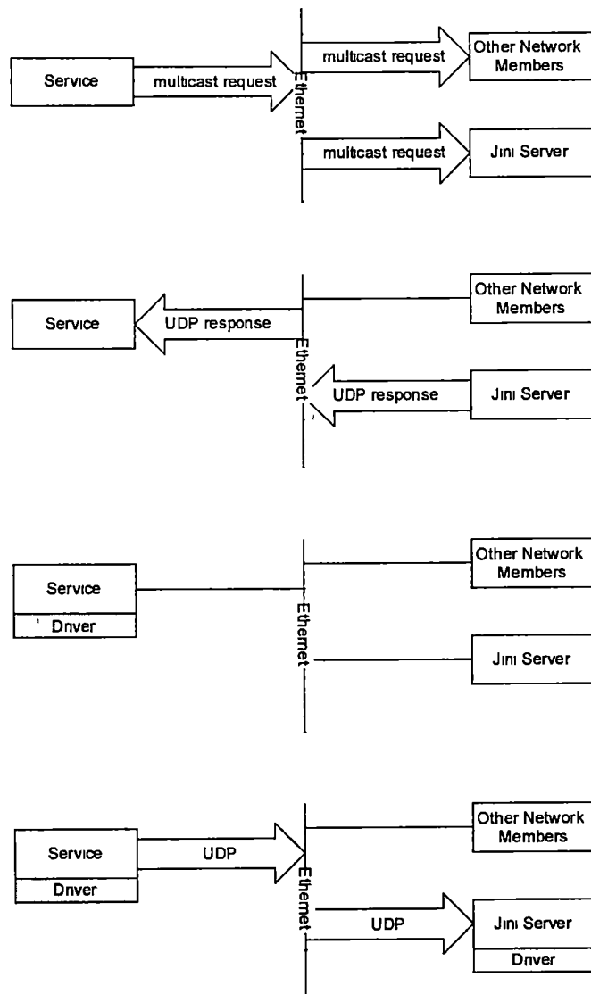
Figure 4 4 Discovery / Join
