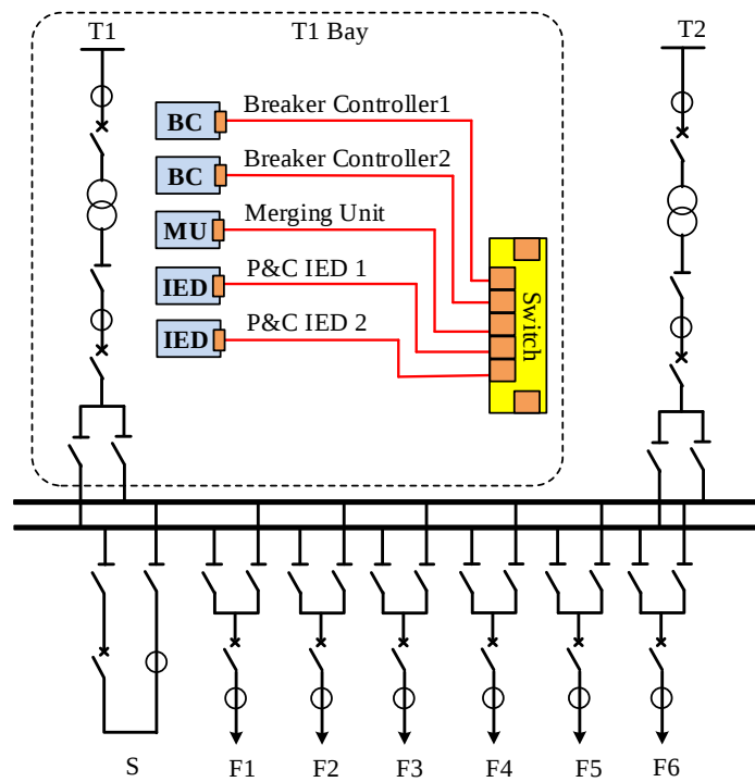
(a) Component connection diagram
