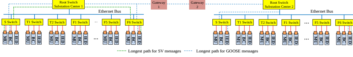
Fig. A1. Diagram of network connection of two substations.
