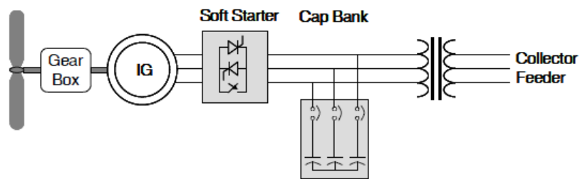
(a) Type 1 WECS
