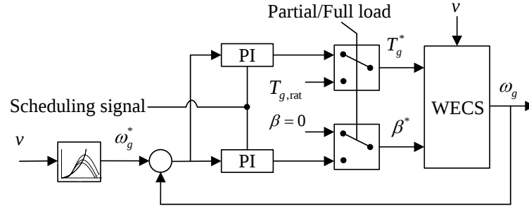
Fig. 3–6. Block diagram of classic WECS control.
