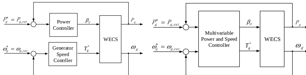
Fig. 2–3. Decentralized control method.
