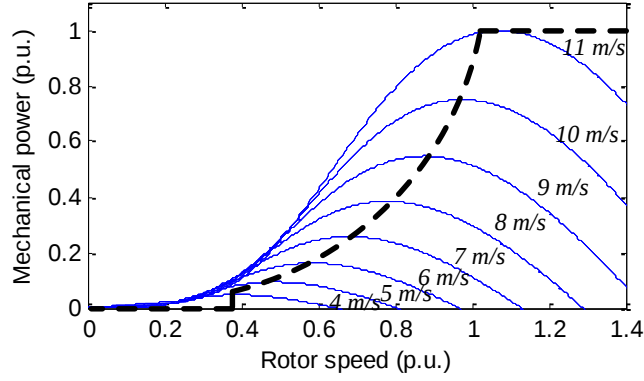
Fig. 3–2. Wind turbine characteristic curves at various wind speeds.
