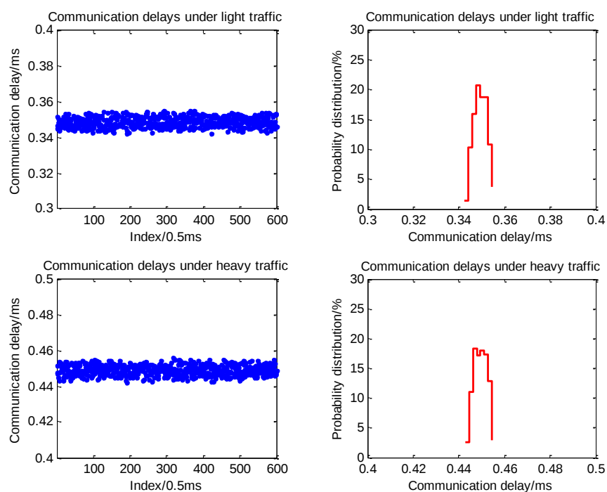
Fig. 4–10. GOOSE delays between two substations: records and statistics.
