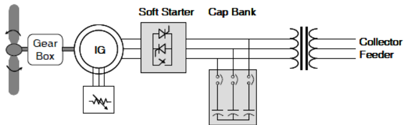
(b) Type 2 WECS
