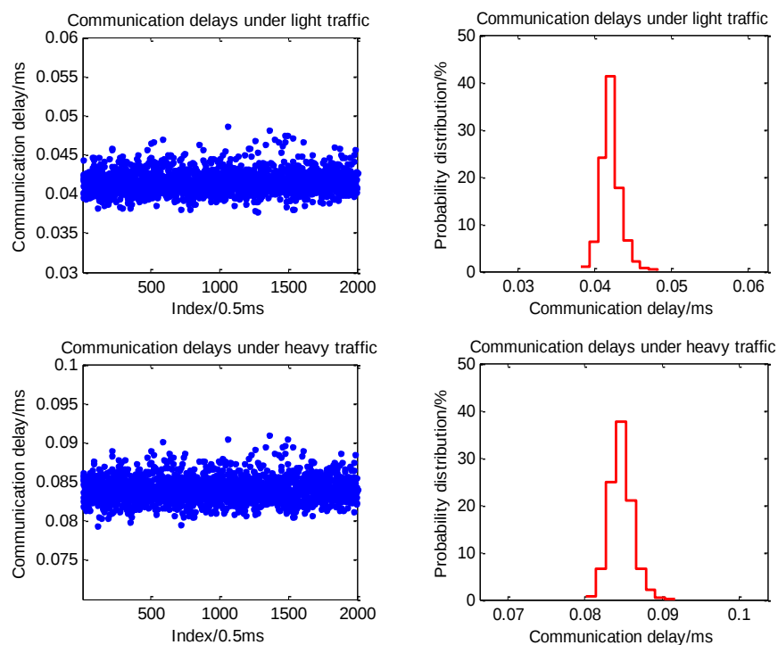
Fig. 4–9. SV delays in a substation: records and statistics.
