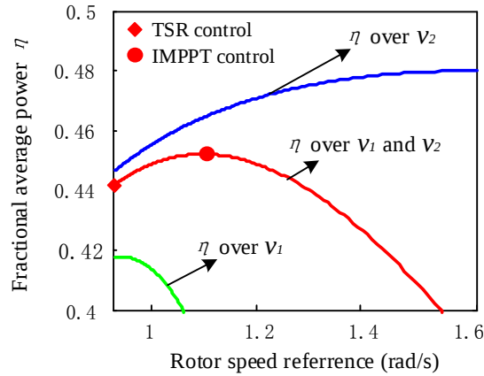
Fig. 3-5. MPPT efficiency with different rotor speed commands.
