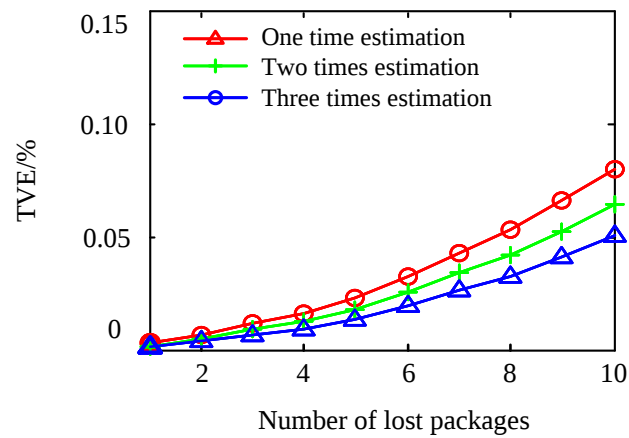
(c) Simulation results in the post-fault state
