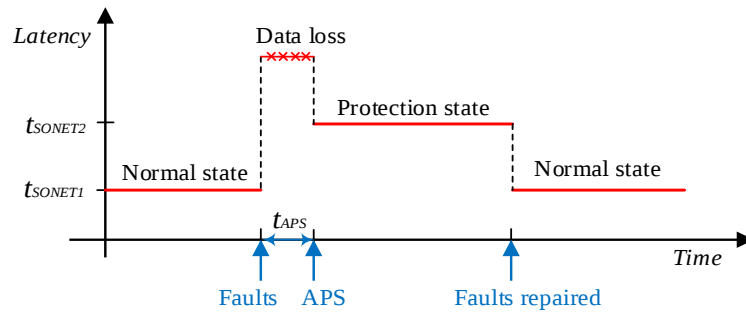
(c) Operating latency of automatic switching
