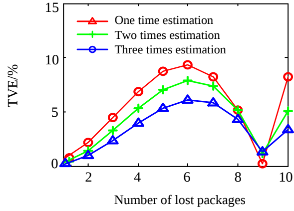
(a) Simulation results in the pre-fault state
