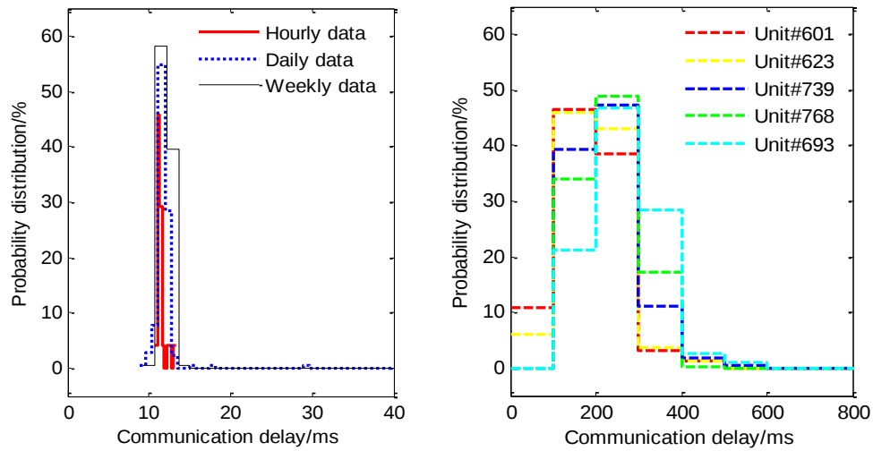
(a) Statistical results of different time spans; (b) Statistical results of different locations.
