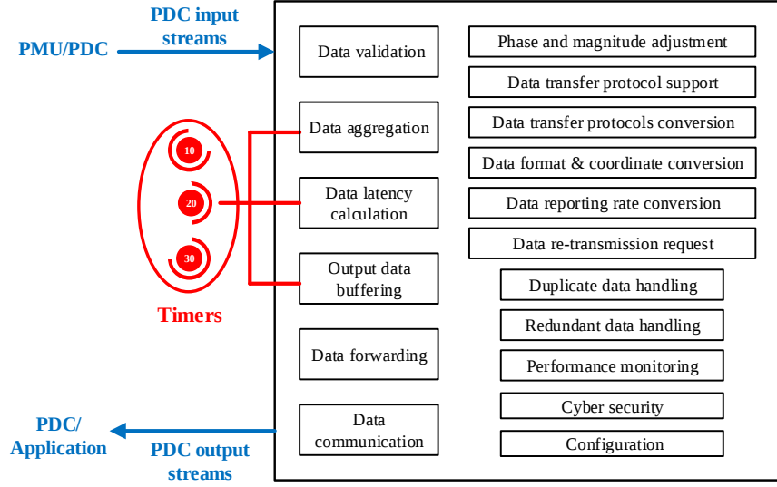
Fig. 4-3. Block diagram of PDC functions.
