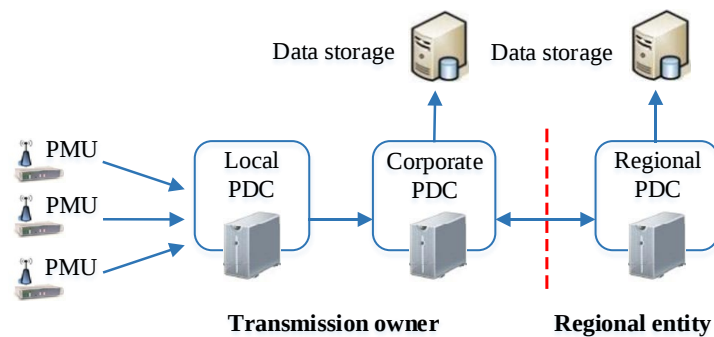
Fig. 1–3. Configuration of a WAMS.
