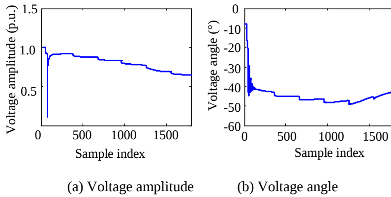
Fig. 5-9. PMU data profile in one minute.
