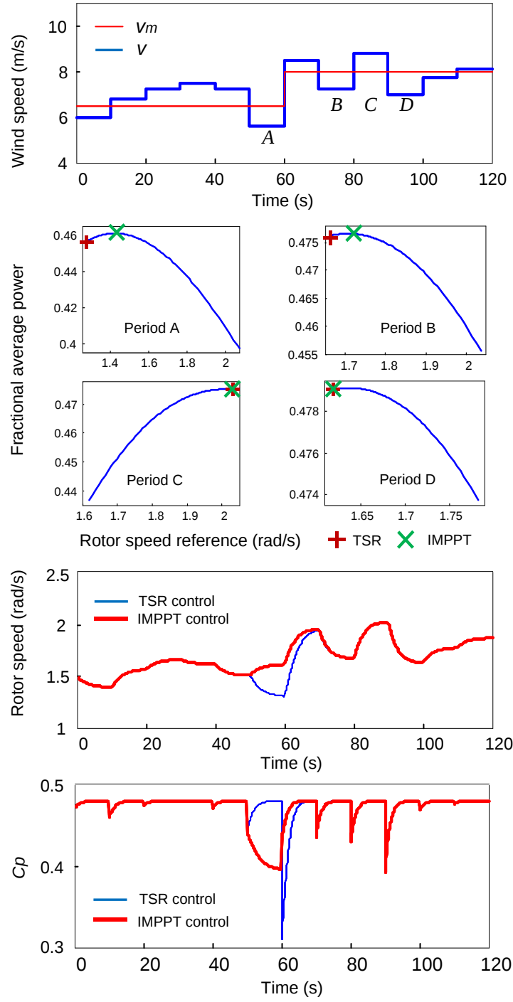
Fig. 3–8. Results of MPPT and IMPPT.
