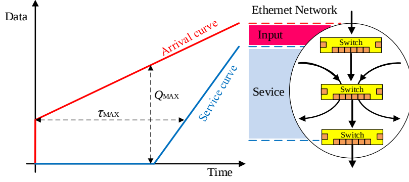
Fig. 4-5. Typical arrival and service curves.
