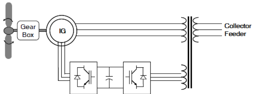
(c) Type 3 WECS
