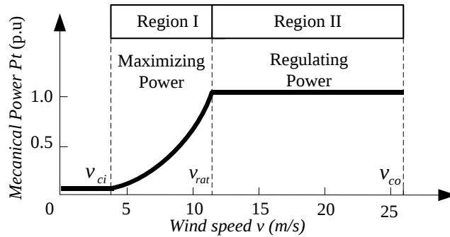
Fig. 2–1. Wind turbine characteristic curve.
