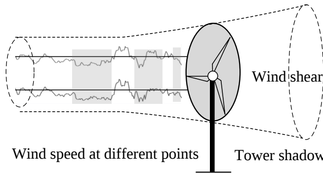
Fig. 2-2. Spatial and temporal distributions of wind speed.
