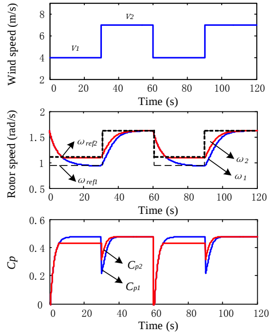
Fig. 3-4. Simulation results of MPPT and IMPPT.
