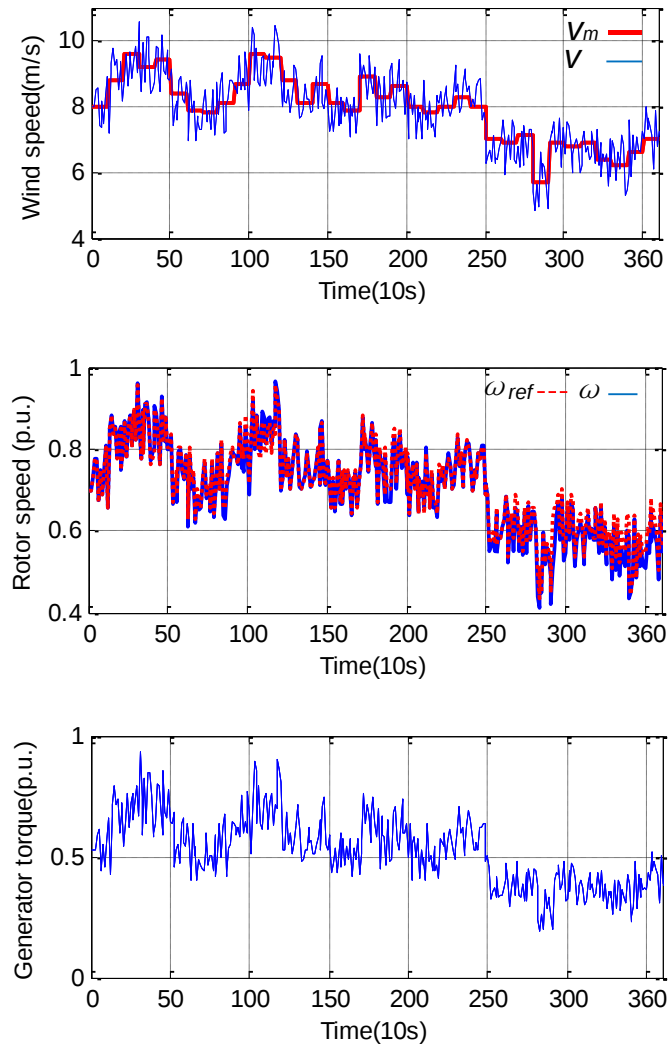
Fig. 3–9. Results of WECS control.
