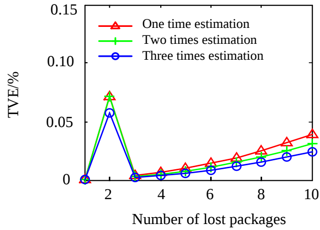
(b) Simulation results in the fault state
