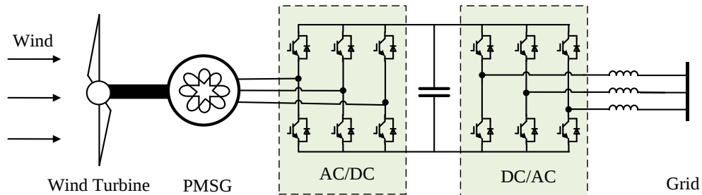
Fig. 3–1. PMSG-based WECS.
