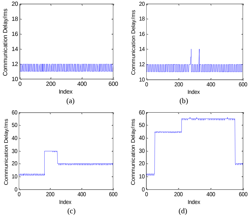
Fig. 4-1. Communication delay measurements in short-term (one minute).
