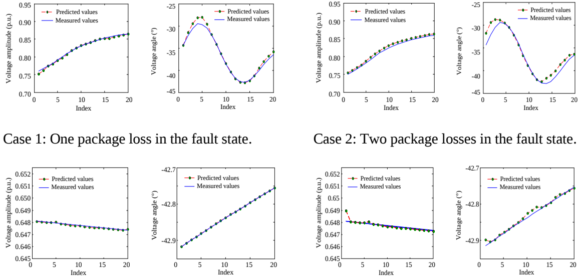
Case 3: One package loss in the post-fault state. Case 4: Two package losses in the post fault state.
