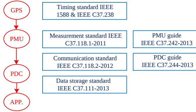
Fig. 2–5. IEEE Standards for synchrophasor systems.
