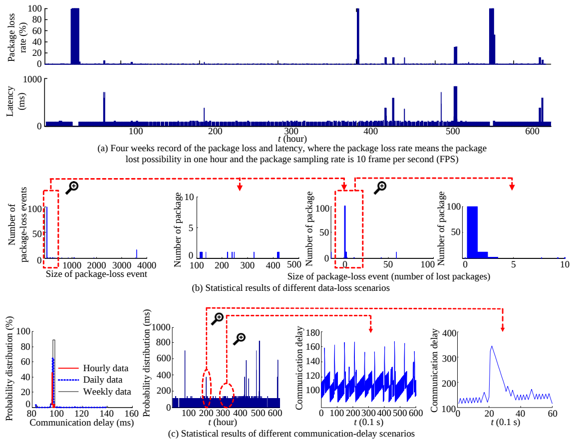
Fig. 5–5. Data loss and latency events in FNET/GridEye.
