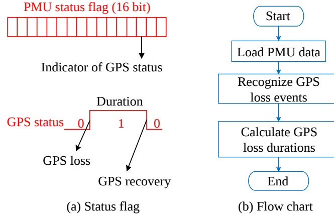
Fig. 5-1. Statistical approaches.
