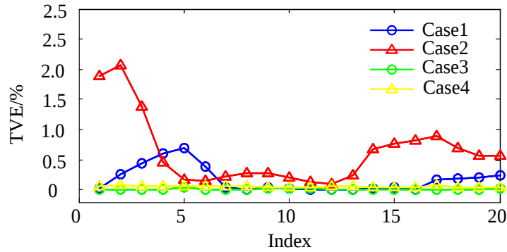
Fig. 5–13. TVE results of the prediction method.
