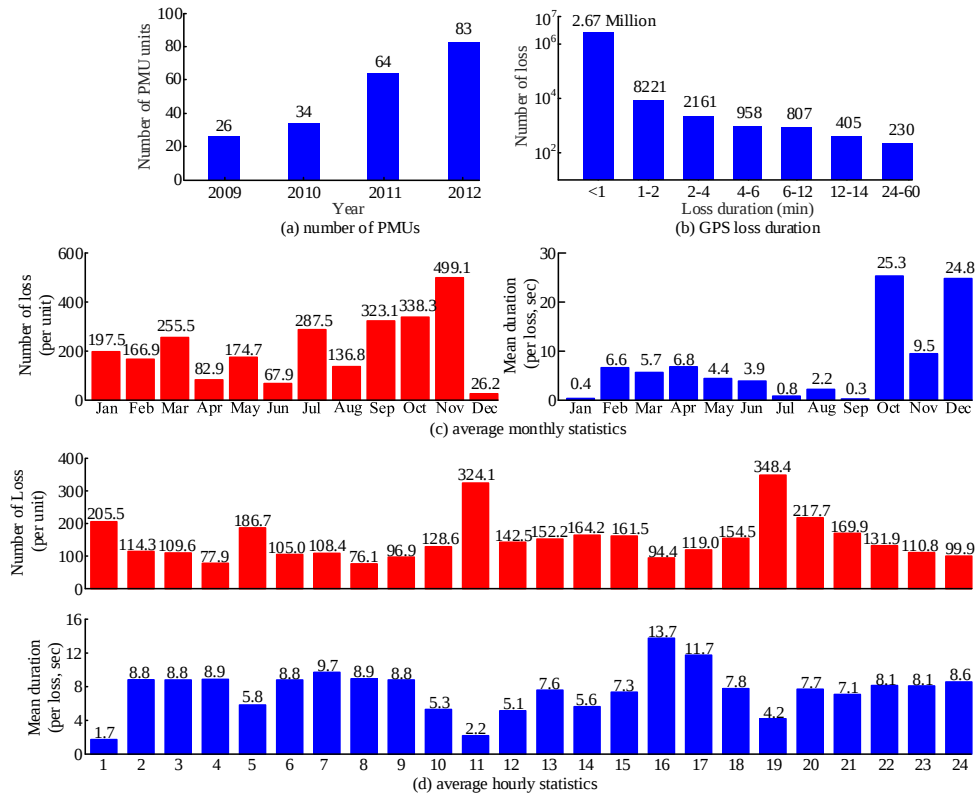
Fig. 5-2. Statistical results of GPS loss events in PMUs from 2009 to 2012.
