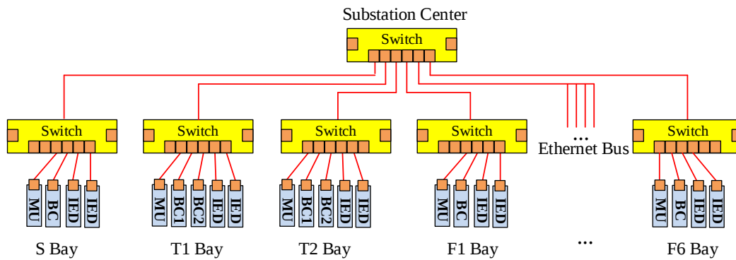
(b) Network connection diagram
