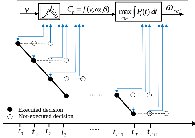
Fig. 3-3. Schematic diagram of IMPPT.
