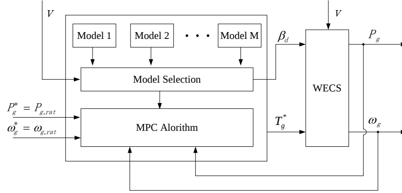
Fig. 2–4. Multivariable MPC method.
