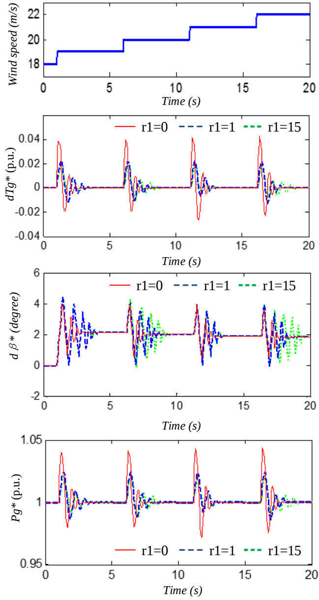
Fig. 3–7. Results of WECS control with different weights.
