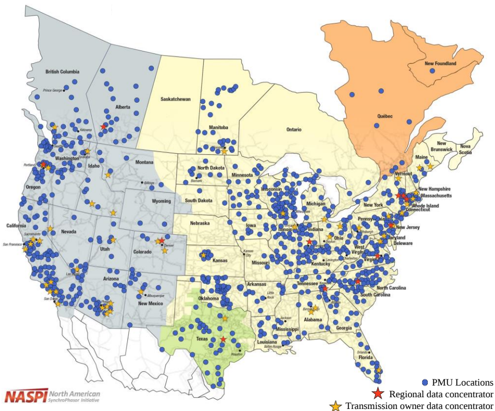
Fig. 1–4. Map of PMU locations in North America.
