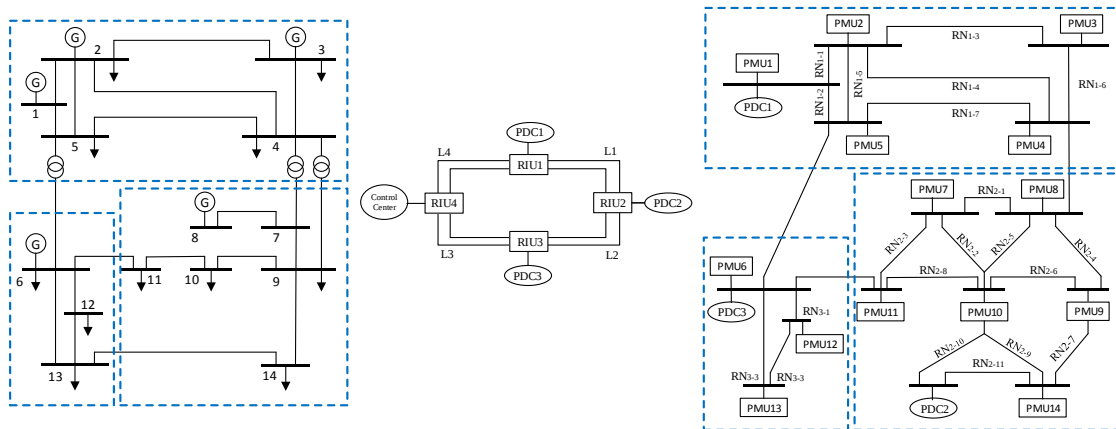
Fig. 4–6. IEEE 14 bus test system.
