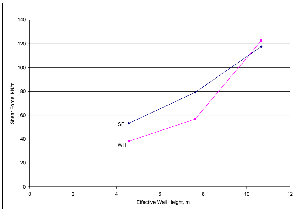
Figure 4.2-10 Maximum Shear in Batter Pile as Function of Wall Height
