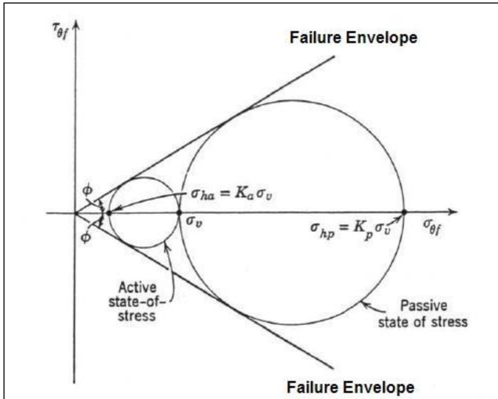
Figure 1.2-1 States of Stress (Lambe and Whitman, 1969)
