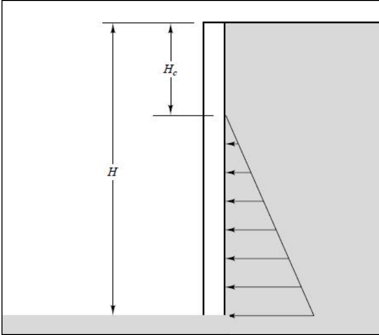
Figure 3.8-1 Theoretical Active Pressure Distribution for Cohesive Soils (Coduto, 2001)
