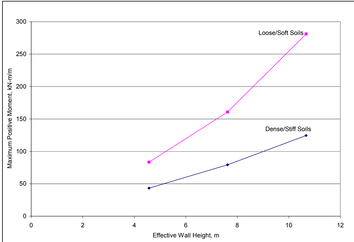
Figure 5.2-1 Design Envelope for Maximum Positive Moment
