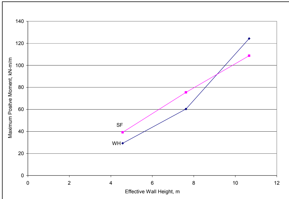
Figure 4.2-9 Maximum Moment in Batter Pile as Function of Wall Height
