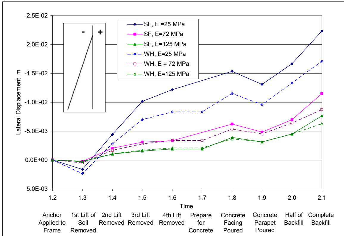
Figure 4.2-18 Effect of Soil Stiffness on Wall Deflection during Construction
