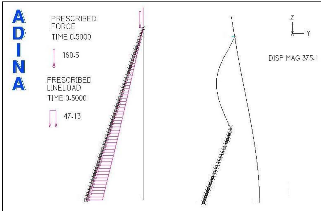
Figure 3.5-5 Simple Frame Analysis Undeformed and Deformed Shapes
