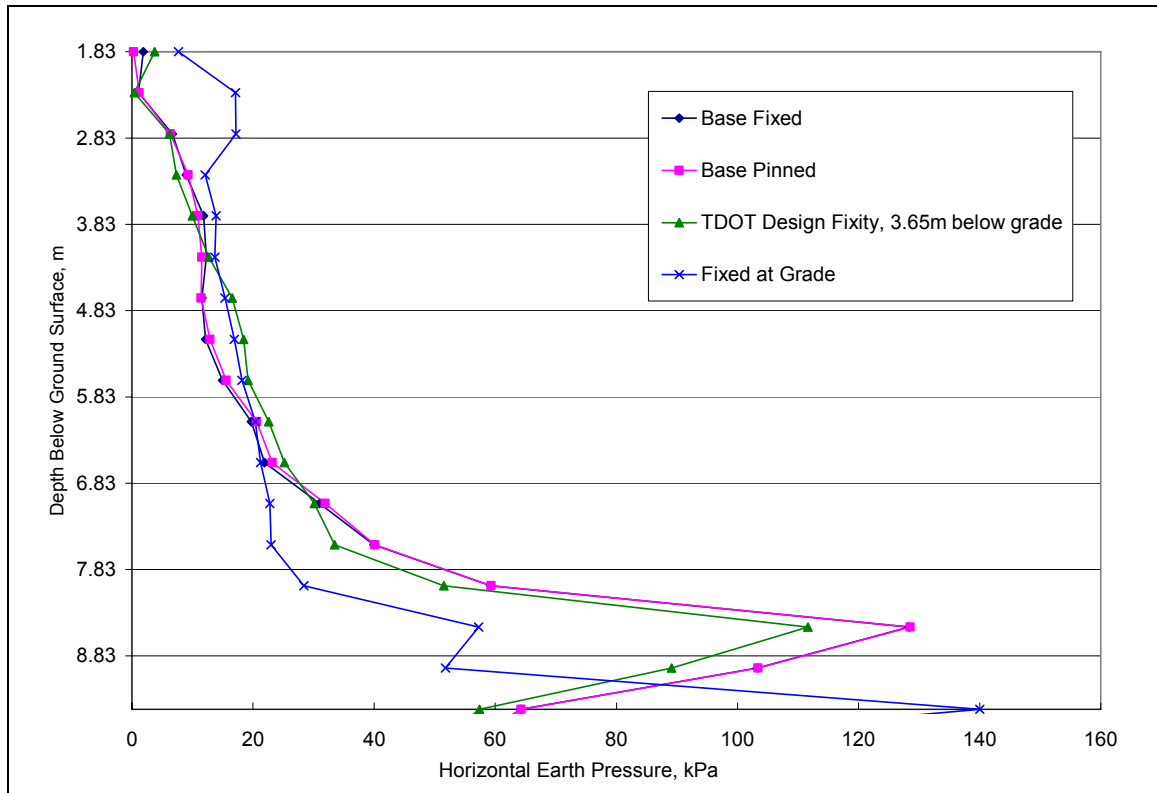
Figure 4.2-5 SF Soil - Effect of Fixity on Earth Pressures
