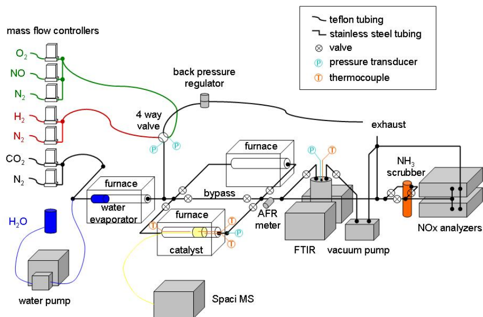
Figure 3.1. Schematic of the Bench Flow Reactor
