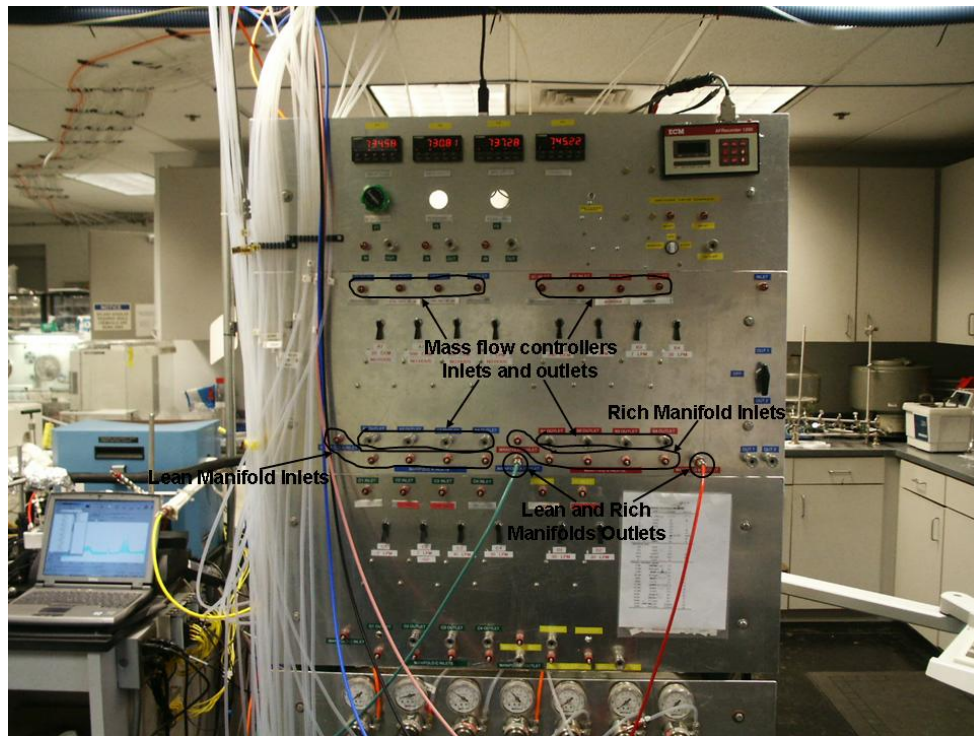
Figure 3.3. Front Panel of the Manifold Setup
