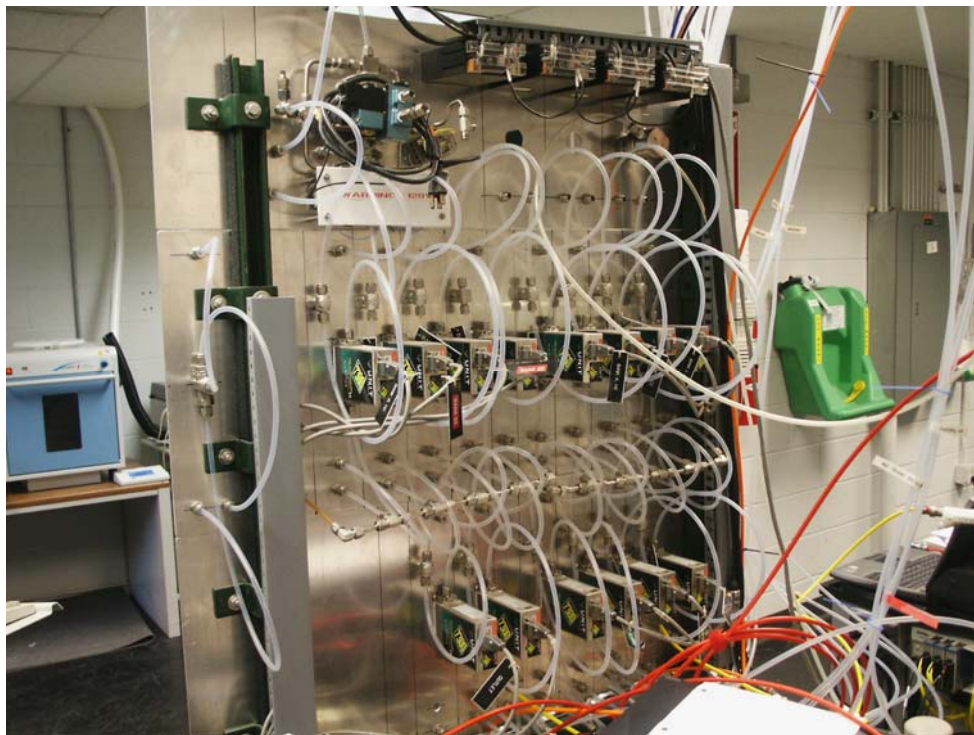
Figure 3.4. Back Panel of the Manifold Setup
