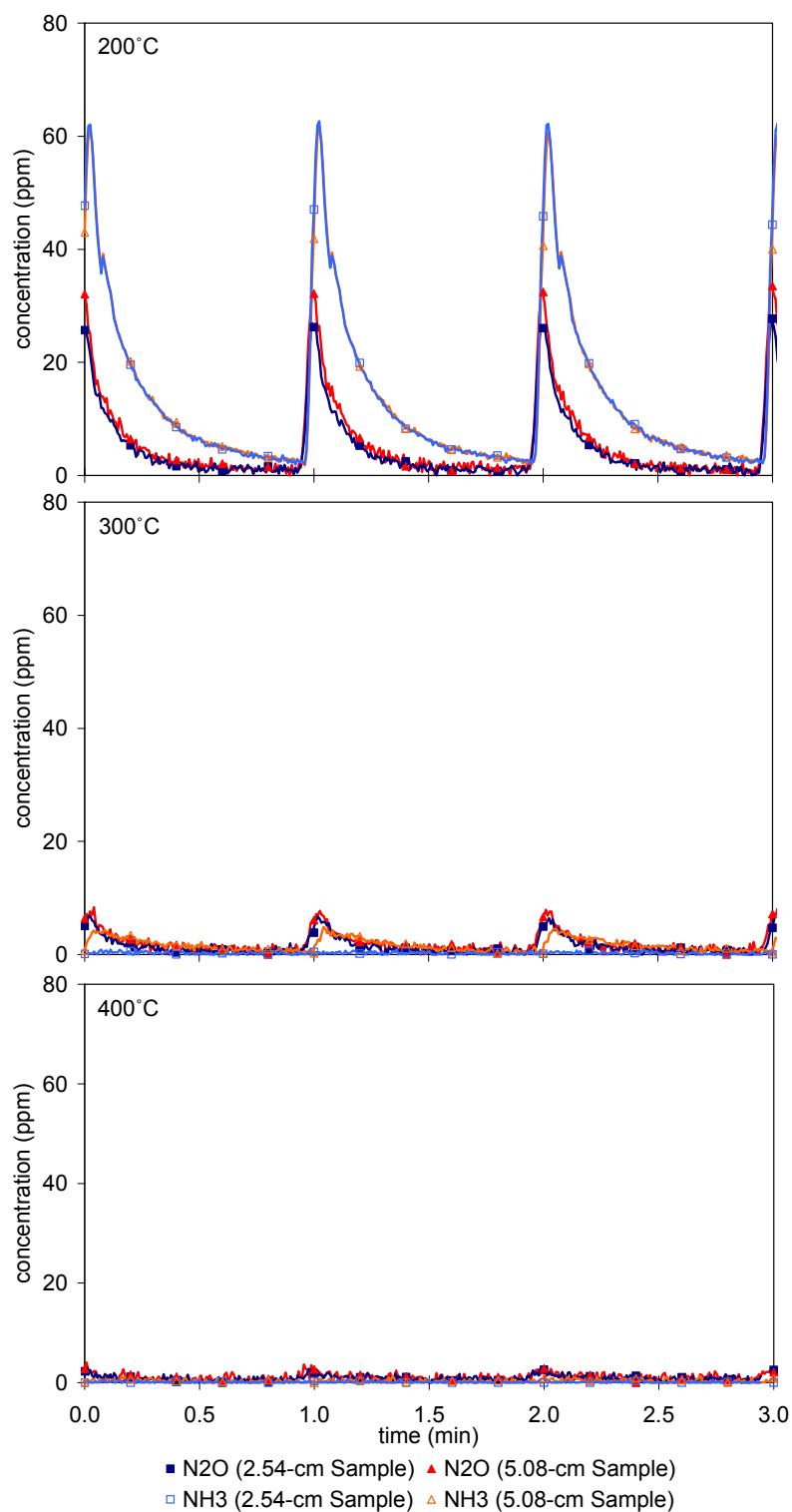
Figure 4.11. Catalyst A's outlet concentrations of \text{N}_2\text{O} and \text{NH}_3 for 2.54 and 5.08-cm-long samples in short-cycle experiments with 1.0% \text{H}_2 in rich phase at 200, 300 and 400°C
