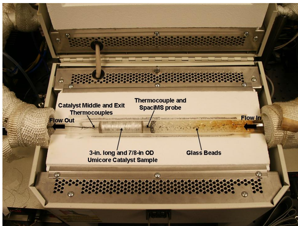
Figure 3.8. Reactor Setup
