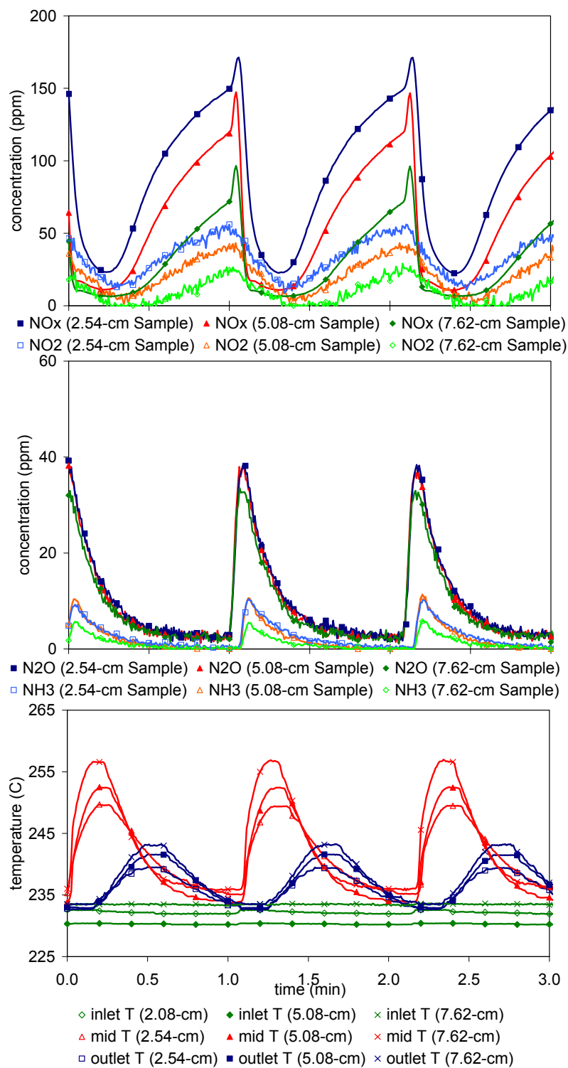
Figure 4.30. Catalyst B's outlet gas concentrations and temperature profiles for 2.54, 5.08 and 7.62-cm-long samples in short-cycle experiments with 1.4% H 2 in rich phase at 230°C
