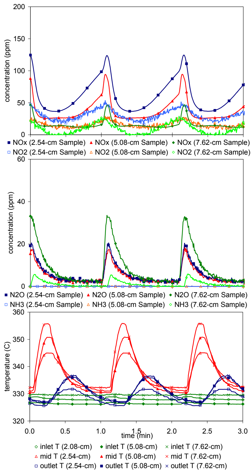
Figure 4.31. Catalyst B's outlet gas concentrations and temperature profiles for 2.54, 5.08 and 7.62-cm-long samples in short-cycle experiments with 1.4% H 2 in rich phase at 325°C
