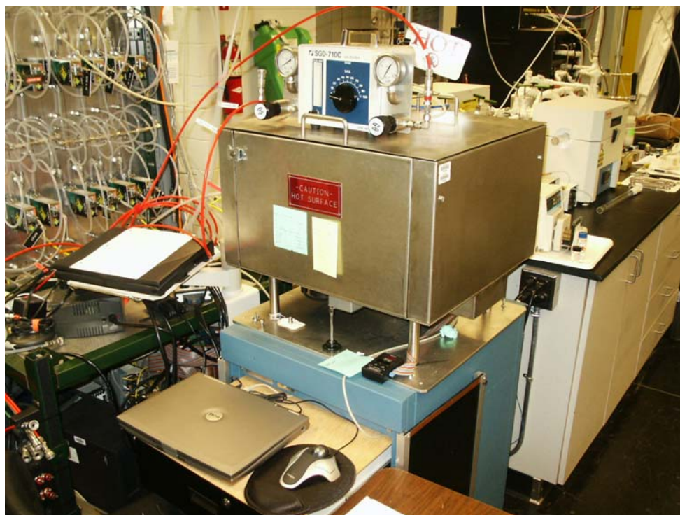
Figure 3.10. Spatially-Resolved Capillary Inlet Mass Spectrometer
