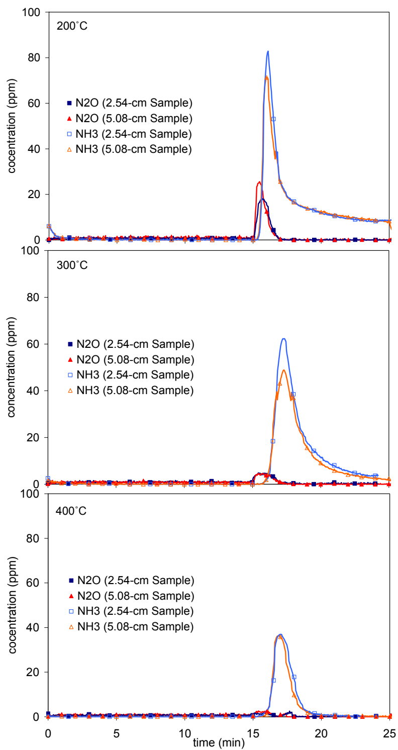
Figure 4.8. Catalyst A's outlet concentrations of \text{N}_2\text{O} and \text{NH}_3 for 2.54 and 5.08-cm-long samples in long-cycle experiments with 0.2% \text{H}_2 in rich phase at 200, 300 and 400°C
