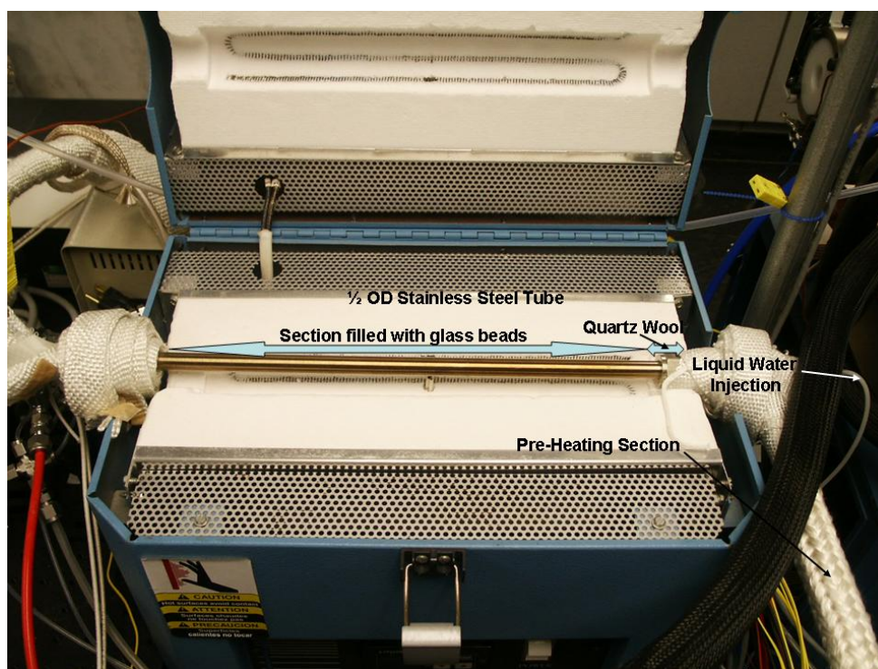
Figure 3.7. Water Evaporator
