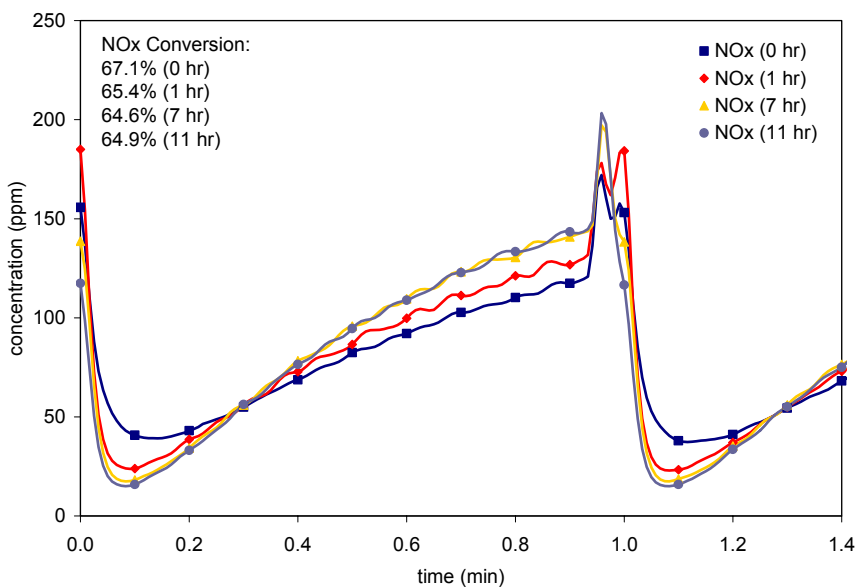
Figure 4.2. Catalyst A's outlet concentrations of NO x for 2.54-cm-long sample in short-cycle baseline experiments with 1.0% H 2 in rich phase at 300°C and 30,000 h -1 space velocity after different "degreening" times
