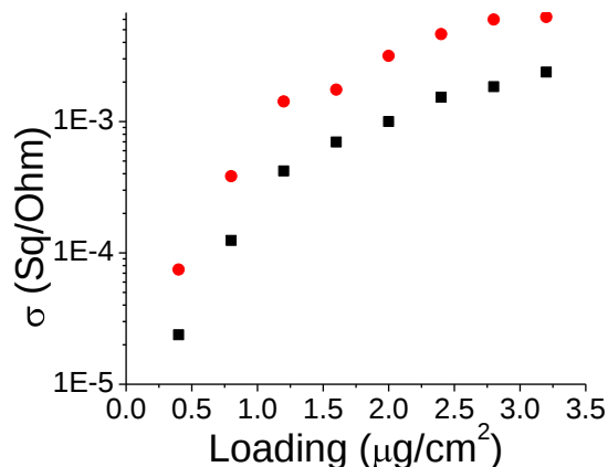
Figure 67 Immersion of a set of SDS-dispersed films in \text{SOCl}_2 causes a factor of three increase in conductivity for each film, independent of nanotube loading.
