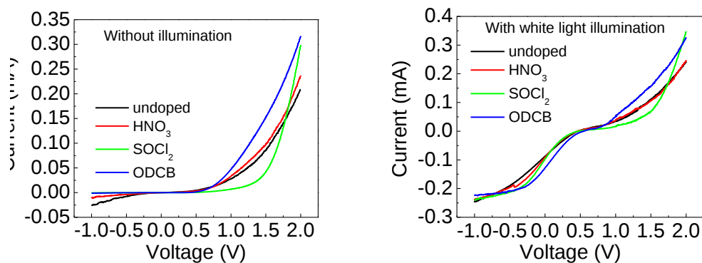
Figure 74 Films with different methods of doping were used in photovoltaic cells. ODCB doped films were the most effective in PV devices, \text{SOCl}_2 doped films were the least effective. PV cell has structure: Glass/SWNT/Pedot/P3HT:PCBM(1:0.8)/Al
