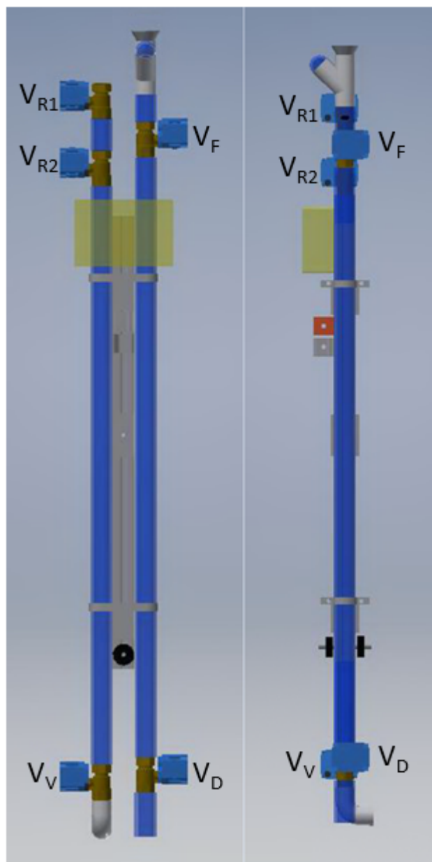
Figure 3.2. A rendering of the cylinder unit. The image on the left is a front view, with the Reference column on the left and the Sample column on the right. The image on the right represents a side view from the Sample cylinder side. V_{R1} and V_{R2} are the Top and Bottom Reservoir valves on the reference cylinder. The Vent valve on the reference cylinder is V_V . The Fill valve and the Drain valve on the sample cylinder are V_F and V_D , respectively.
