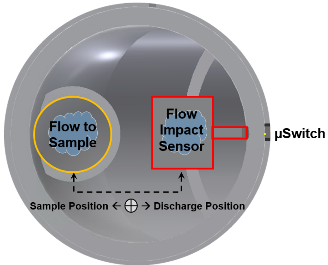
Figure 3.5. A rendering of the water diverter from above, looking directly down into the diverter. The image shows the outer 3" thin-wall PVC diverter body and the 3" 45° PVC elbow below it, the 3/4" PVC pass-through pipe (outlined in yellow) that extends down through the elbow to carry water to the Sample column, the Honeywell microswitch in black to the right side, and the moment arm and flow sensing weight/plate (outlined in red) at the end of the moment arm. Before sampling, the servo holds the inlet tube to the right above the flow sensor in the "Discharge Position". When flow occurs the water pushes down on the weight/plate sufficiently to trigger the microswitch. The microcontroller then causes the servo to rotate, moving the inlet tube left over the 3/4" pass-through pipe ("Sample Position") and directing its flow into the Sample column.
