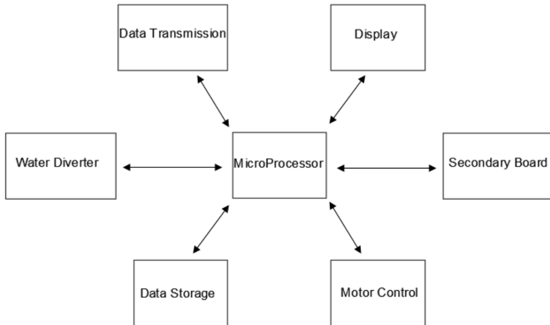
Figure 3.10. The general responsibilities of the main electronics box. The primary Teensy 3.2 in this box communicates with the secondary Teensy (on the Secondary Board) and controls its operations. Additionally, the primary Teensy is responsible for controlling the flipping motor, reading the motor encoder, responding to the diverter flow sensor and operating the water diverter, storing/transmitting the pressure data, and turning on/off an RGB LED.
