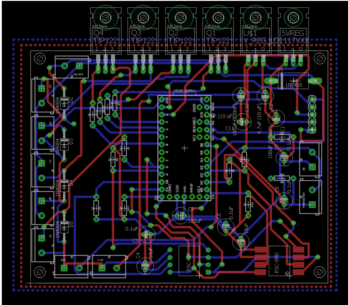
Figure A.6. The above image represents the layout for the secondary printed circuit board.
