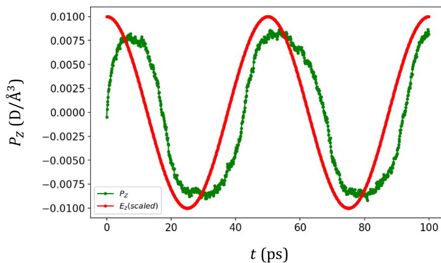
Figure 6.2 The polarization lags behind the electric field in MD simulations using SPC/E model for \nu=20 GHz. The magnitude of electric field is scaled for a better comparison.
