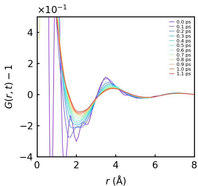
Figure 3.6 Time-sliced G(r, t) of water at 295 K
