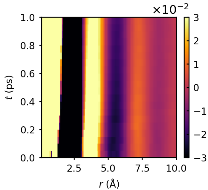
Figure 3.7 Intensity plot of G(r, t) of D_2O at 295 K
