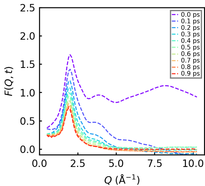
Figure 3.4 Time-sliced F(Q, t) at 295 K for D2O
