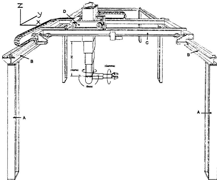
Figure 3.1: Gantry System
