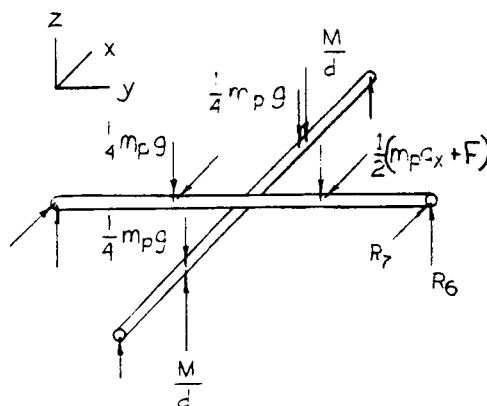
Control Tube Forces
