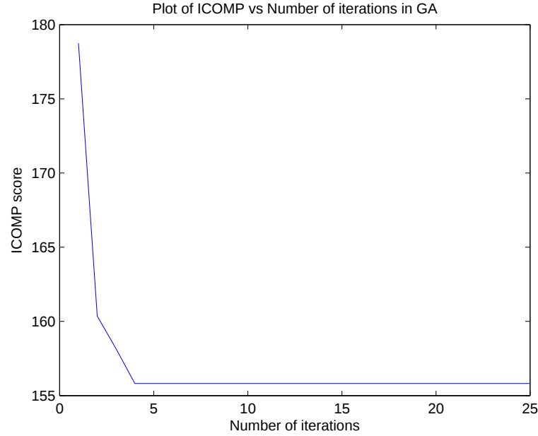
Figure 6.21: HCS Data (MVLR): Plot of ICOMP vs Number of iterations in GA
