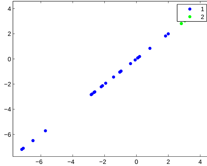
Figure 6.35: KCS Group 2 Data: Scatter Plot Matrix
