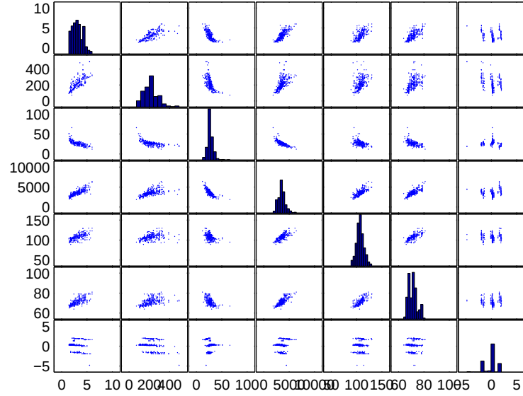
Figure 6.7: Beta-Carotene: Plot matrix of the best predictors in the model RetPlasma
