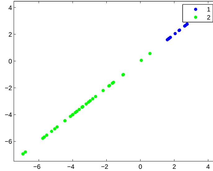
Figure 6.33: KCS Group 1 Data: Scatter Plot Matrix
