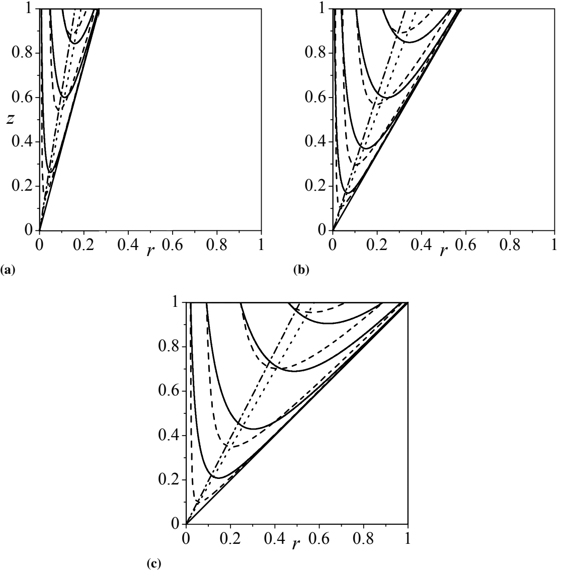
Figure 5.3: Flow streamlines for \sigma_c = 1 and cone half-angles of \alpha = (a) 15^\circ , (b) 30^\circ , and (c) 45^\circ . Here the present model (—) is compared to the Beltramanian model (---).
