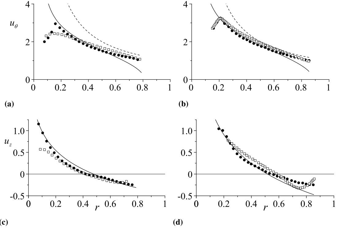
Figure 3.6: The theoretical Beltramanian model (—) and free vortex ( 1/r ) model (---) plotted against experimental (●) and numerical (□) results by (a) and (c) Hsieh and Rajamani (1988) at an axial location of z = 167.67 and (b) and (d) Monredon et al. (1992) at an axial location of z = 181.67 . The tangential velocity, u_\theta , scales with (a) U = 7.98 m/s and (b) U = 6.26 m/s while the axial velocity, u_z , scales with (c) \sigma_c = 0.2 and (e) \sigma_c = 0.305 .
