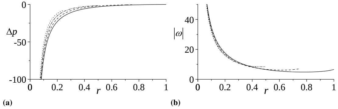
Figure 3.7: The (a) pressure difference and (b) vorticity magnitude for \sigma_c = 1 and divergence angle \alpha = 45^\circ at four axial locations of z/L = 1 (—), 0.75 (---), 0.5 (- · -), and 0.25 (····).
