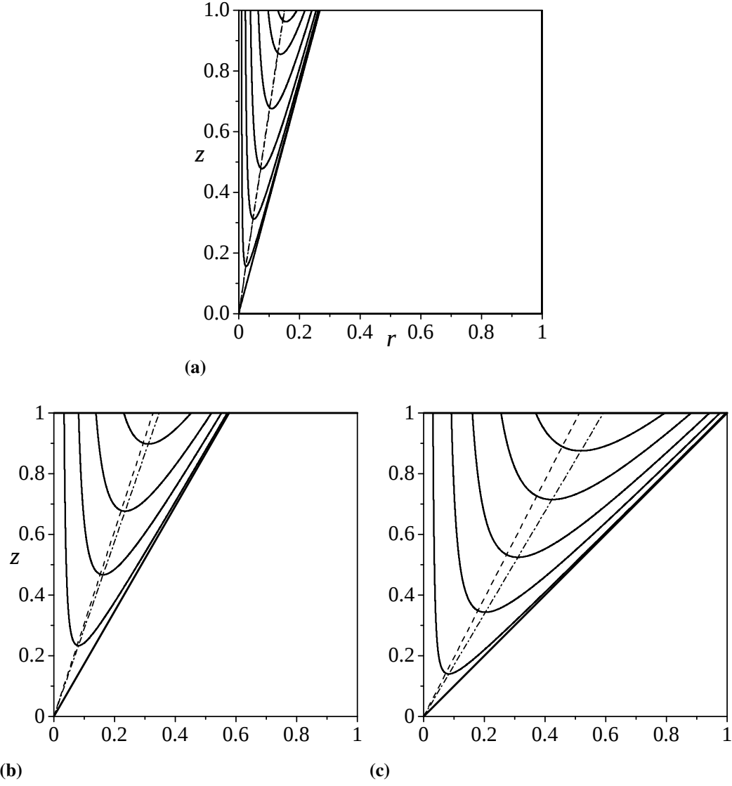
Figure 3.1: Streamlines of the Beltramian model for \sigma_c = 1 with the spherical radial velocity mantle, \beta_R , as (---) and the axial velocity mantle, \beta_z , as (-\cdot-) . Plot (a) displays the divergence half-angle of \alpha = 15^\circ with values of \beta_R = 9.09^\circ , \beta_z = 9.21^\circ and at the axial location of z/L = 1 , b_r = 0.597 and b_z = 0.605 . Plot (b) displays the divergence half-angle of \alpha = 30^\circ with values of \beta_R = 18.16^\circ , \beta_z = 19.14^\circ and at the axial location of z/L = 1 , b_r = 0.568 and b_z = 0.601 . Plot (c) displays the divergence half-angle of \alpha = 45^\circ with values of \beta_R = 27.18^\circ , \beta_z = 30.62^\circ and at the axial location of z/L = 1 , b_r = 0.514 and b_z = 0.592 .
