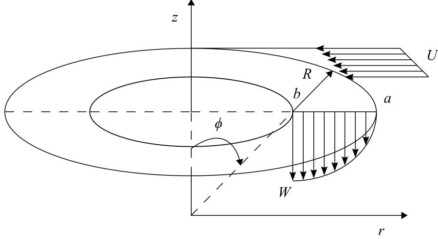
Figure 4.1: The generalized Beltramian analysis inlet axial velocity profile as a half-parabola shape.
