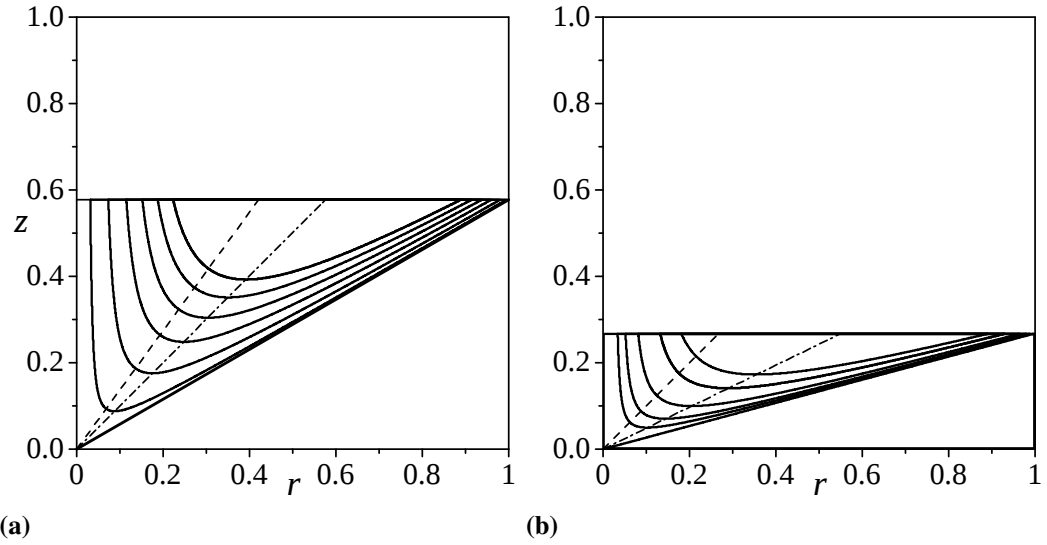
Figure 3.2: Streamlines of the Beltramanian model for \sigma_c = 1 with the spherical radial velocity mantle, \beta_R , as (- - -) and the axial velocity mantle, \beta_z , as (- \cdot -) . Plot (a) displays the divergence half-angle of \alpha = 60^\circ with values of \beta_R = 36.12^\circ , \beta_z = 44.95^\circ and at the axial location of z/L = 1 , b_r = 0.421 and b_z = 0.576 . Plot (b) displays the divergence half-angle of \alpha = 75^\circ with values of \beta_R = 44.93^\circ , \beta_z = 66.99^\circ and at the axial location of z/L = 1 , b_r = 0.267 and b_z = 0.549 .
