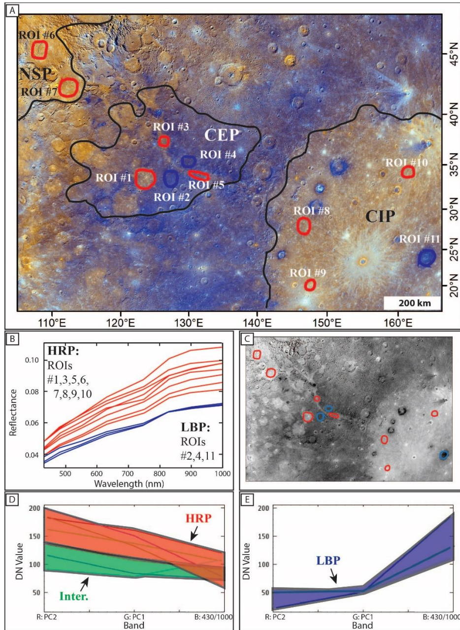
Figure 30. A: Color mosaic (R: 430 nm, G: 750 nm, B: 1000 nm) with overlaid ROIs within the CEP, CIP, and NSP. These ROIs cover HRP (red) and LBP (blue) units in each of the CEP, CIP, and NSP, which are marked by black outlines. B: Spectra of the ROIs. The LBP spectra are tightly clustered while the HRP spectra exhibit a greater spread in spectral slopes. C: The extracted PC2 from the 8-band enhanced color mosaic, highlighting further differences between HRP and LBP units. The location of ROIs from A are represented by open circles, with red representing the HRP and blue representing the LBP. D: Enhanced color mosaic RGB combination (R: PC2, G: PC1, B: 430 nm/1000 nm) used for comparison from the enhanced color mosaic between HRP units in the CIP and NSP (red band) versus the red plains units in the CEP (green band), which I characterize as an "Intermediate" composition. E: Enhanced color mosaic RGB combination (R: PC2, G: PC1, B: 430 nm/1000 nm), where blue plains units cluster together (blue band), with clearly different slopes than the HRP and Intermediate units. The locations for these extracted data correspond to the ROIs in A. The PC2 DN values for the HRP are range from ~150-200, while the PC2 DN values for the LBP range from ~5-50.
