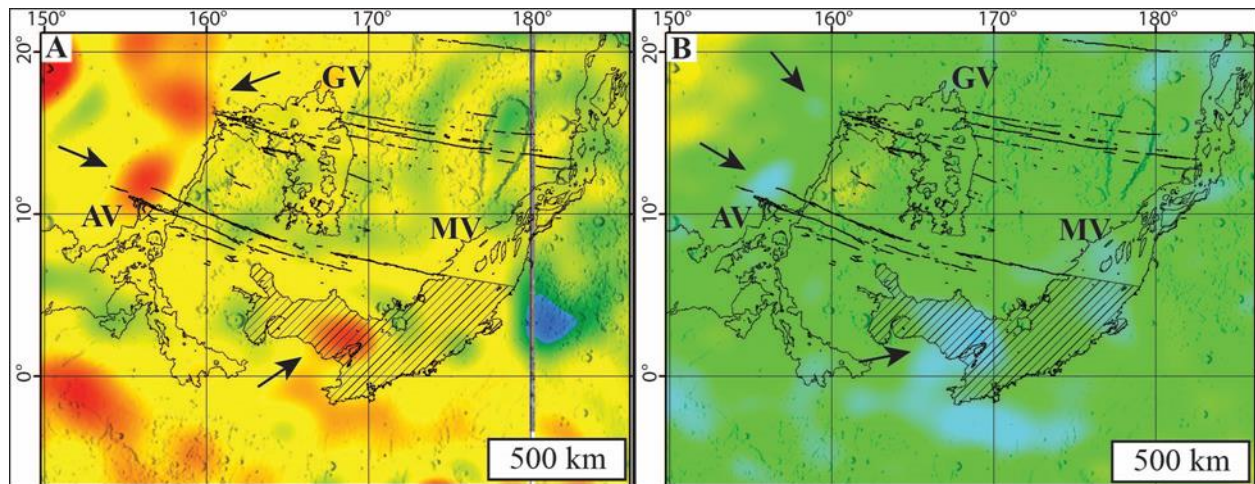
Figure 9. The mapped extent of the three main channels and their associated lavas in the study area, Athabasca (AV), Grjóta (GV), and Marte Valles (MV). A: Free-air gravity anomaly map (data from Genova et al, 2016), where warm colors denote positive anomalies and cool colors denote negative anomalies. Three anomalies (black arrows) are found in proximity to the source regions for the channelized lavas. The lack of topographic variability (Fig. 1) indicates that the regions of high density associated with the positive gravity anomalies are due to subsurface variation. B: Crustal thickness map (data from Genova et al., 2016), where warm colors denote thicker regions and cool colors denote thinner regions. Relatively low crustal thicknesses (black arrows) are found in proximity to the source regions for the channelized lavas. An apparent spatial correlation exists between the positive gravity anomalies and regions of relatively thin crust.
