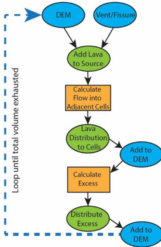
Figure 17. Simplified schematic of model architecture. Lava is erupted from the vent or fissure and added at the source. The flow into adjacent cells is calculated and then distributed to these cells. Once the initial distribution is completed, if any volume from that iteration remains, the amount of excess lava is calculated and then distributed to the next adjacent cells. Once the full volume of each iteration has been distributed, the model loops back to the beginning, to distribute the next pulse of lava along the flow pathway. (Blue ovals denote model inputs, green ovals denote a process, and orange rectangles denote a calculation).
