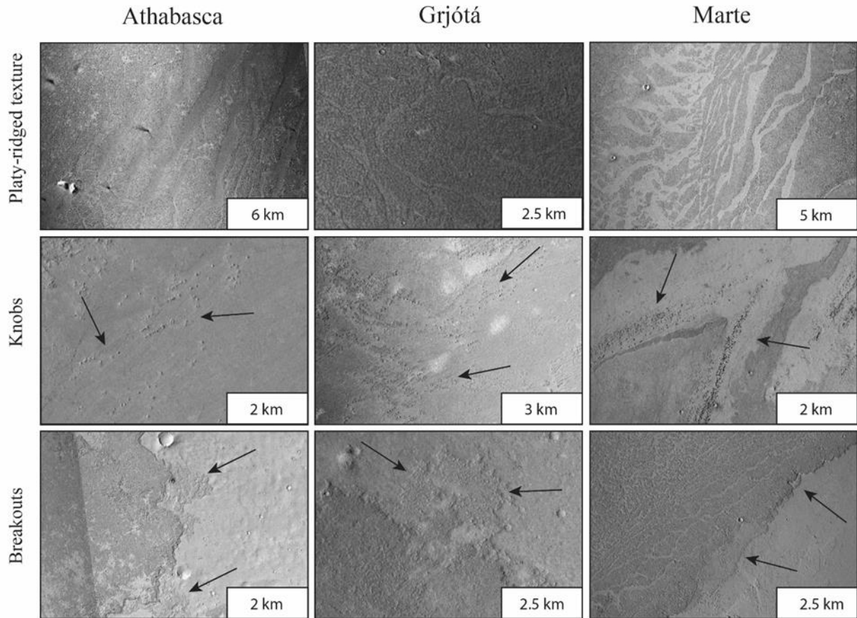
Figure 2. Typical surface textures identified in the three channelized lavas, including platy-ridges, knobs, and breakouts. The interplate regions of the platy-ridged texture are dark in Athabasca Valles, unlike in Grjótá and Marte Valles. These plates and ridges are smaller and extremely muted in Grjótá Valles. Each flow contains populations of knobs (black arrows), often found in curvilinear concentrations. The margins of the flows may also exhibit limited breakouts (black arrows) from beneath their coherent crusts. These breakouts are generally small, with the exception of those found along the eastern margin of Marte Vallis.
