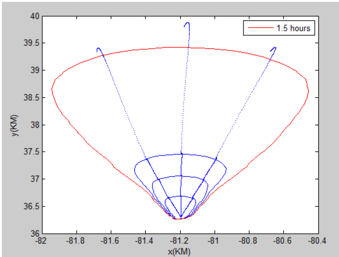
Figure 4.9 Sensors reach the predicted locations of the new boundary, but they send measurements less than the boundary threshold
