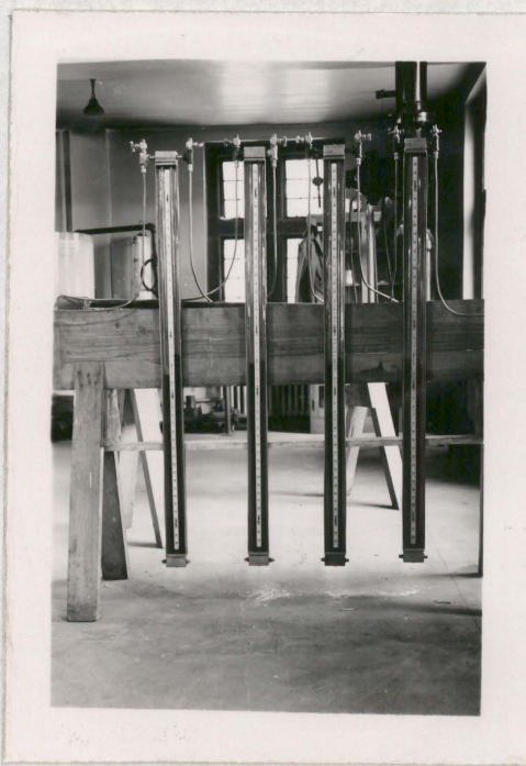
Plate II b - Set of Four Manometers Used in the Tests.
