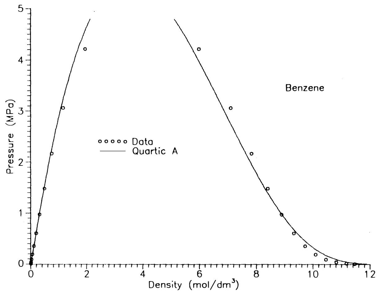
Figure 4.13: Saturated VLE calculations for Benzene
