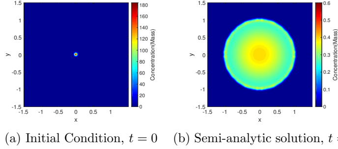
Figure 1.1: Initial condition and semi-analytic solution for the line source benchmark.
