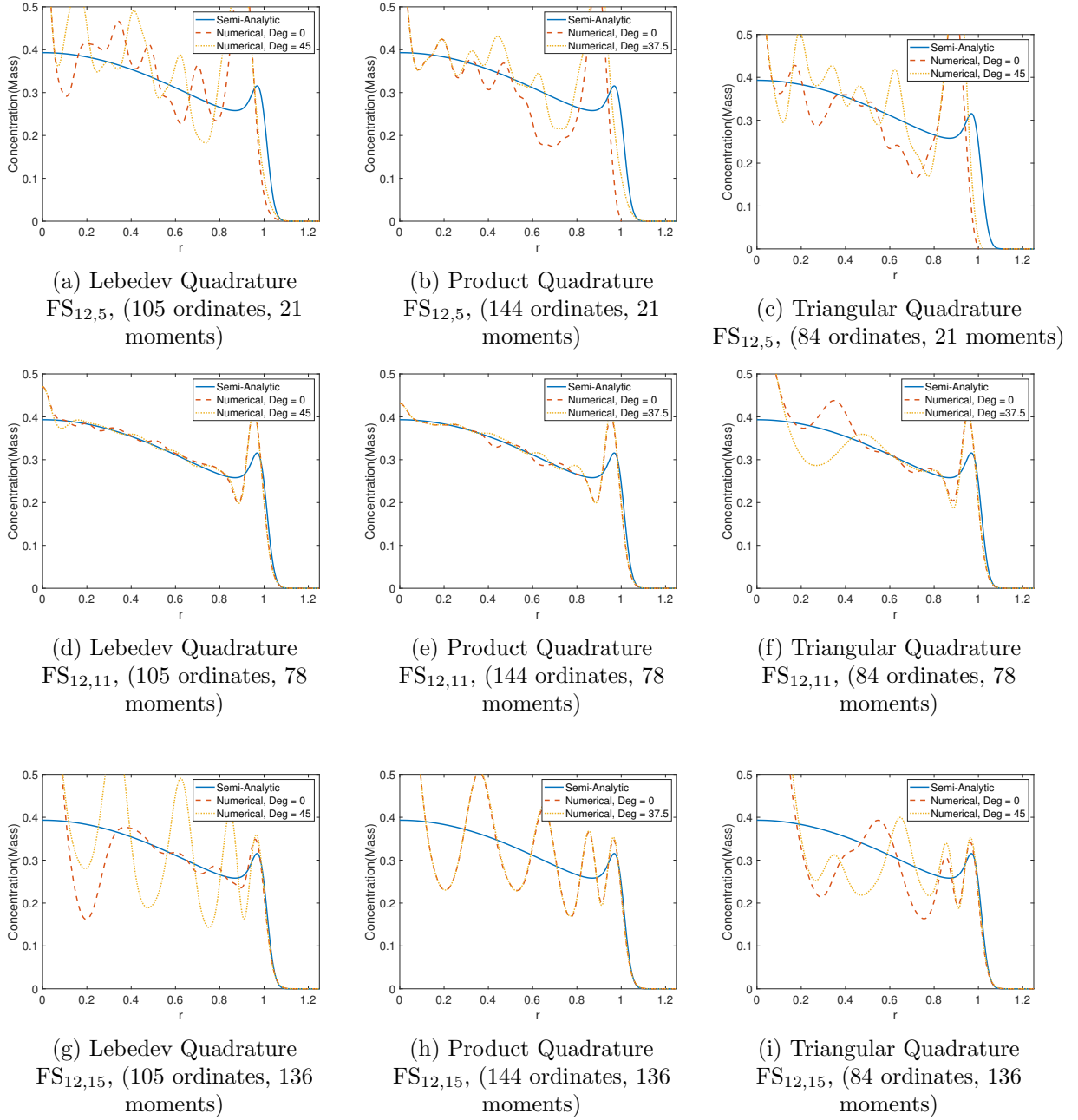
Figure 3.3: Radial line-outs of the solutions in Figure 3.2.
