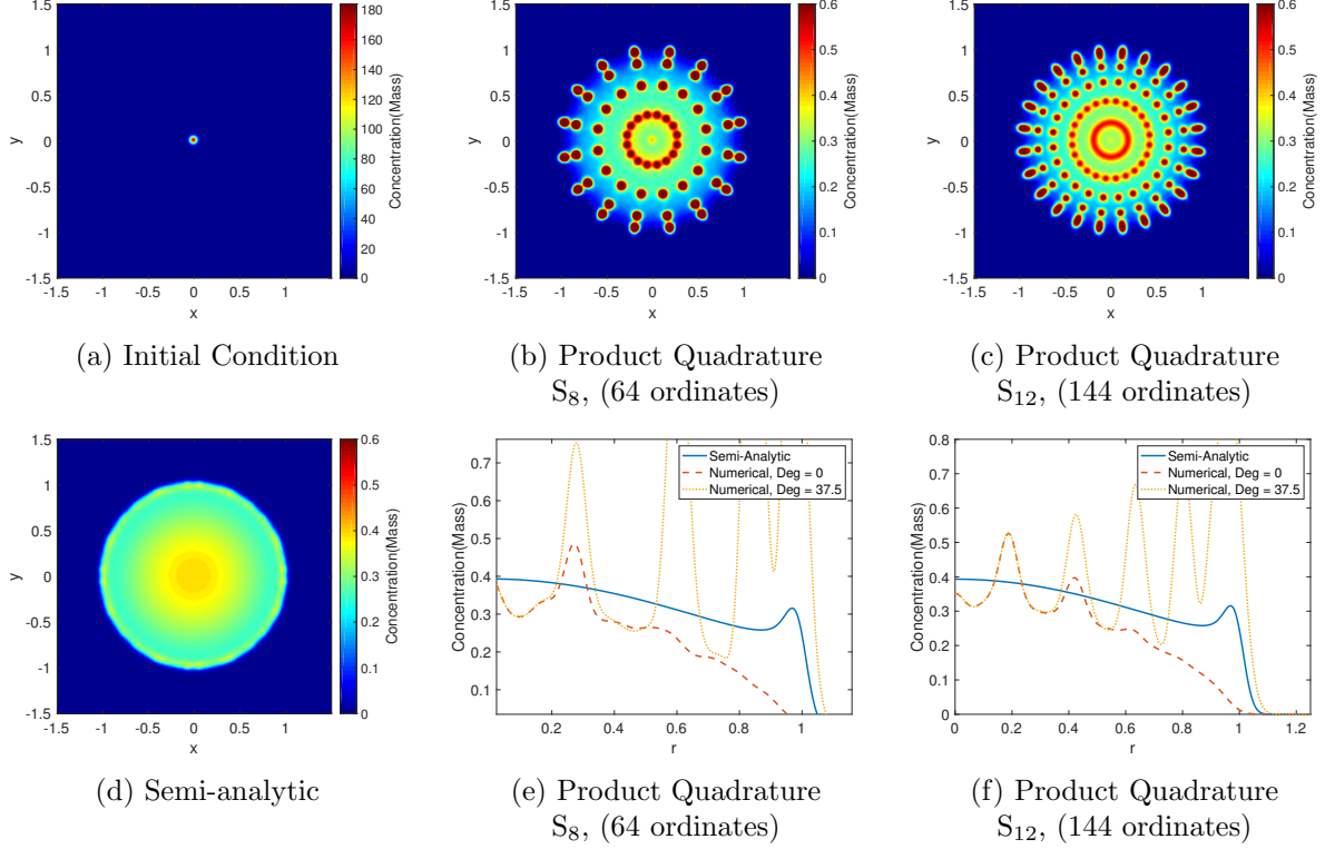
Figure 3.1: Line-source solutions with line-outs.
