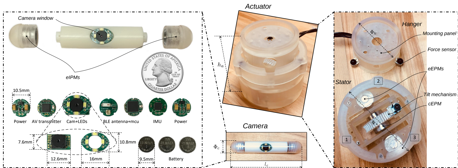
Figure 2.14: Prototype II.
