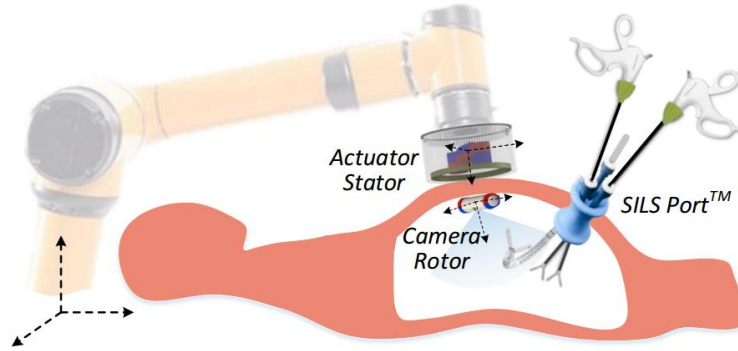
Figure 5.1: Concept of camera pose estimation with the sCAM system. An AUBO-i5™.
