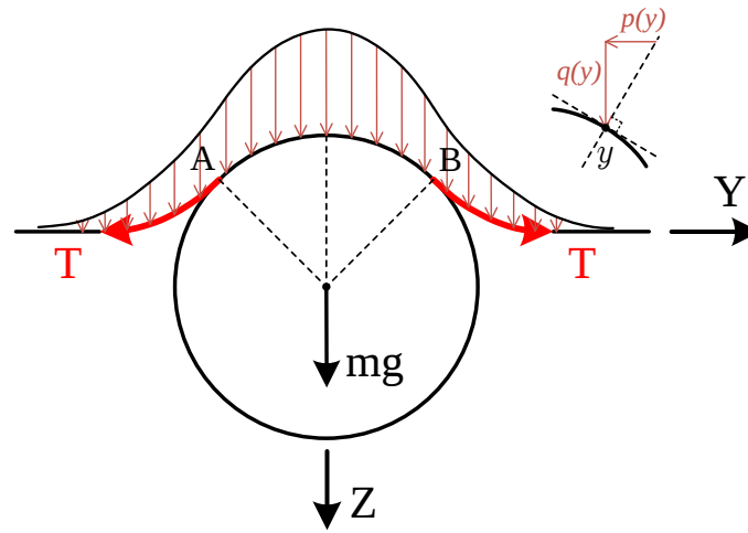
Figure 4.5: Latitudinal sectional view of stress distribution.
