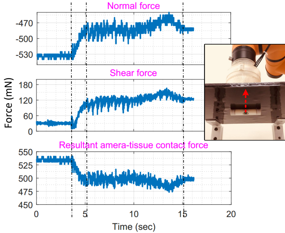
Figure 4.21: Translation experiment.
