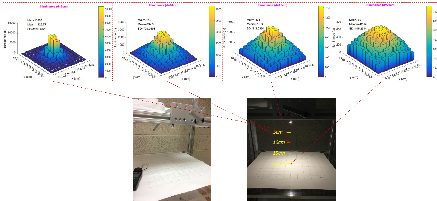
Figure 2.9: Illuminance test.
