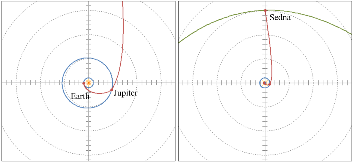
Figure 2 Earth – JGA – Sedna trajectory showing (left), the Jupiter swingby from Earth and (right), the approach to Sedna.
