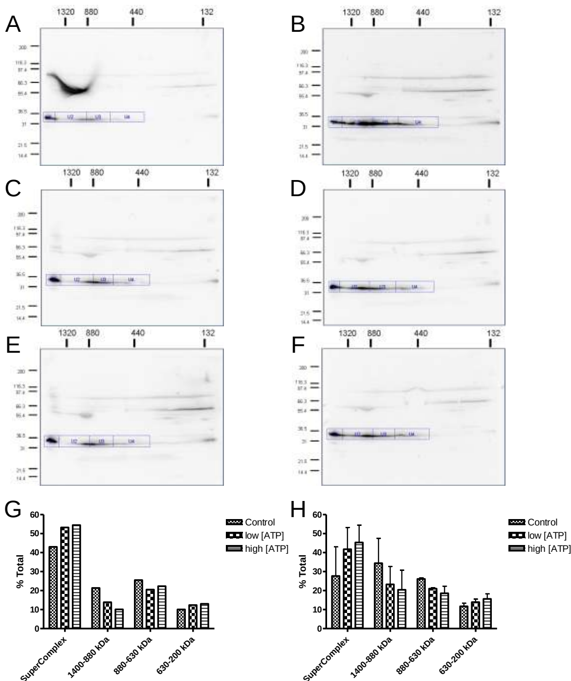
Figure 3-23 Two-dimensional BN/SDS-PAGE analysis of Toc34 distribution with prSSU incubation in binding and active import conditions.
