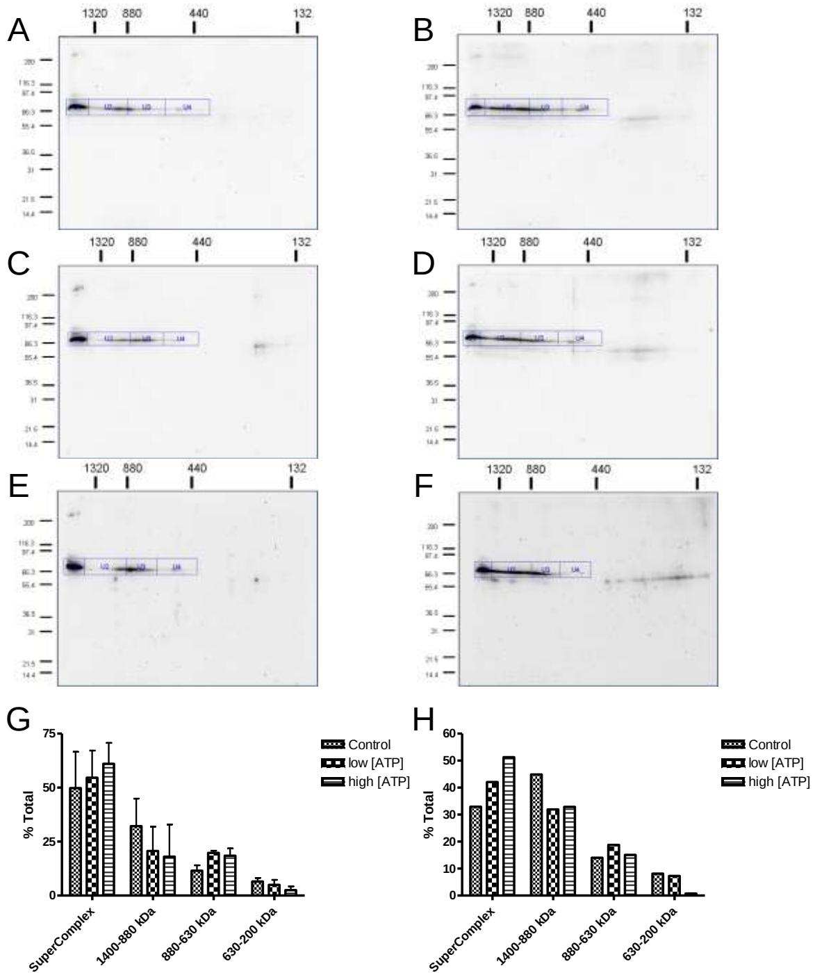
Figure 3-22 Two-dimensional BN/SDS-PAGE analysis of Toc75 distribution with prSSU incubation in binding and active import conditions.
