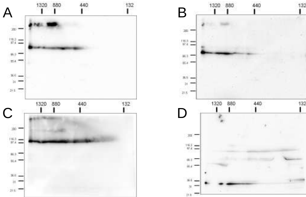
Figure S-1 Two-dimensional BN/SDS-PAGE analysis of Tic110 distribution. Blots are control treatment of chloroplasts from first POTRA experiment. A represents the \alpha -Toc159 western blot. B represents the PVDF from A stripped and reprobed with \alpha -Toc75 antiserum. C represents the PVDF from A & B stripped and reprobed with \alpha -Tic110 antiserum. D represents a separate 2d gel and western blot with \alpha -Toc34 antiserum.
