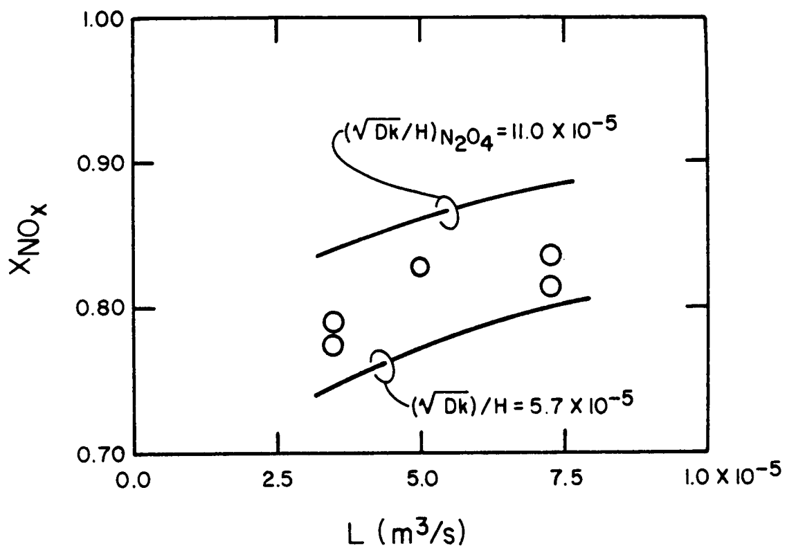
Fig. 18. Experimental nitrogen oxide conversions at varying liquid rates and model predictions over the range of (\sqrt{Dk}/H)_{N_2O_4} values from runs 10-4, 10-5, 10-6, 10-7, and 10-8. Other parameters were G \cong 3.2 \times 10^{-4} std m^3 s^{-1} , H = 0.90 m, Y_{NO_x, in} \cong 0.05 , and P_T = 1.1 atm.
