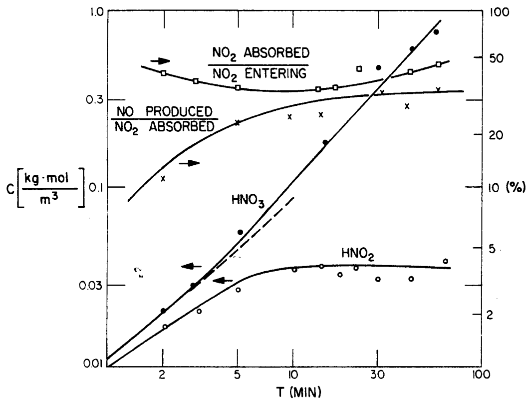
Figure 2. Results of semi-batch \text{NO}_2 absorption studies.
