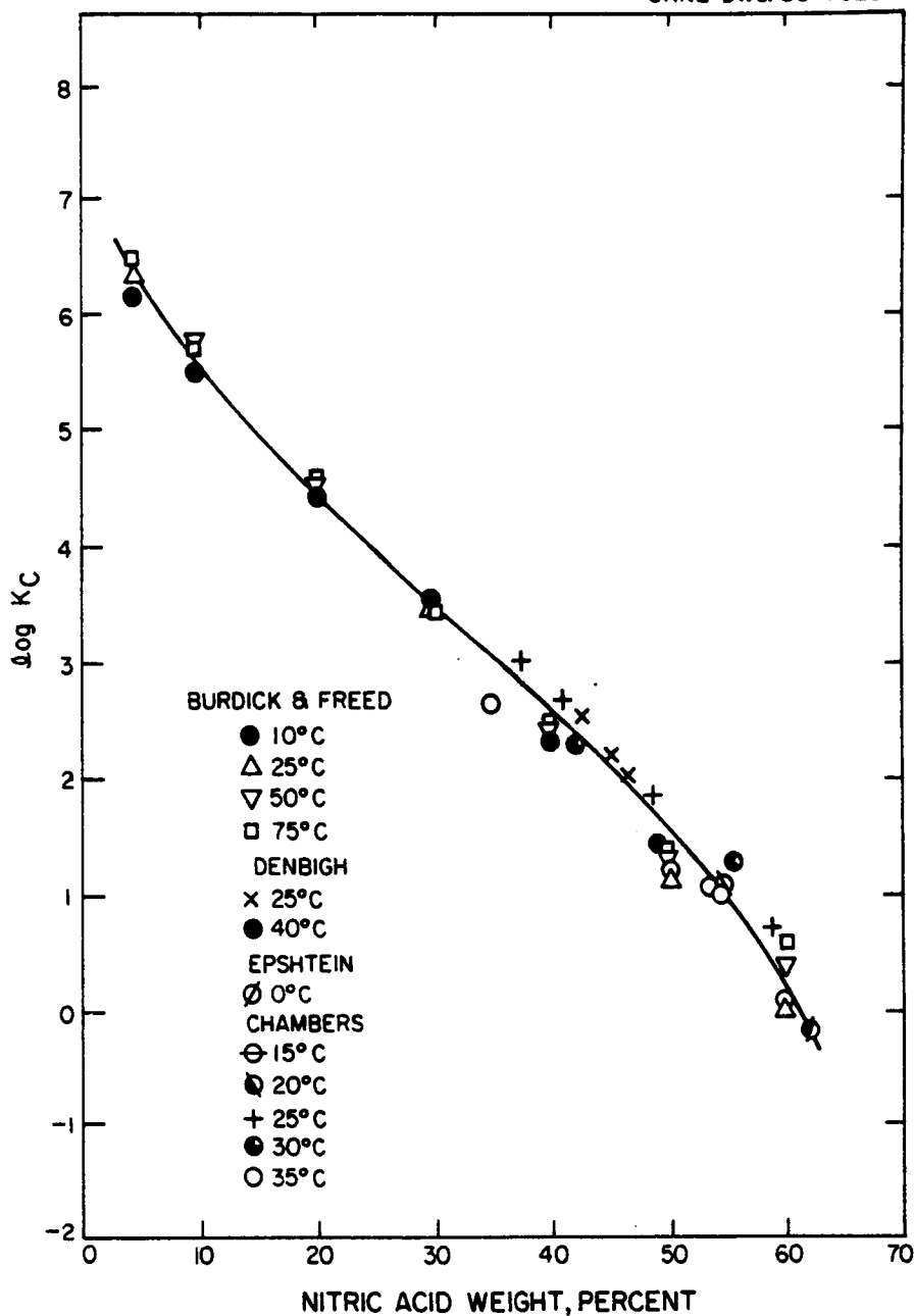
Figure 1. Equilibrium between phases for Reaction (29).
