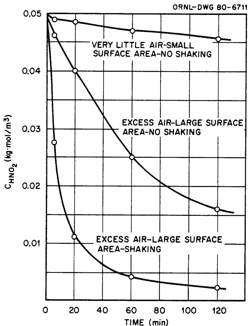
Figure 3. The effect of shaking and surface on the decomposition of 0.05 kg·mol m -3 nitrous acid.
