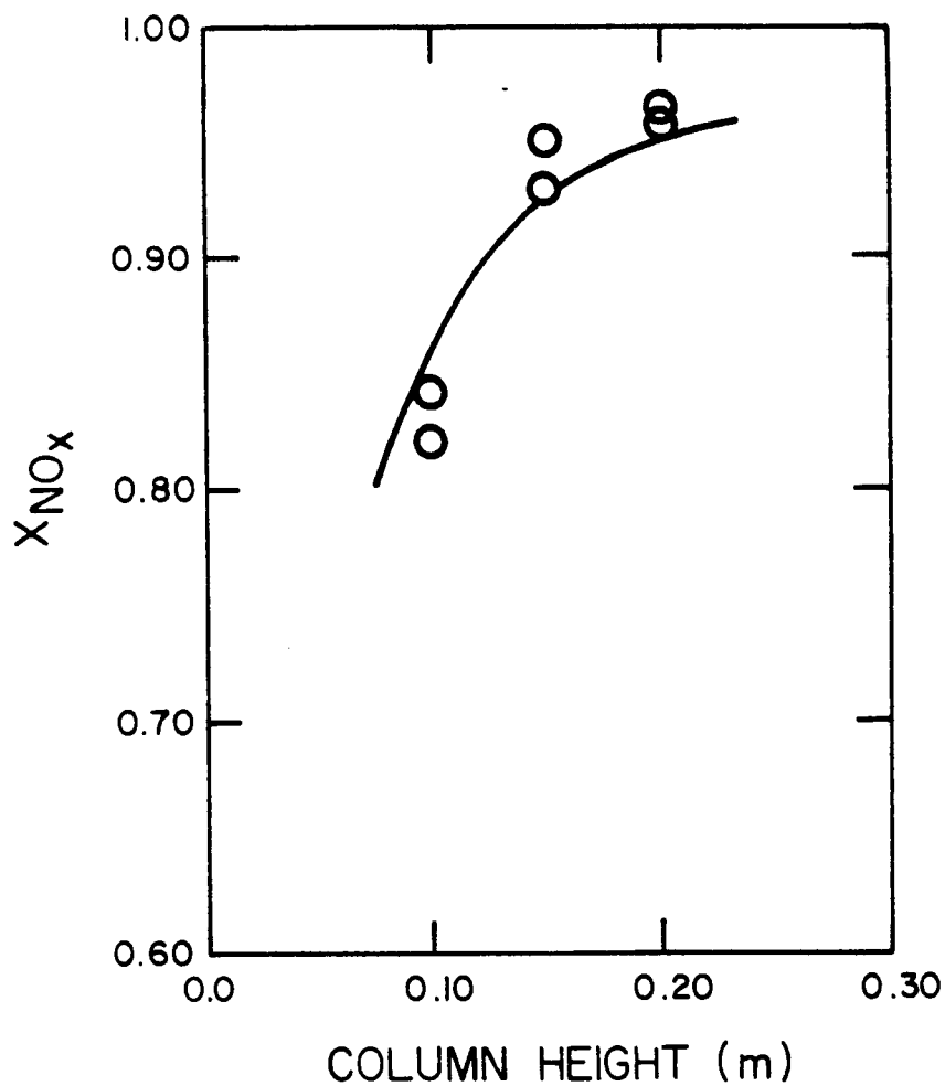
Fig. 19. Experimental and model predicted conversion at varying column heights from runs PTR-19, PTR-20, PTR-21, PTR-22, PTR-23, and PTR-24. Other parameters were G = 3.3 \times 10^{-4} std m^3 s^{-1} , L = 4.5 \times 10^{-5} m^3 s^{-1} , Y_{NO_x, in} = 0.10 , and P_T = 1.10 atm.
