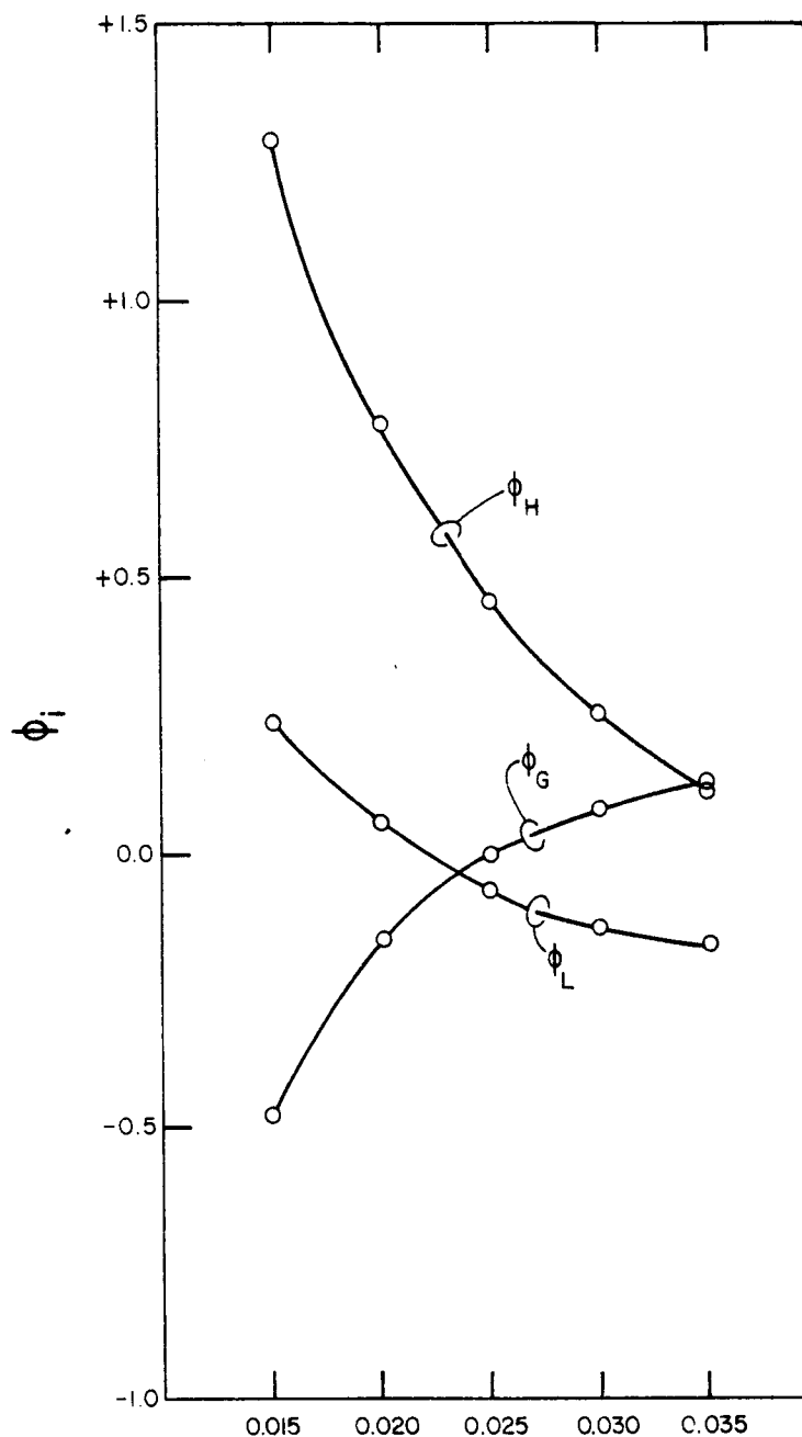
Figure D.5. The relative main effects of the manipulation of L, G, and H on X_{\text{HNO}_2} at varying C_{\text{HNO}_2, \text{in}} .
