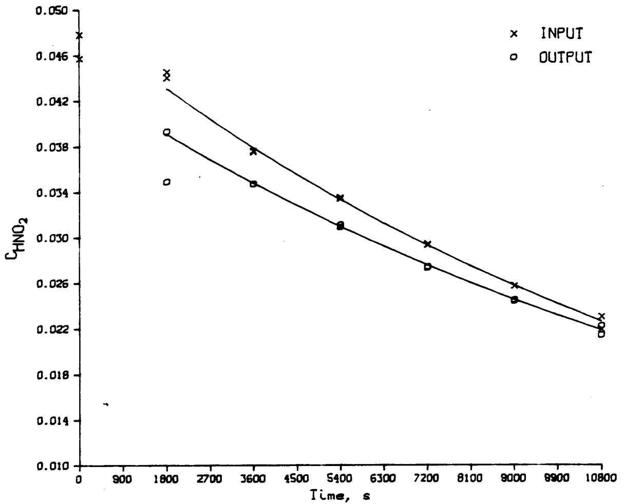
Figure D.1. Column feed and effluent nitrous acid concentrations vs time for experiment A.
