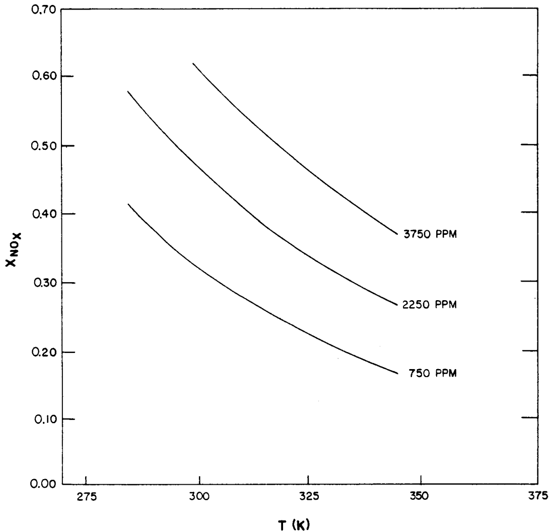
Figure 10. The conversion of NO_x in a packed tower as a function of temperature at gas and liquid rates of 0.156 \text{ m}^3 \text{ s}^{-1} and 9.46 \times 10^{-4} \text{ m}^3 \text{ s}^{-1} , respectively, obtained by Bowman, Kulczak, and Shulman.
