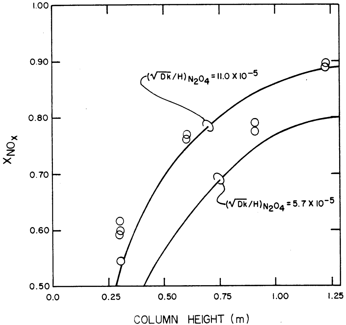
Figure 16. Experimental nitrogen oxide conversions at varying column heights and model predictions over the range of (\sqrt{Dk}/H)_{N_2O_4} values from runs 10-5, 10-6, 10-11, 10-12, 10-15, 10-16, 10-17, 10-18, 10-21, and 10-22. Other parameters were G \cong 3.2 \times 10^{-4} std m^3 s^{-1} , L = 3.5 \times 10^{-5} m^3 s^{-1} , Y_{NO_x, in} = 0.05 , and P_T = 1.1 atm.
