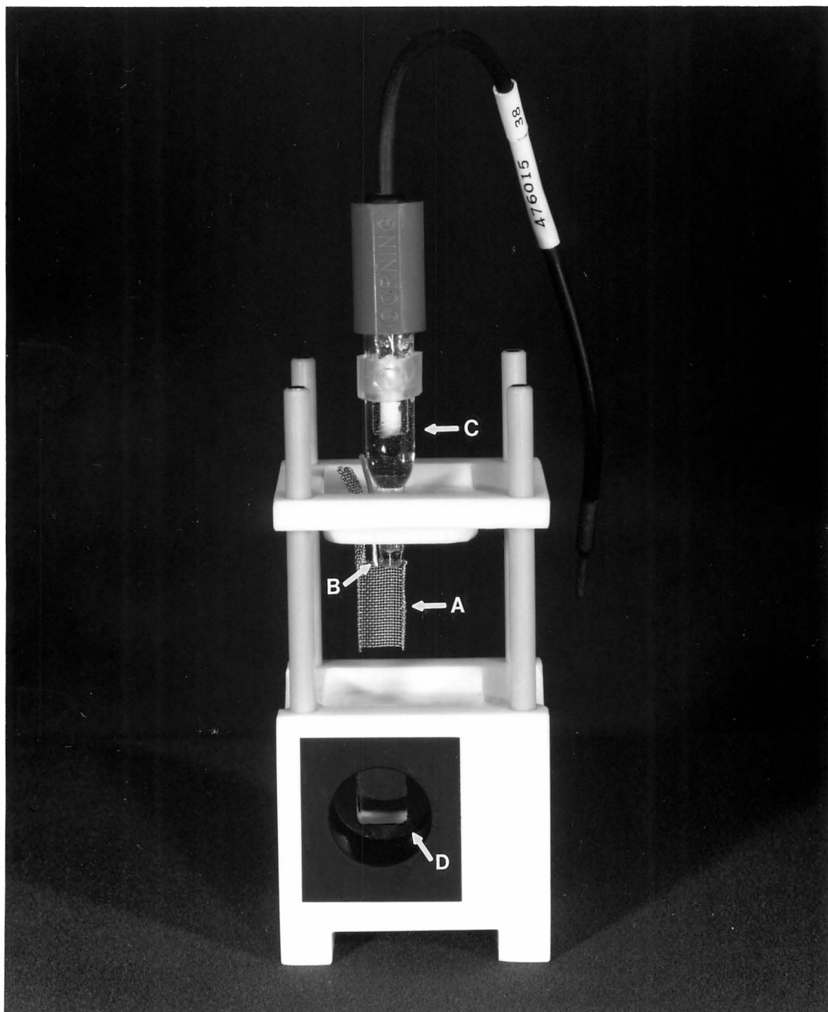
Figure 6. Teflon cell holder with lid in "up" position. Platinum screen working electrode (A), platinum counter electrode (B), SCE reference electrode (C), and optical path through quartz cell (D).
