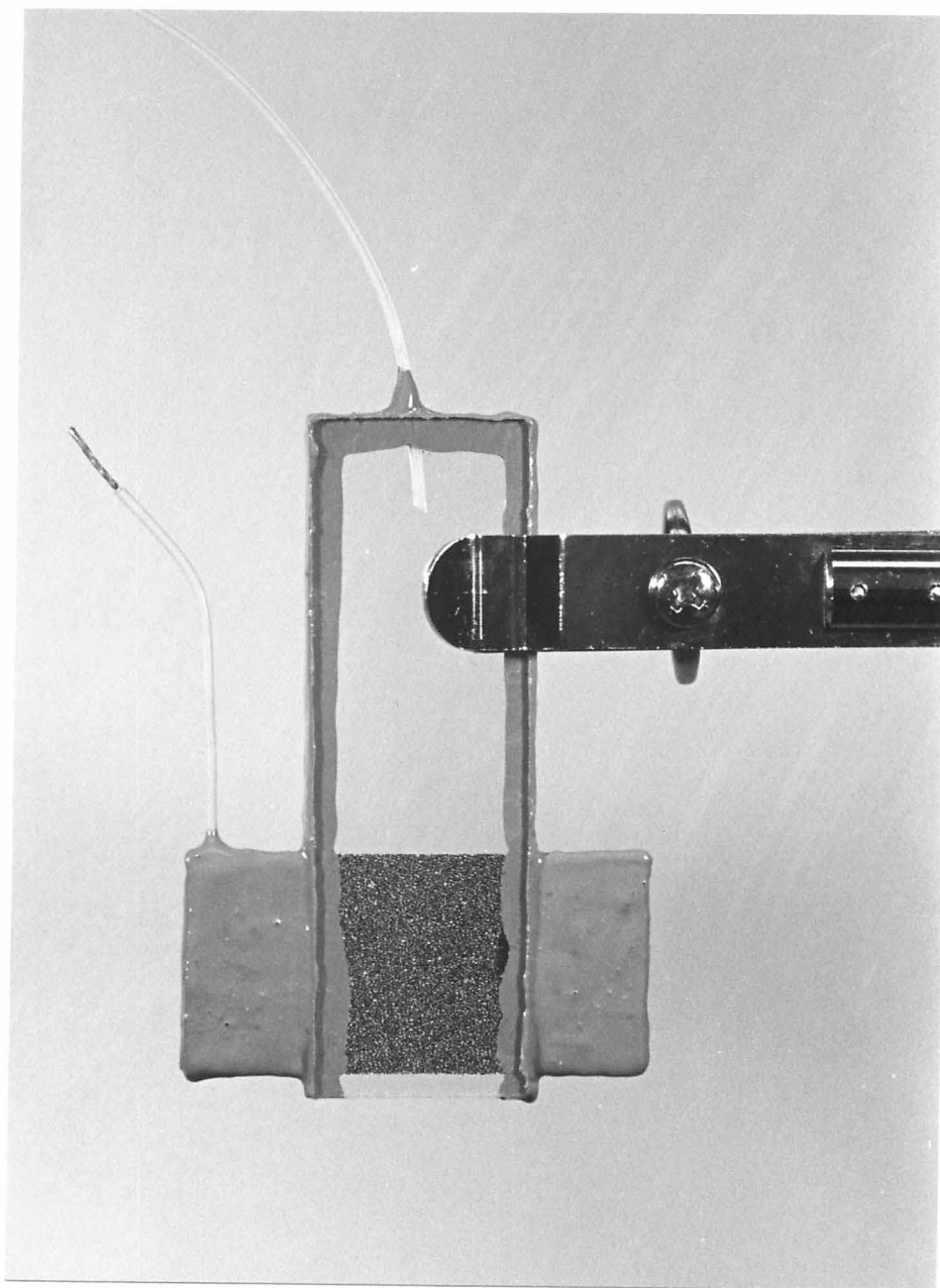
Figure 5. A reticulated vitreous carbon optically transparent electrode (RVC-OTE).
