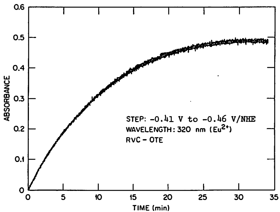
Figure 13. Absorbance vs time curve for the potential-step electrolysis of Eu(III) in an RVC-OTE. RVC: 100 ppi, 1 mm path length, [Eu(III)] = 1.0 \times 10^{-2} M.
