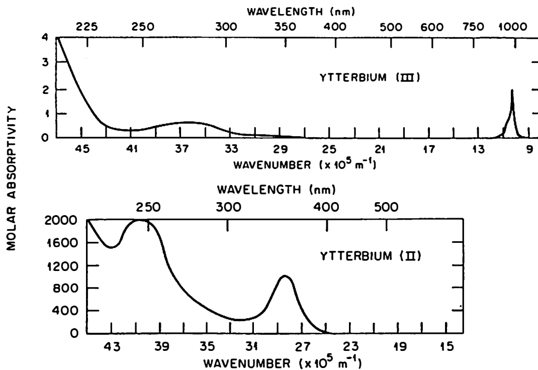
Figure 11. Solution absorption spectra of Yb(III) and Yb(II) in 1 M HClO 4 .
