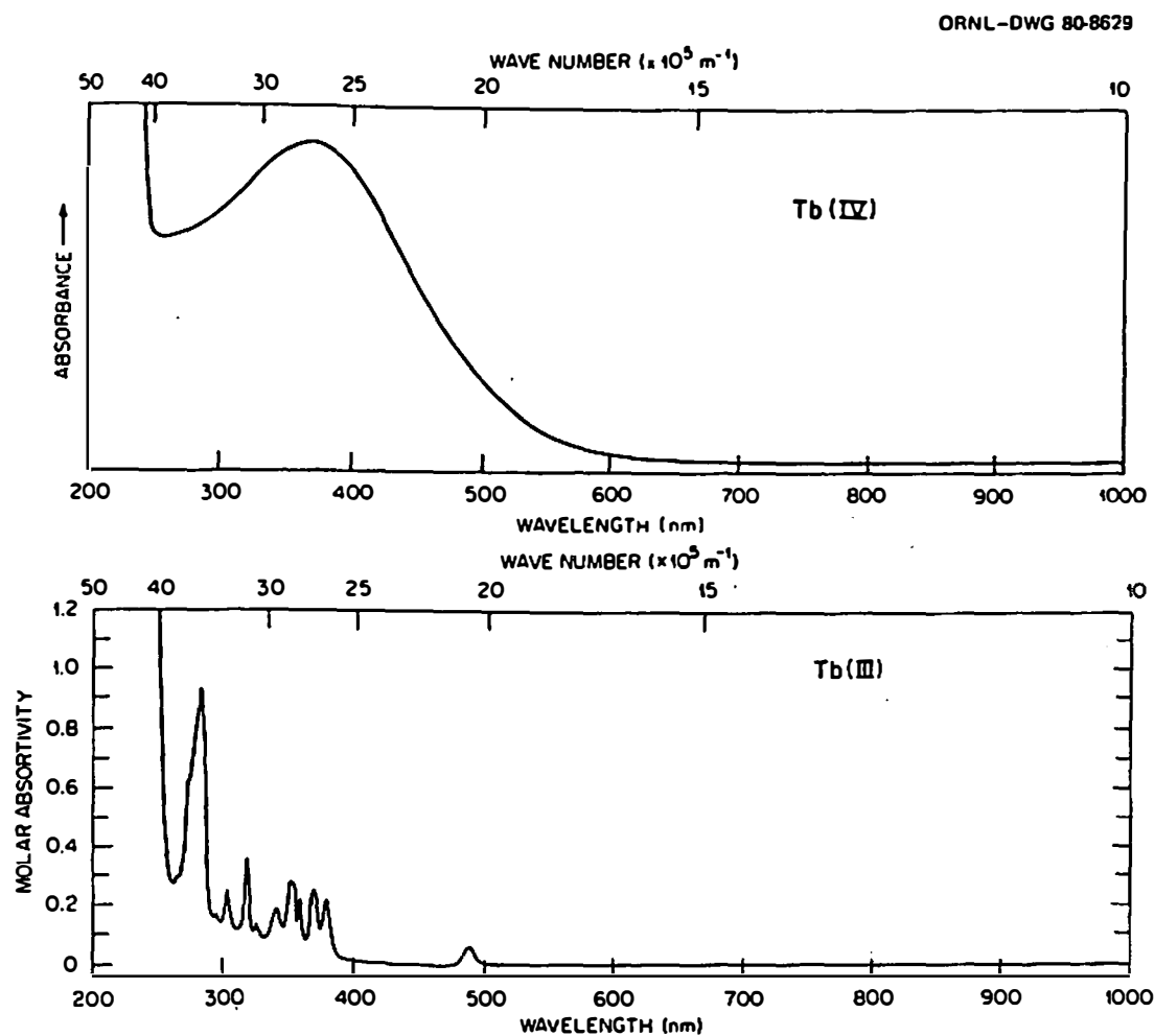
Figure 22. Solution absorption spectra of Tb(III) and Tb(IV) in 5.5 M \text{K}_2\text{CO}_3 .
