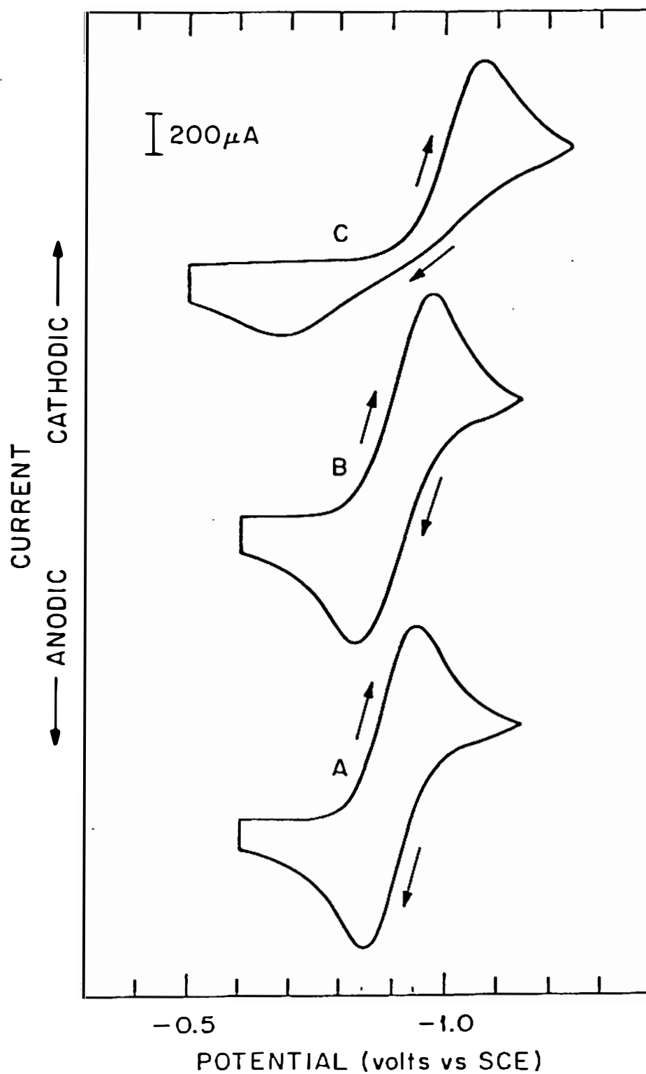
Figure 29. Cyclic voltammograms of U(IV) in 1 M KCl at an HMDE. pH 0 (A), pH 1 (B), and pH 2 (C). [\text{U(IV)}] = 1.0 \times 10^{-1} \text{ M} , sweep rate: 200 mV/s.
