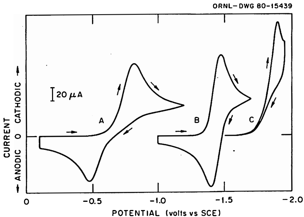
Figure 8. Cyclic voltammograms of M(III) species of Eu (A), Yb (B), and Sm (C) in 1 \text{ M} KCl. pH 6, HMDE, sweep rate: 200 \text{ mV/s} , [\text{M(III)}] = 1.0 \times 10^{-2} \text{ M} .
