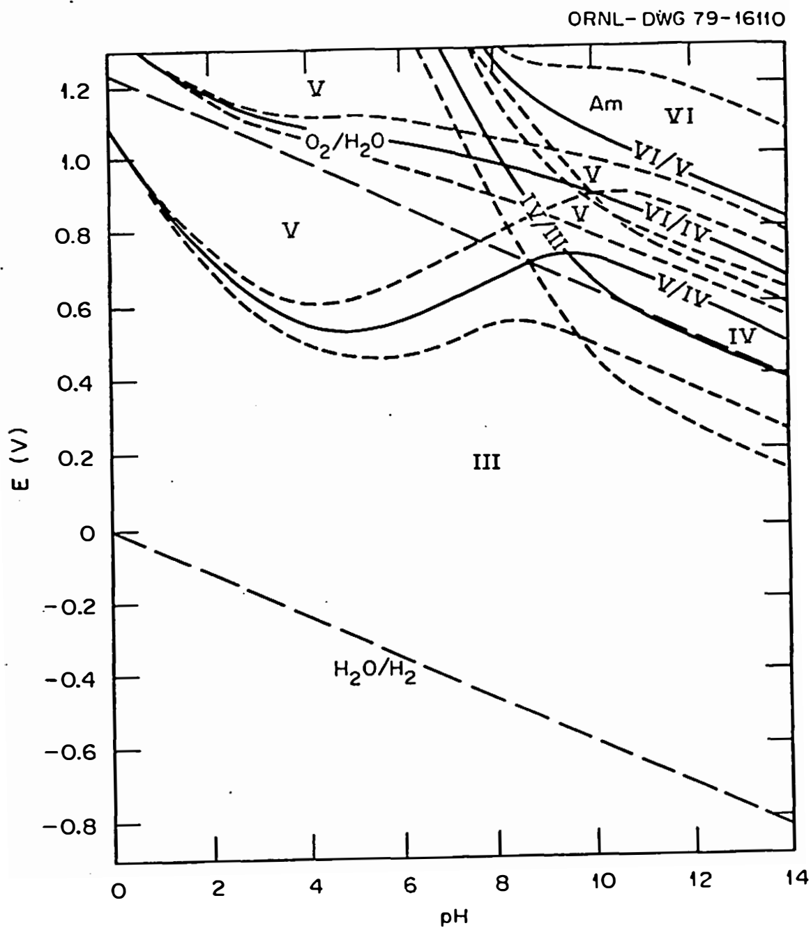
Figure 50. Potential vs pH diagram for the predicted oxidation state species of Am in aqueous solution. Potential in V vs NHE.
