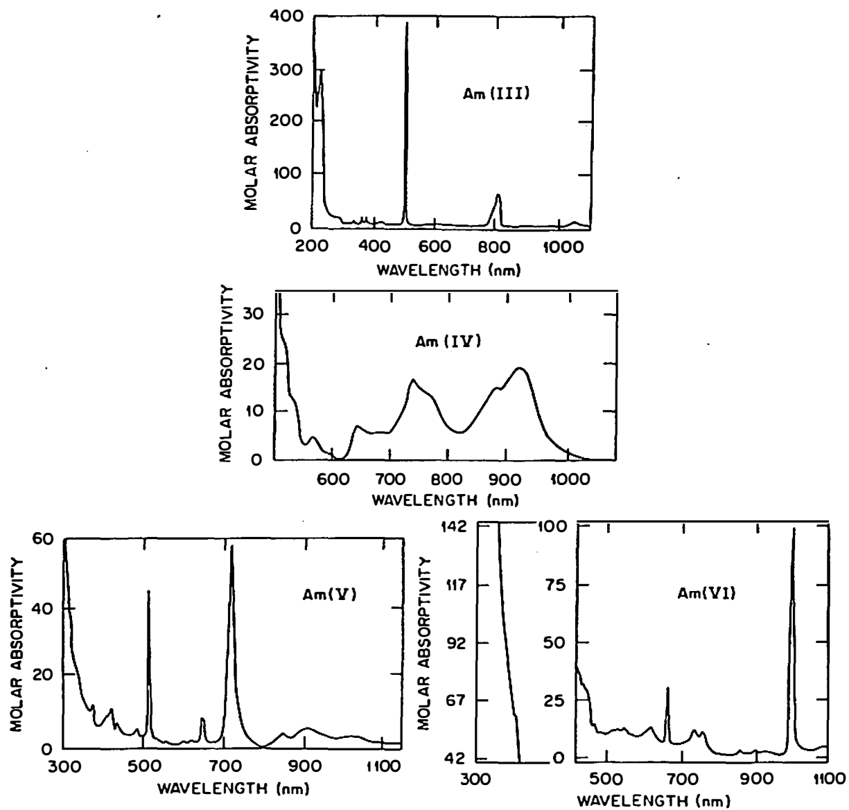
Figure 40. Solution absorption spectra of Am(III, IV, V, and VI). Am(IV) in 10 M H 3 PO 4 , others in 1 M HClO 4 .
