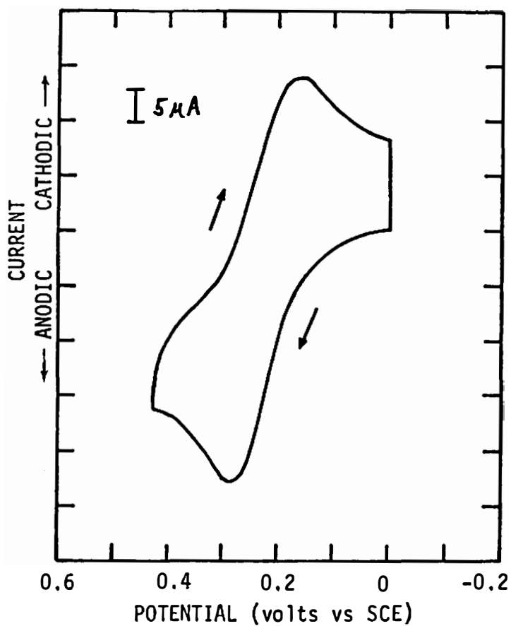
Figure 36. Cyclic voltammogram of Np(VI) in 2 M Na 2 CO 3 at pH 13. Pt electrode, sweep rate: 50 mV/s, [Np(VI)] = 10 -3 M .
