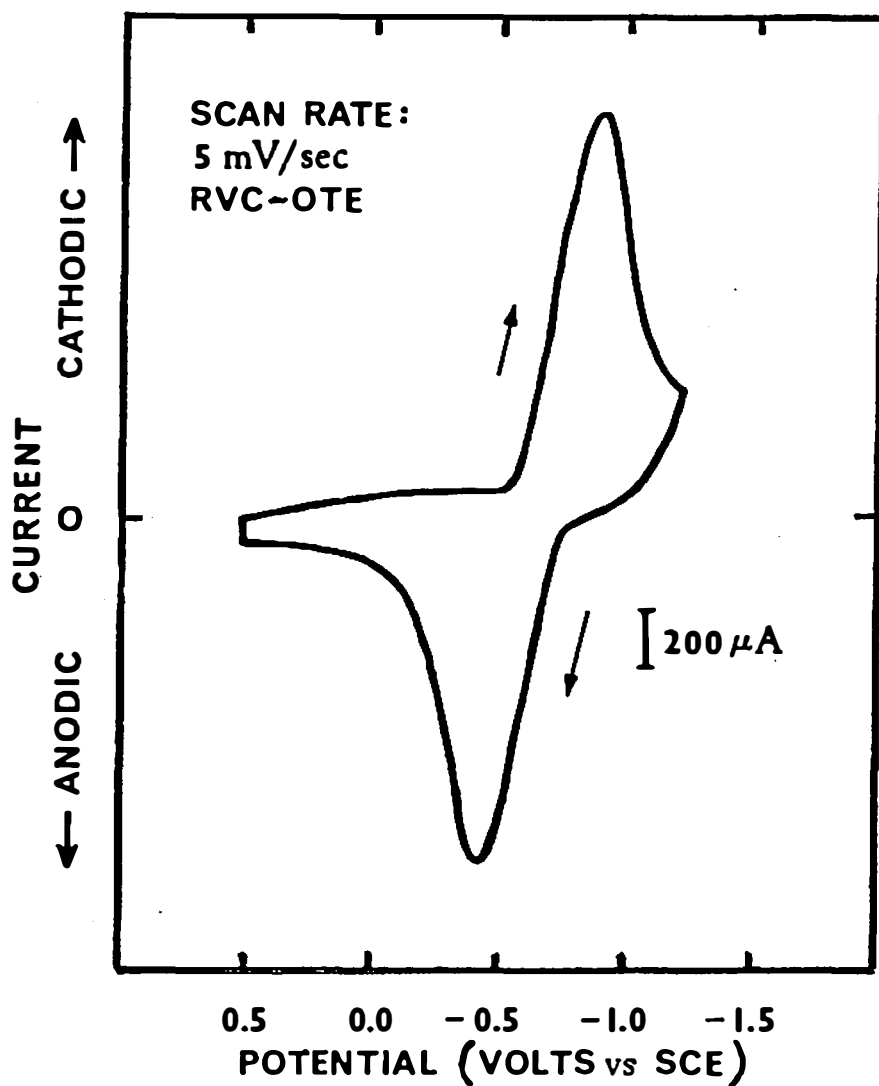
Figure 9. Cyclic voltammogram of Eu(III) in 1 M KCl in an RVC-OTE. pH 6, RVC-OTE: 100 ppi, 0.62 mm path length, [Eu(III)] = 1.0 x 10 -4 M .
