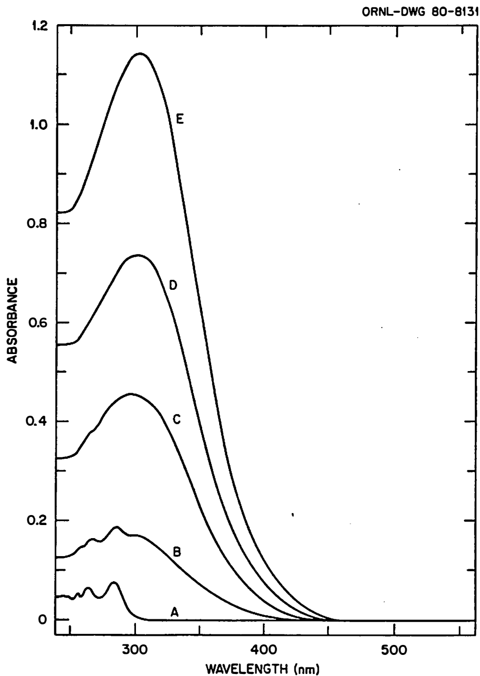
Figure 19. Solution absorption spectra of Ce(IV) and Ce(III) at various values of applied potential in 5.5 M \text{K}_2\text{CO}_3 . -0.26 V (A), 0.002 V (B), 0.04 V (C), 0.06 V (D), 0.44 V (E). RVC-OTE: 100 ppi, 1 mm path length, [\text{Ce(III)}] = 1.0 \times 10^{-3} M.
