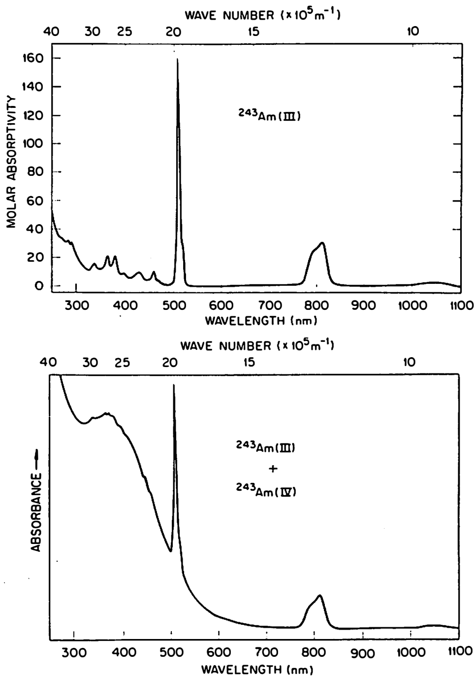
Figure 41. Solution absorption spectra of Am(III) and Am(III) plus Am(IV) in 5.5 M \text{K}_2\text{CO}_3 .
