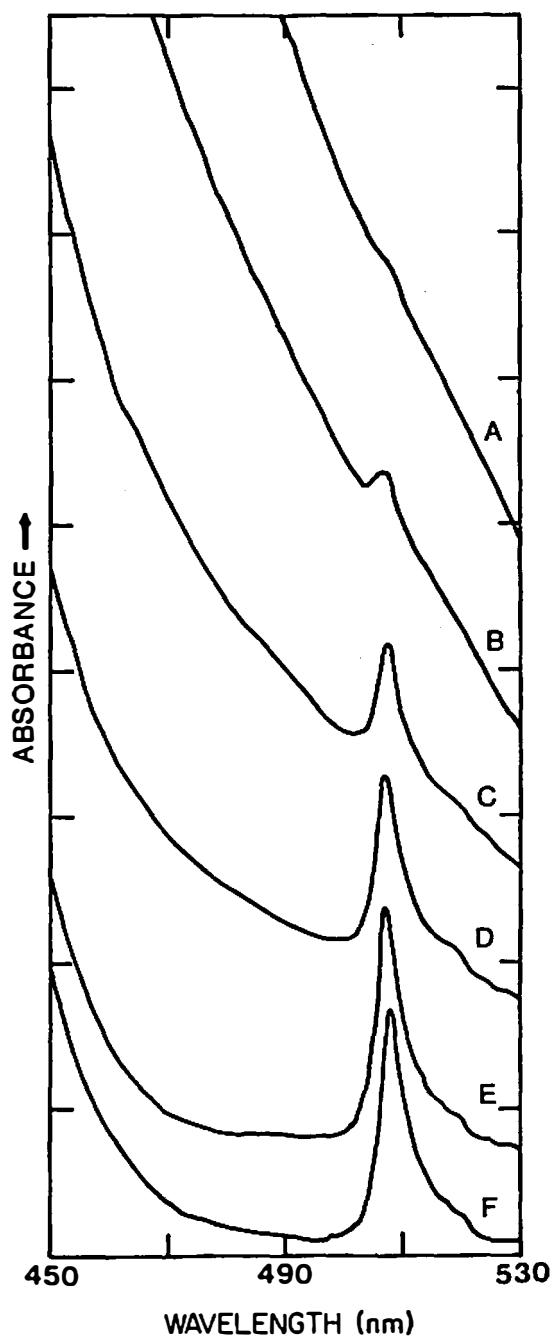
Figure 45. Solution absorption spectra of Am(IV) and Am(III) as a function of titrant added during a spectrophotometric titration of Am(IV) with ferrocyanide solution. 0 \mu\text{L} (A), 50 \mu\text{L} (B), 100 \mu\text{L} (C), 150 \mu\text{L} (D), 175 \mu\text{L} (E), and 200 \mu\text{L} (F).
