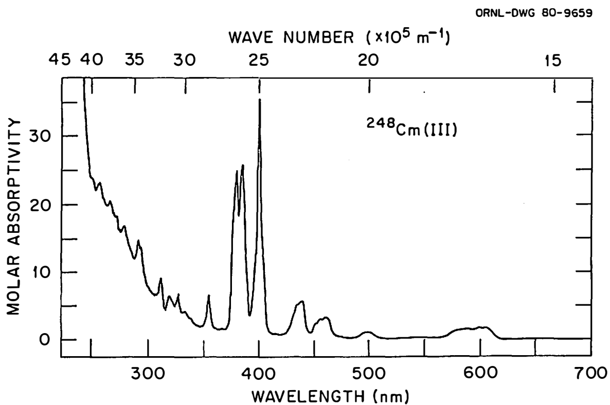
Figure 49. Solution absorption spectrum of Cm(III) in 5.5 M \text{K}_2\text{CO}_3 .
