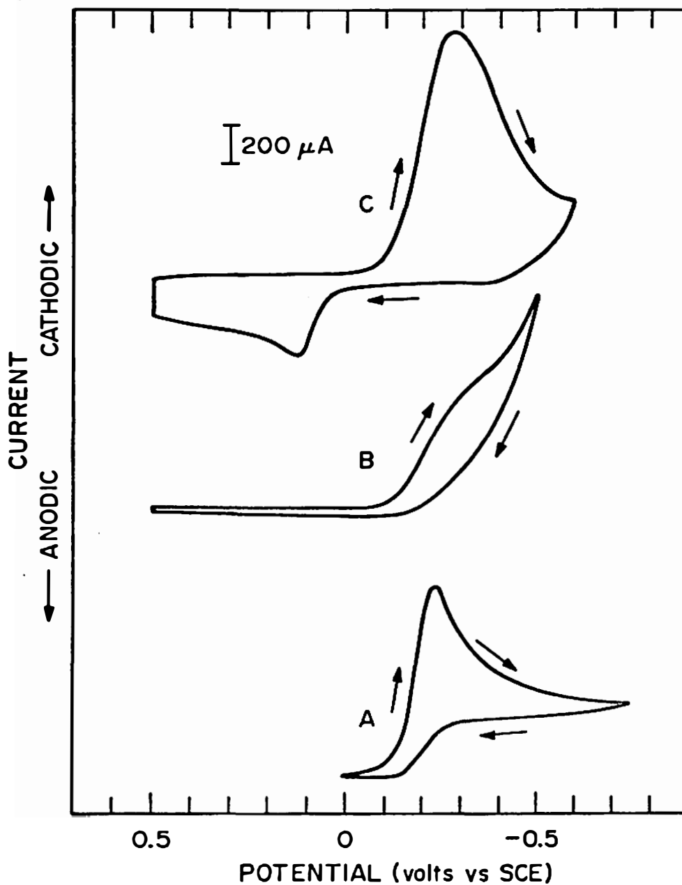
Figure 25. Cyclic voltammograms of U(VI) in 1 M KCl. pH 0 at HMDE (A), pH 0 at Pt (B), and pH 3 at Pt (C). Scan rate: 200 mV/s, [U(VI)] = 1.0 \times 10^{-2} M .
