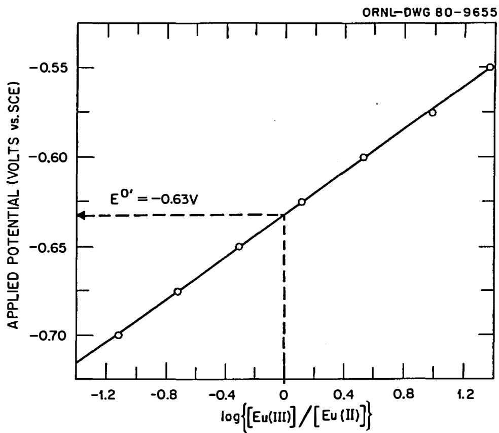
Figure 15. Nernstian plot for the Eu(III)/Eu(II) redox couple in 1 M KCl. pH 6.
