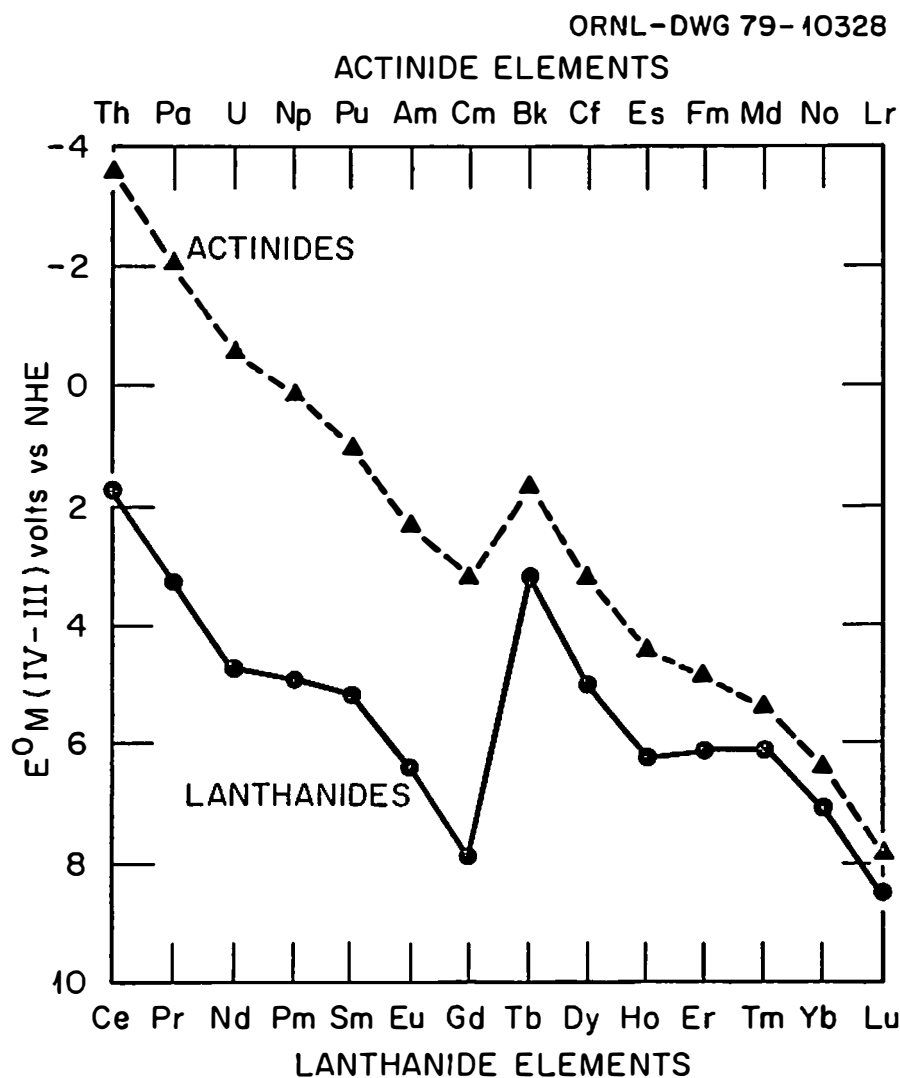
Figure 2. Standard reduction potentials for M(IV)/M(III) redox couples of the lanthanide and actinide elements.
