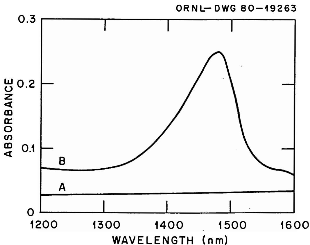
Figure 28. Solution absorption spectra of U(VI) and U(V) in an RVC-OTE. U(VI) initial solution (A) and electrogenerated U(V) (B). RVC-OTE: 100 ppi, 1 mm path length, 1 M KCl/D 2 O at pH (pD) 3, adjusted with DCl, [U(VI)] = 5.0 x 10 -1 M .
