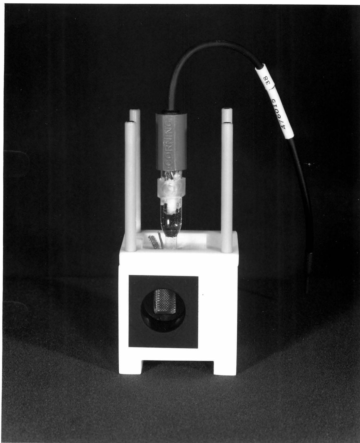
Figure 7. Teflon cell holder with lid in "down" position.
