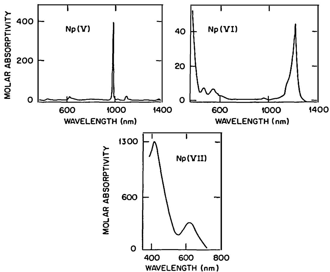
Figure 32. Solution absorption spectra of Np(V) and Np(VI) in 1 M HClO 4 and Np(VII) in 1 M LiOH.
