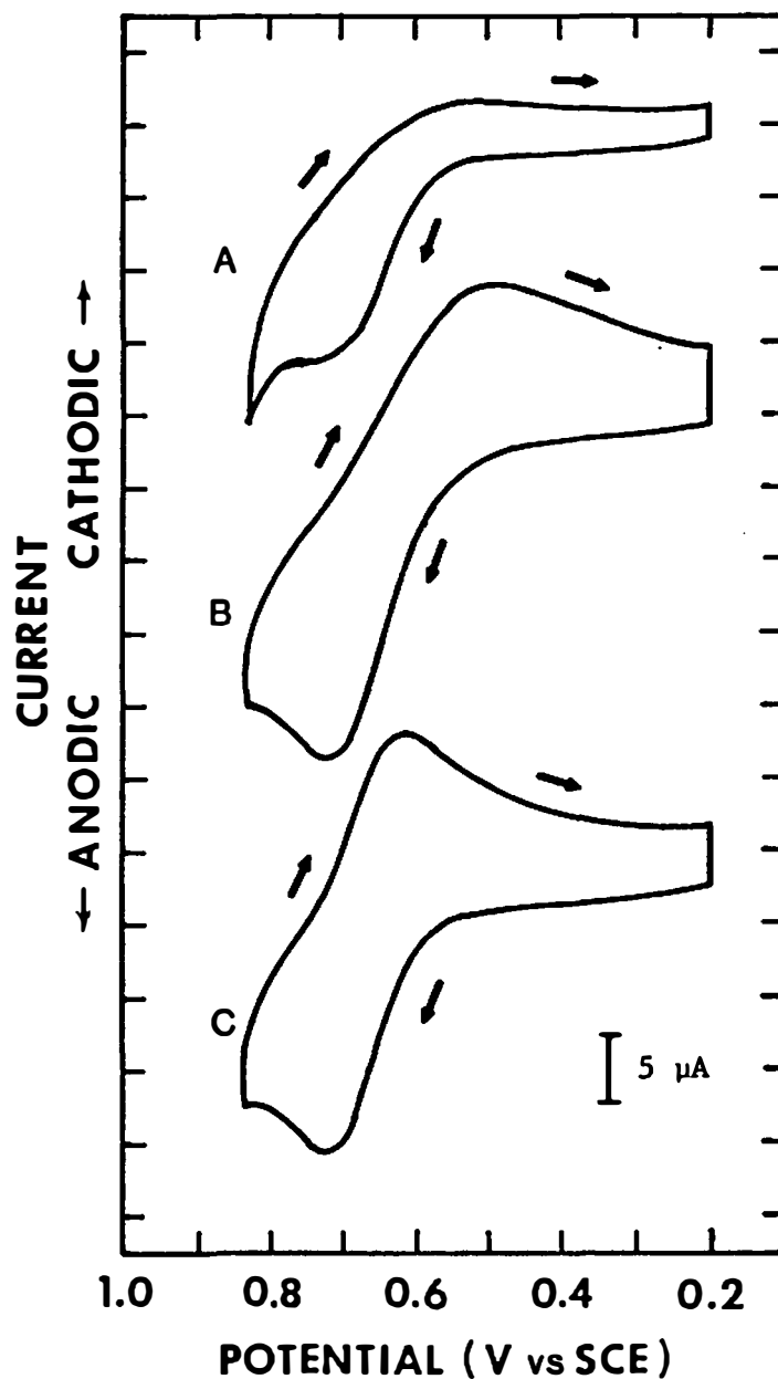
Figure 39. Cyclic voltammograms of Am(III) in 2 M \text{Na}_2\text{CO}_3 at various pH values. pH 12.5 (A), pH 10.2 (B), and pH 9.7 (C), Pt electrode, sweep rate: 50 mV/s, [\text{Am(III)}] = 1.0 \times 10^{-3} \text{ M} .
