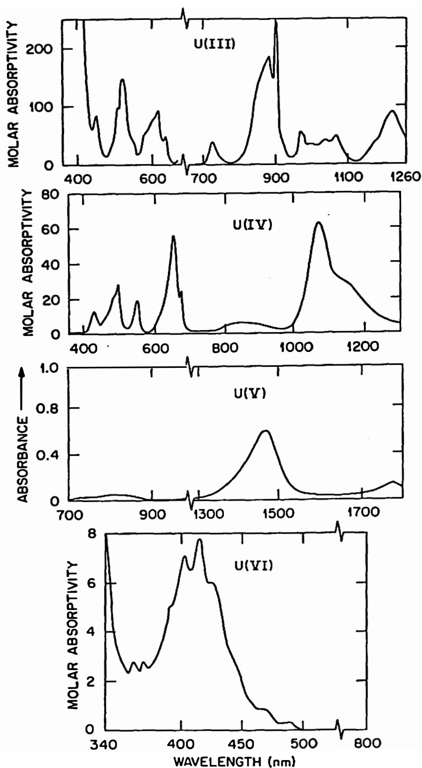
Figure 26. Solution absorption spectra of U(VI, V, IV, and III). In 1 M HClO 4 except U(III) in DClO 4 at pH (pD) 3.09.
