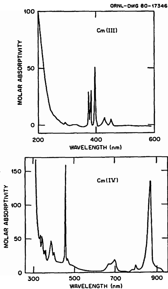
Figure 48. Solution absorption spectra of \text{Cm(III)} in 1 M \text{HClO}_4 and \text{Cm(IV)} in 15 M \text{CsF} at 10.5°C.
