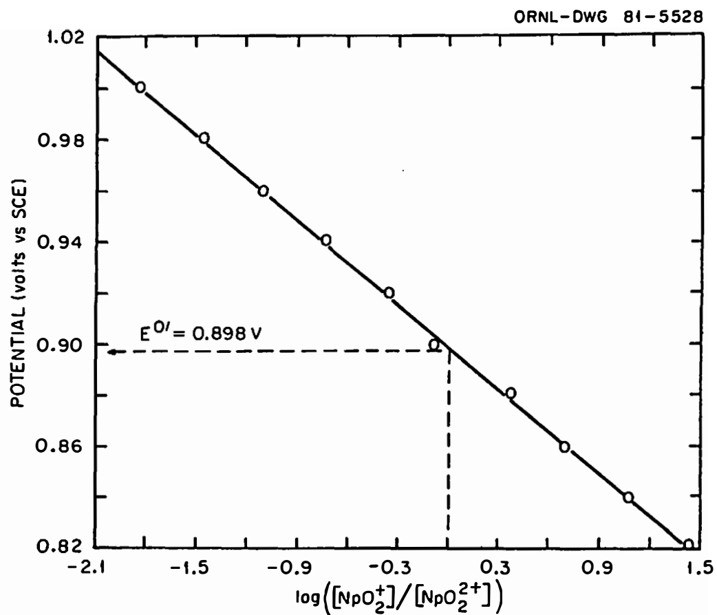
Figure 34. Nernstian plot for the Np(VI)/Np(V) redox couple in 1 M \text{HClO}_4 .
