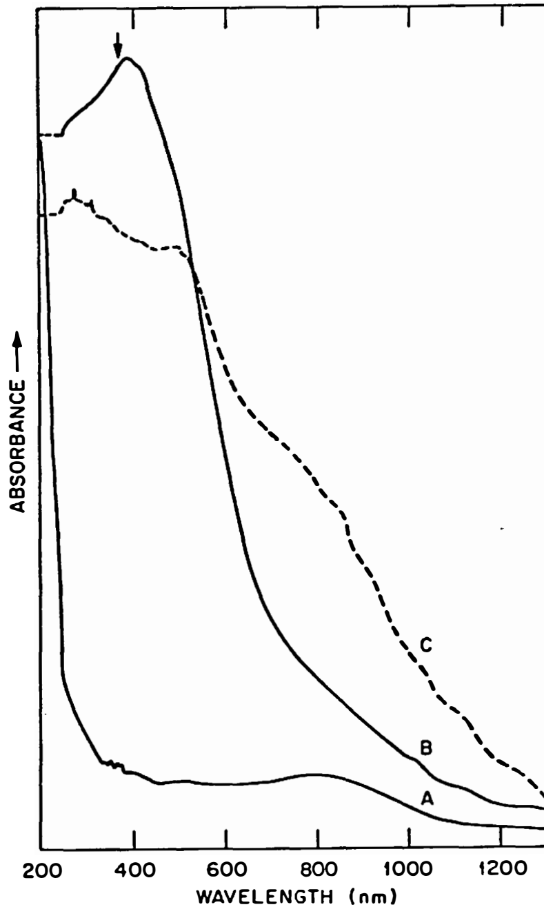
Figure 24. Solid-state reflectance spectra of Tb 2 (CO 3 ) 3 (A), unknown solid (B), and Tb 7 O 12 (C). Arrow indicates absorption maximum of Tb(IV) in carbonate solution.
