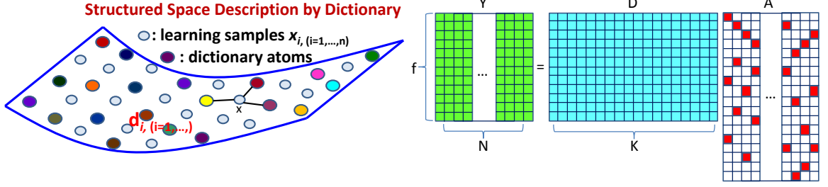
Figure 2.1: A graphic illustration of dictionary learning. Left, dictionary atoms are used for description of the data space structure; Right, feature samples are represented as sparse coefficient vectors.
