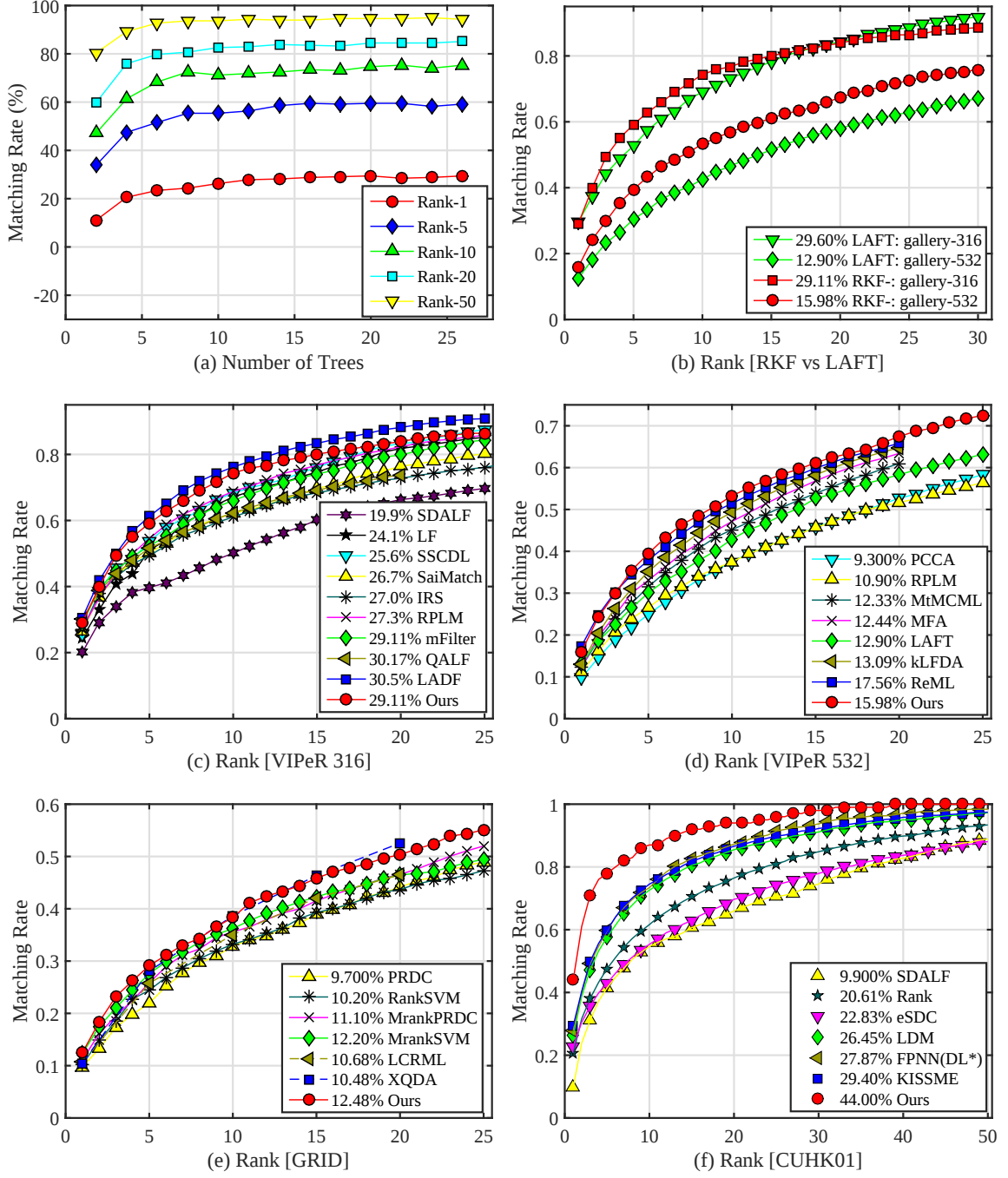
Figure 4.7: Evaluations: (a) Performance comparison of different numbers of trees in random kernel forest. (b) Comparison between RKF and LAFT via CMC curves. (c) CMC curves on VIPeR dataset with 316 gallery images. (d) CMC curves on VIPeR dataset with 532 gallery images. (e) CMC curves on GRID dataset with 900 gallery images. (f) CMC curves on CUHK01 dataset with 100 gallery images.
