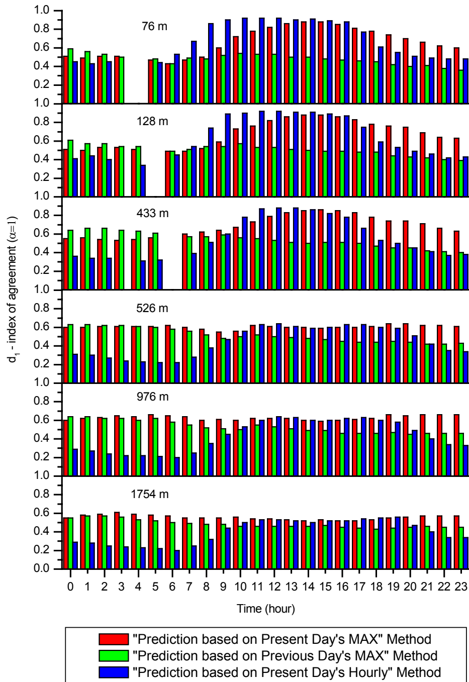
Figure 4-15. Relative Performance in Terms of d_1 (Index of Agreement, \alpha=1 ) for High Elevations (76 m, 128 m, 433 m, 526 m, 976 m, and 1754 m), Using “Prediction based on Present Day’s Maximum,” “Prediction based on Previous Day’s Maximum,” and “Prediction based on Present Day’s Hourly” Methods Full ozone season data (April – October) of 1998 were used.
