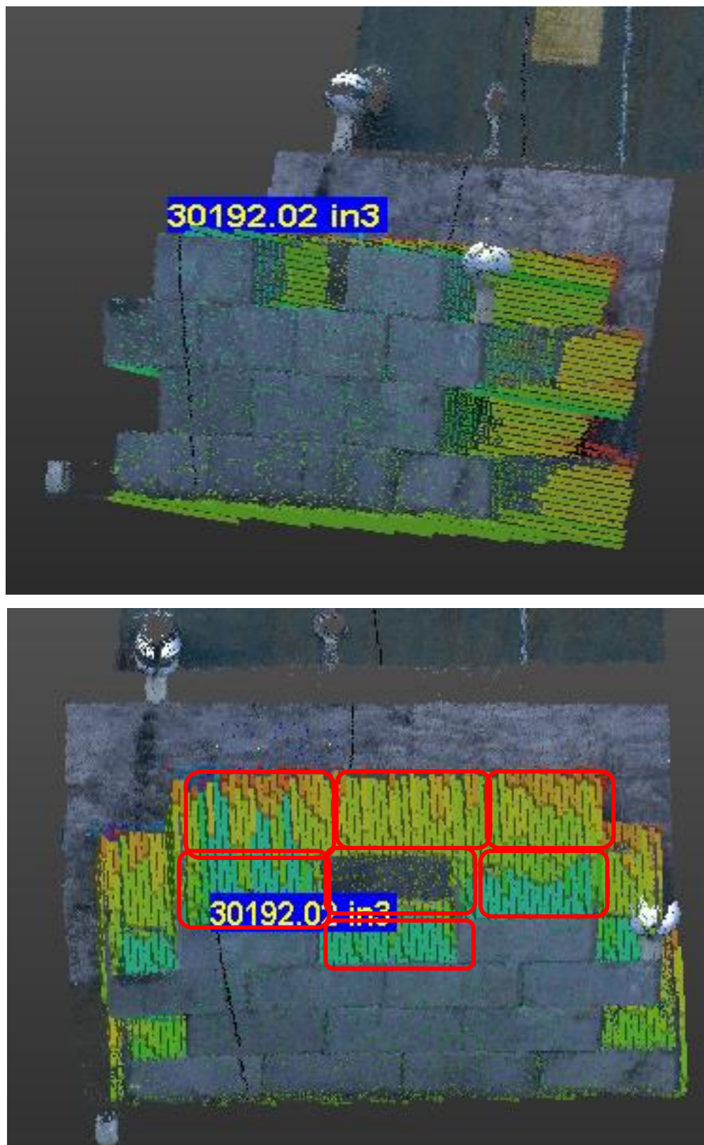
Figure 24: Seven blocks removed from the brick wall.
