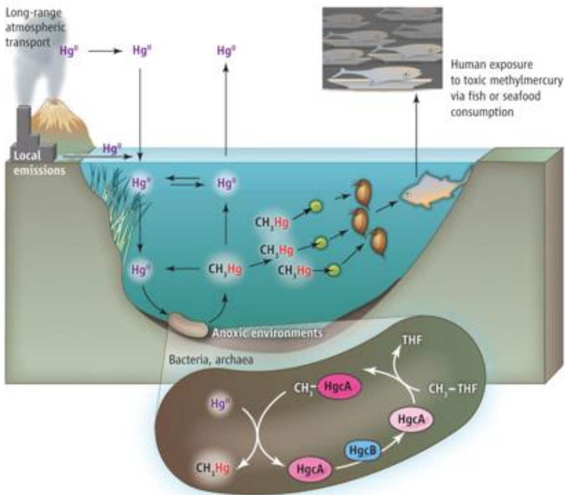
Figure 1: Mercury methylation in the environment (Poulain, A. J. et al. 2013).
