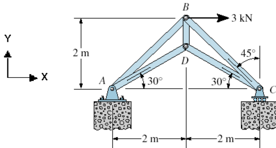
Figure 4.11 Hibbeler Example 6-2
