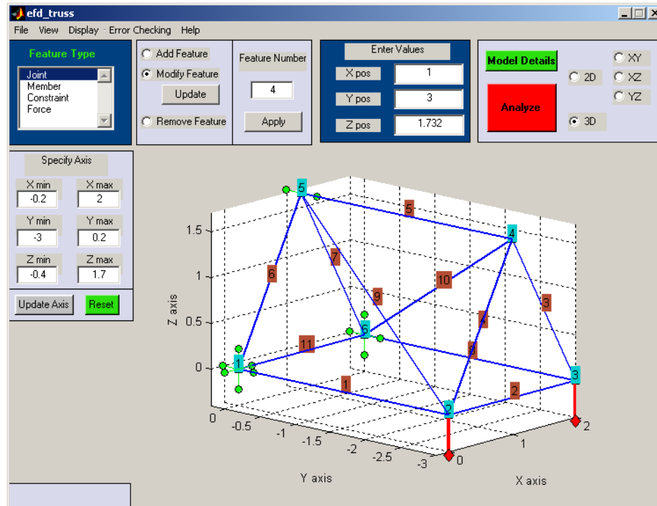
Figure 4.18 Hibbeler Homework 6-62 / 6-63 entered into truss solver
