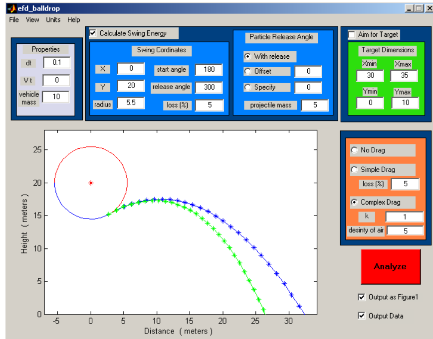
Figure 3.66 Swing Launching Application, Analysis Output
