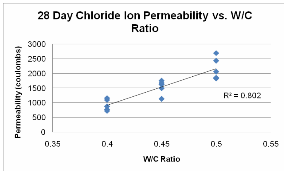
Figure C-10 28 Day Chloride Ion Permeability vs. W/C Ratio
