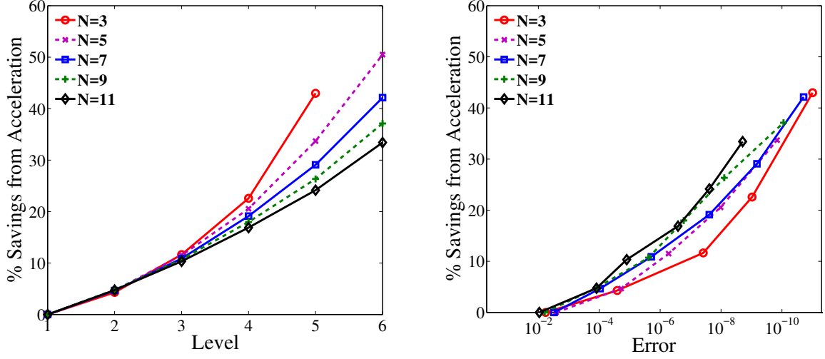
Figure 5.4: Percentage cumulative reduction in CG iterations vs level (left) and error (right) for solving (5.34)–(5.35) using our accelerated approach, with N = 3, 5, 7, 9, 11 , and for correlation length R_c = 1/64 .
