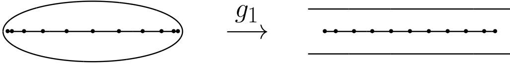
Figure 7.1: The mapping (7.6) takes the Bernstein ellipse E_{1.4} (left) to a strip of half-width 2(1.4 - 1)/\pi \approx .255 .
