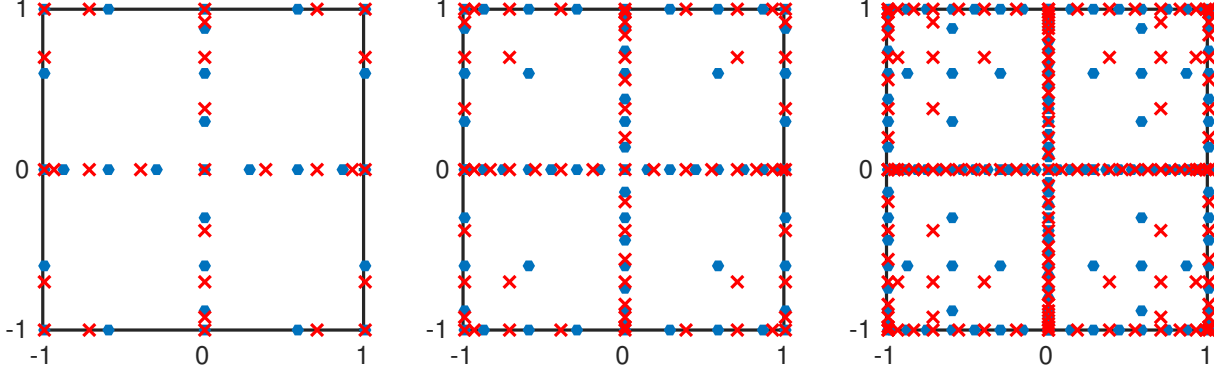
Figure 7.3: Location of the two-dimensional transformed sparse grid nodes (blue dot) using an underlying Clenshaw–Curtis rule, compared to standard Clenshaw–Curtis sparse grids (red x).
