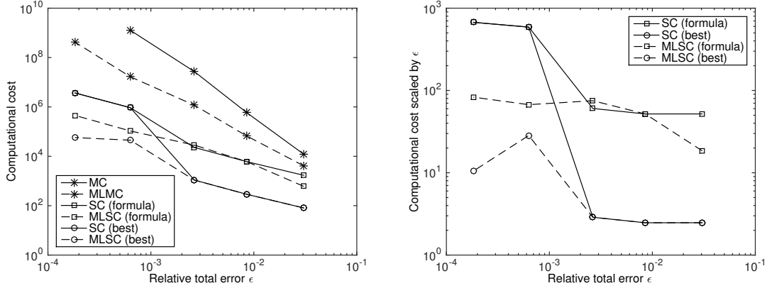
Figure 4.2: D = (0, 1)^2 , N = 10 . Left: computational cost versus relative error \varepsilon . Right: computational cost scaled by \varepsilon^{-1.36} versus relative error \varepsilon .
