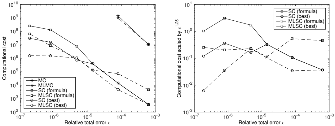
Figure 4.5: D = (0, 1) , N = 20 . Left: computational cost versus relative error \epsilon . Right: computational cost scaled by \epsilon^{-1.25} versus relative error \epsilon .
