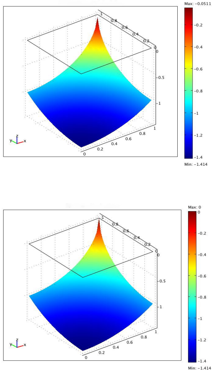
Figure 3.3: Test 3.1c. Computed solution (top) and exact solution (bottom). \epsilon = 0.0125 , h = 0.009
