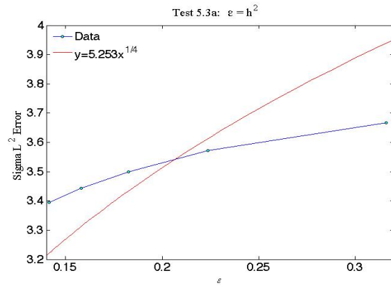
Figure B.11: Test 5.3a. L^2 Error of \sigma_h^\varepsilon
