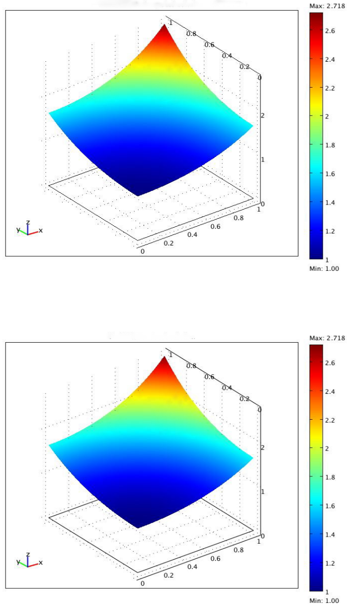
Figure 3.1: Test 3.1a. Computed solution (top) and exact solution (bottom). \epsilon = 0.0125 , h = 0.009
