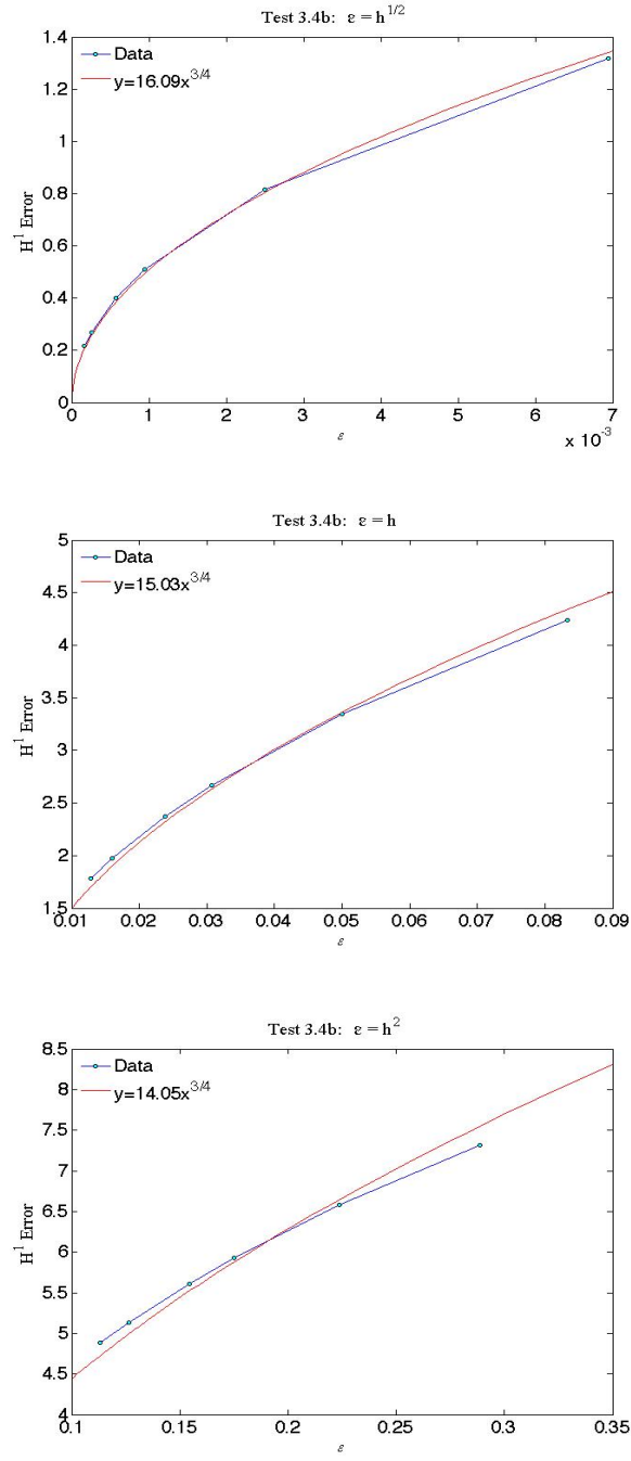
Figure B.4: Test 3.4b. H^1 Error of u_h^\epsilon
