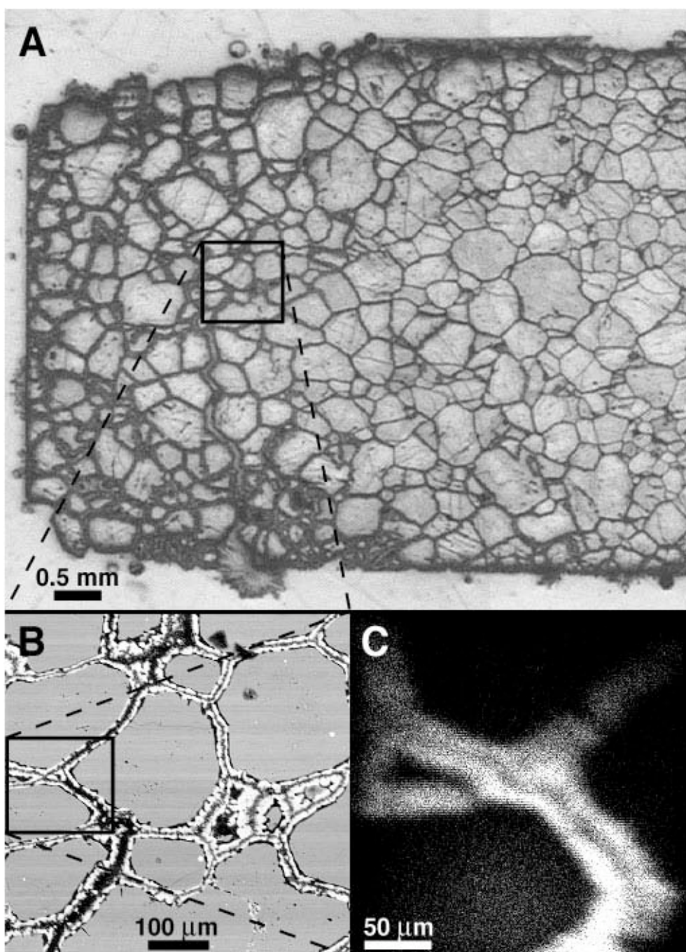
Figure 2. (A) Thin section photomicrograph of experiment LM7 (700 °C, 29 days). Areas of reaction are found primarily along grain boundaries, fractures within grains, and the outer edge of the sample. (B) LM7 BSE image showing distribution of reaction products along grain boundaries. (C) LM7 ^{18}\text{O} ion image showing an ^{18}\text{O} enrichment (white areas) in reaction products. Reaction products exchange with infiltrating isotopically enriched fluid during crystallization.
