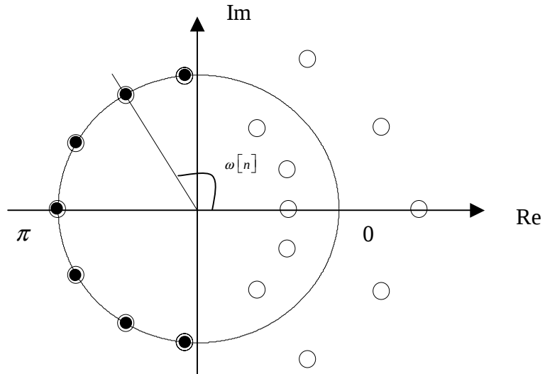
Figure 3.2. Double Zeros on the Unit Circle and the Angles
