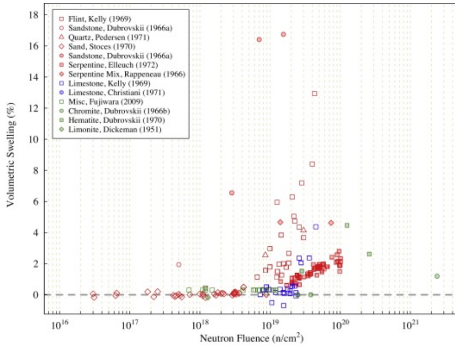
Figure 2.19: Volumetric swelling of concrete vs. neutron fluence. Temperature > 100^\circ\text{C} is indicated with filled symbols. Temperature < 100^\circ\text{C} is indicated with open symbols ( Field et al., 2015 ).
