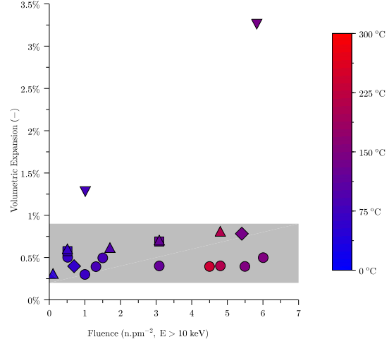
Figure 3: Carbonates RIVEs: calcite ( \circ ); dolomite ( \diamond ); ankerite ( \nabla ); magnesite ( \triangle ); siderite ( \square ). The mark filling color corresponds to the average irradiation temperature.
