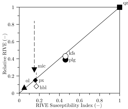
Figure 5: Correlation of the RIVE susceptibility index, I_4 and the relative maximum volumetric expansion, i.e., normalized by that of quartz, i.e., 17.8%, for different groups of minerals – (hbl) hornblende, (kfs): potassium feldspar, (mic): micas, (ol): olivine (data limited to high-magnesian olivine), (plg): plagioclase, (px): pyroxene, (qz): quartz (Whitney and Evans, 2010). Vertical dashed lines indicate the uncertainty on the maximum RIVE expansions.
