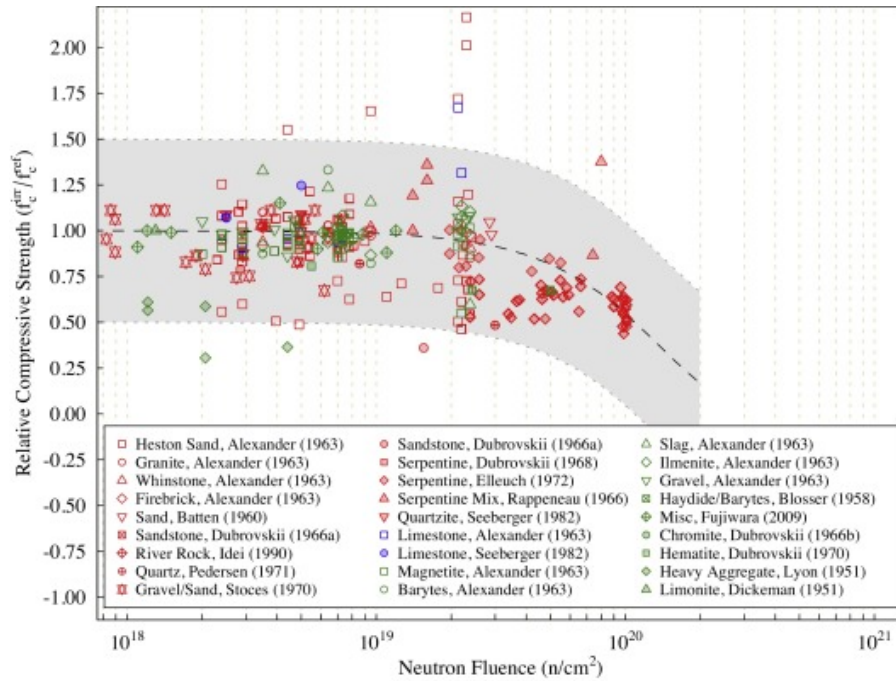
Figure 2.15: Relative compressive strength of irradiated concrete vs. neutron fluence from 1 \times 10^{18} \text{ n.cm}^{-2} to 1 \times 10^{21} \text{ n.cm}^{-2} . Red symbols are siliceous concrete, blue are calcareous concrete, and green are miscellaneous concrete. Temperature > 100^\circ\text{C} is indicated with filled symbols. Temperature < 100^\circ\text{C} is indicated with open symbols (Field et al., 2015).
