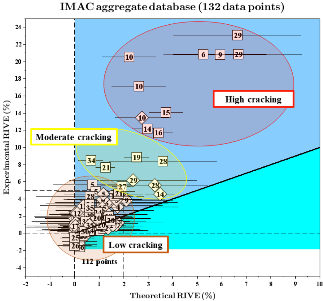
Figure 4.8: Comparison between experimental and theoretical RIVs for the 132 aggregates in the IMAC database. (◇) indicates data points relevant to temperature range in LWRs. (□) indicates data points irrelevant to temperature range in LWRs. Light blue shaded area above the unity line indicates cracked aggregates. Light green shaded area below the unity line indicates contracting or overestimating. Horizontal bars indicate the variation in the theoretical RIVs with 90% confidence.
