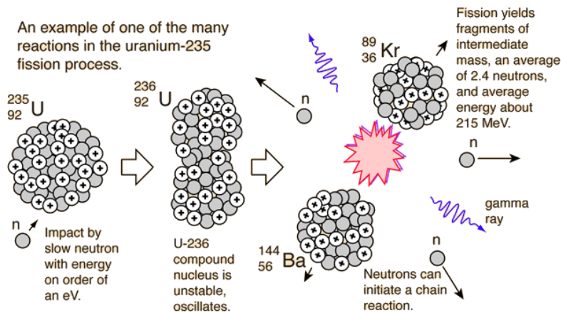
Figure 2.3: An example of a fission reaction in the uranium-235 ( ^{235}_{92}\text{U} ) (Mulligan, 1980).
