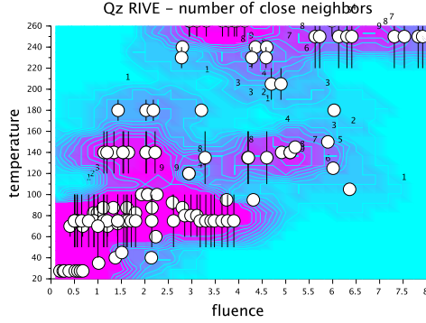
Figure 1: Quartz RIVE database: projection in the fluence ( n^{E>10 \text{ keV}} \cdot \text{pm}^{-2} )-temperature ( ^{\circ}\text{C} ) plane. Color map of the number of neighboring data (radius: \delta < 0.15 ) from light blue to pink areas indicating low to high density of data. Contour plots indicate iso-number of neighbors. (o): IMAC data. Vertical bars indicate the uncertainties on the irradiation temperature.
