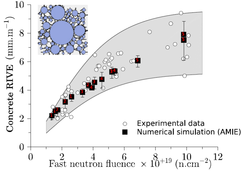
Figure 2.23: Comparison between simulated and the experimentally observed RIVE of Elleuch et al. (1972) data with an example of damage pattern produced at a neutron fluence of 1.3 \times 10^{19} n.cm -2 ( Giorla et al., 2015 ).
