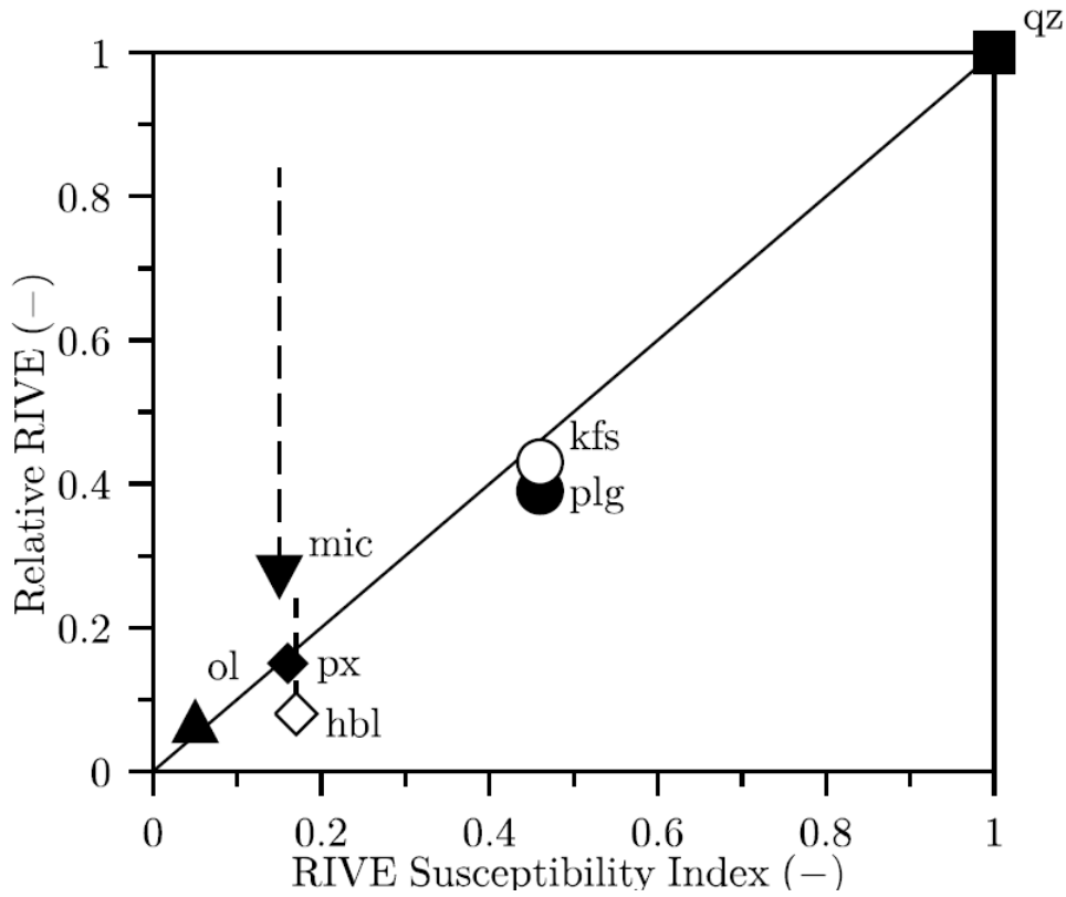
Figure 4.4: Correlation between the maximum normalized RIVE to that of quartz, and the RIVE susceptibility index ( I ). (ol): olivine; (hbl): hornblende; (kfs): potassium feldspar; (mic): micas; (plg): plagioclase; (px): pyroxene; (qz): quartz. Vertical dashed line indicates the uncertainty in maximum RIVEs.
