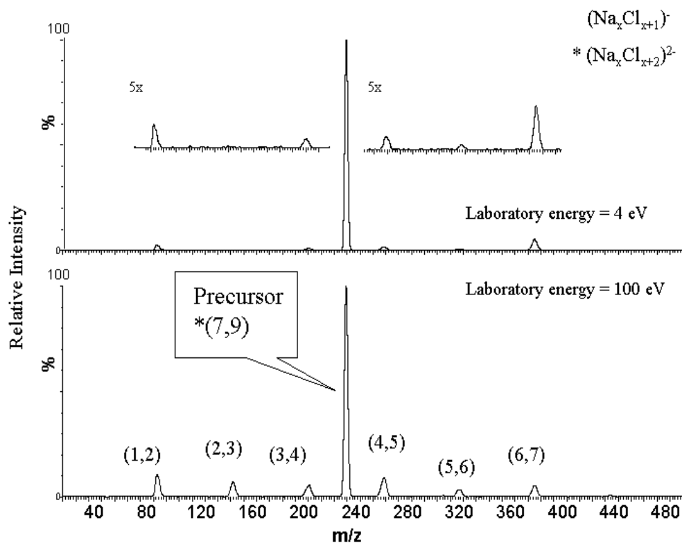
Figure 4.5 Collision-induced dissociation of \text{Na}_7\text{Cl}_9^{2-} (240 amu) at laboratory energies of 4 and 100 eV. We abbreviated the ions such as \text{NaCl}_2^- , and \text{Na}_6\text{Cl}_7^- as (1,2) and (6,7) for brevity.
