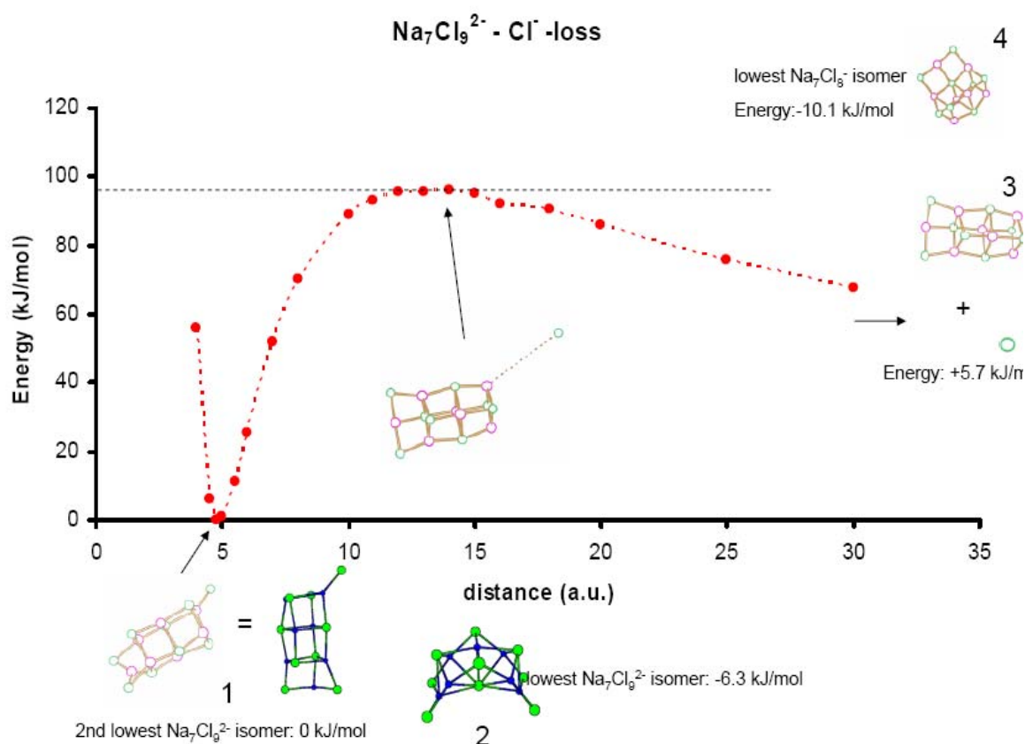
Figure 4.11 Barrier potential for dissociation of \text{Na}_7\text{Cl}_9^{2-} into \text{Na}_7\text{Cl}_8^- and \text{Cl}^- . The barrier height for the loss of \text{Cl}^- is about 95 KJ/mol (0.99 eV).
