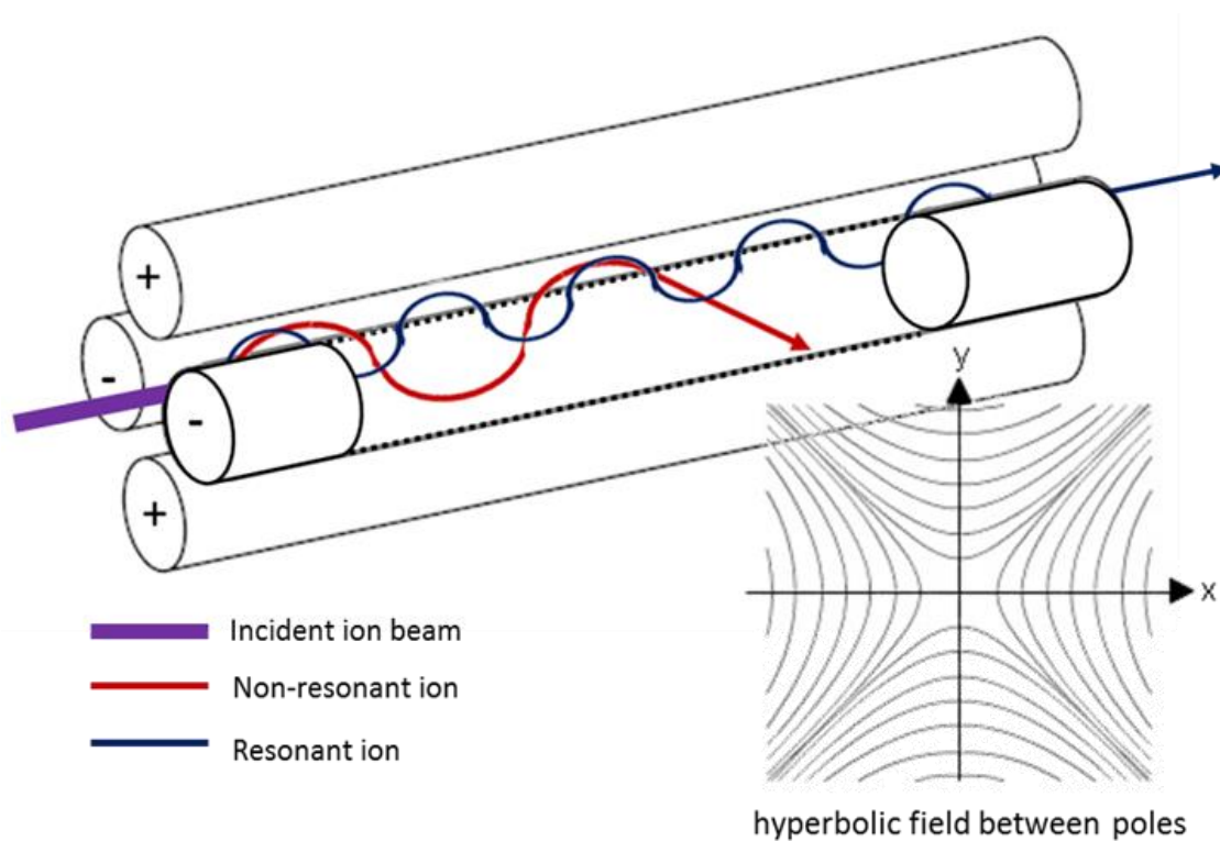
Figure 2.5. Schematic of the quadrupole mass analyzer with cylindrical rods and associated hyperbolic field.
