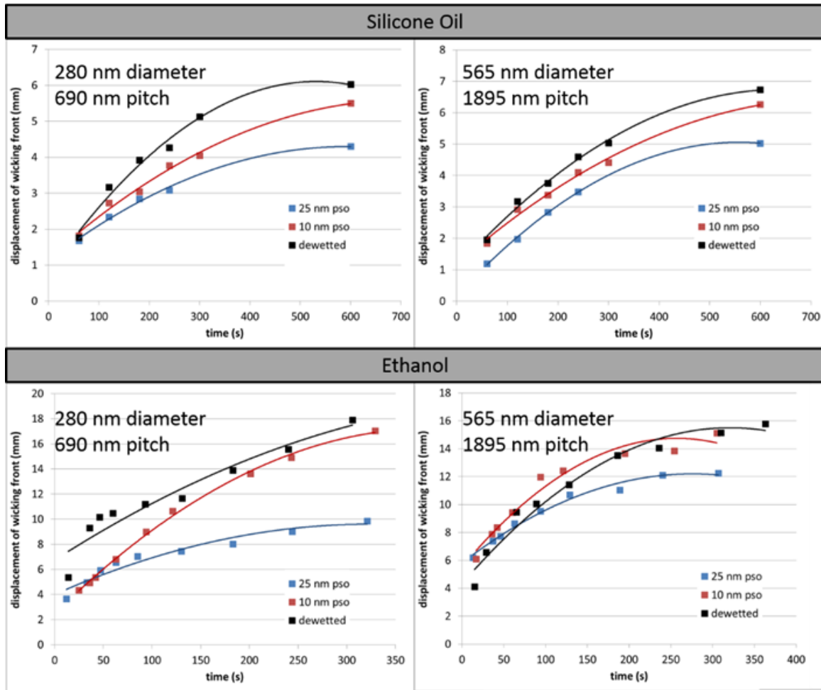
Figure 5.10. Wicking dynamics of both silicone oil and ethanol for stochastic nanopillar arrays with average diameters of 280 and 565 nm with 0, 10, and 25 nm of PSO.
