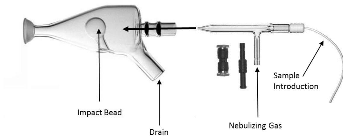
Figure 2.1. A low-volume conical spray chamber fitted with a fixed impact bead and a high performance glass concentric nebulizer.
