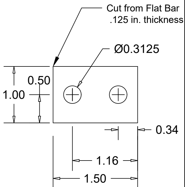
Piece B
