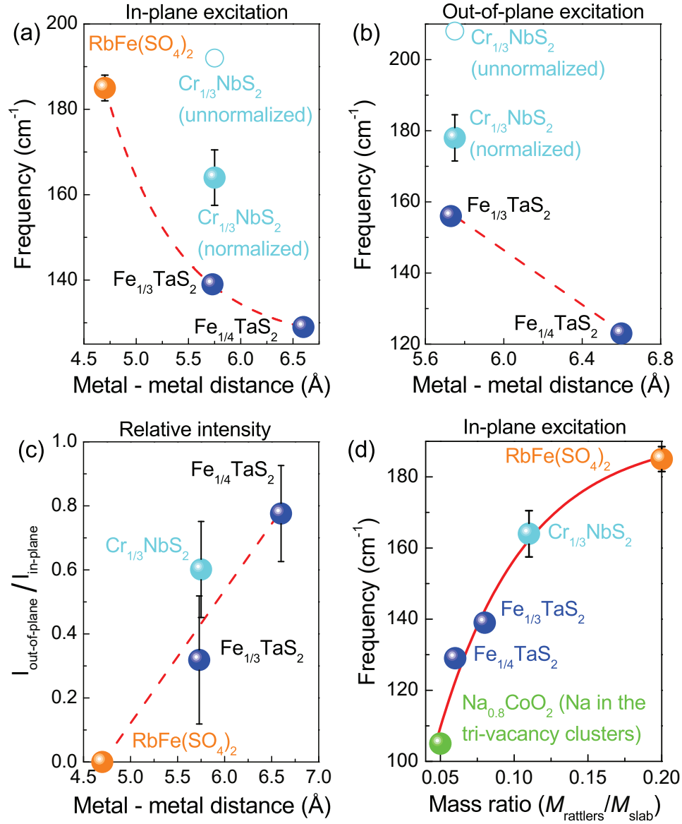
Figure 5.5: (a) Frequency of the in-plane metal monolayer excitation vs. in-plane metal-metal distance in \text{Fe}_x\text{TaS}_2 ( x = 1/4 and 1/3 ) and the analog materials. Results from \text{Cr}_{1/3}\text{NbS}_2 are normalized by the mass of the transition metal center as well as the slabs to better compare with the Fe-containing series. (b) Out-of-plane monolayer excitations as a function of in-plane metal-metal distance. (c) Relative intensity of the out-of-plane to in-plane rattling mode vs. in-plane metal-metal distance. (d) In-plane frequency vs. mass ratio between the intercalated metal monolayer and the chalcogenide slab. The red line is a fit to Eqn. 5.2. We find \omega_{R,\text{max}} = 192 \text{ cm}^{-1} and \kappa = 0.059 .
