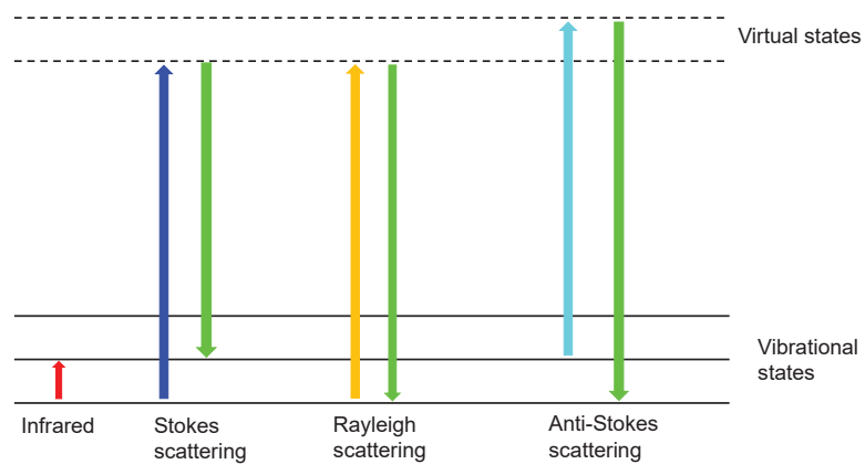
Figure 3.4: Schematic energy diagram which shows the process of Stokes, Rayleigh and Anti-Stokes scattering, as well as the concept of IR spectroscopy.
