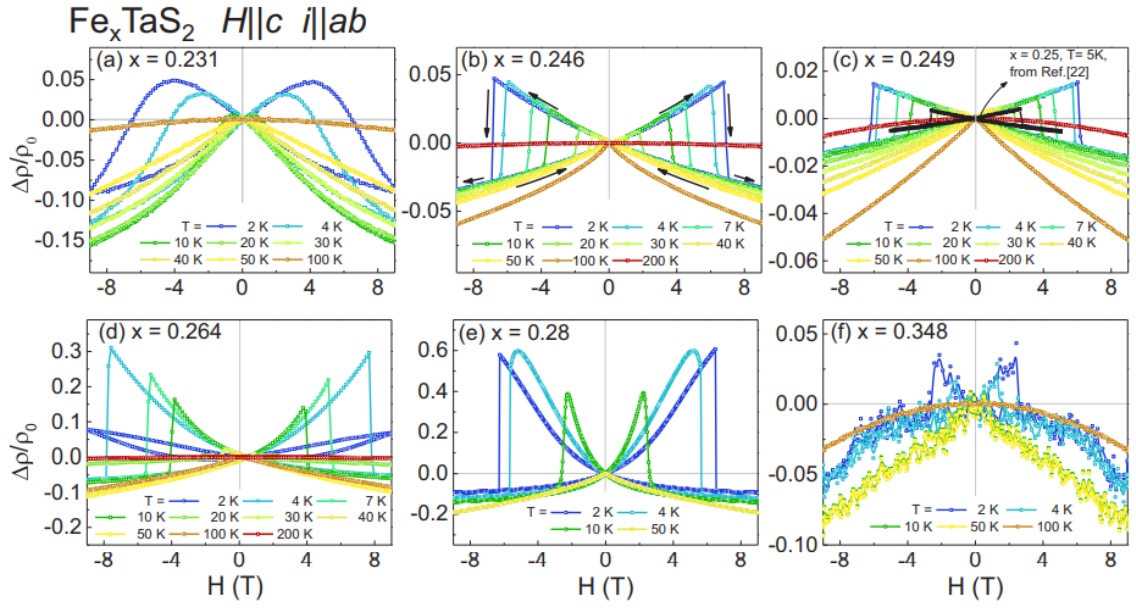
Figure 2.26: Magnetoresistance of \text{Fe}_x\text{TaS}_2 at (a) x = 0.231 , (b) 0.246, (c) 0.249, (d) 0.264, (e) 0.280, and (f) 0.348. Arrows in (b) indicate the field sweep direction [12].
