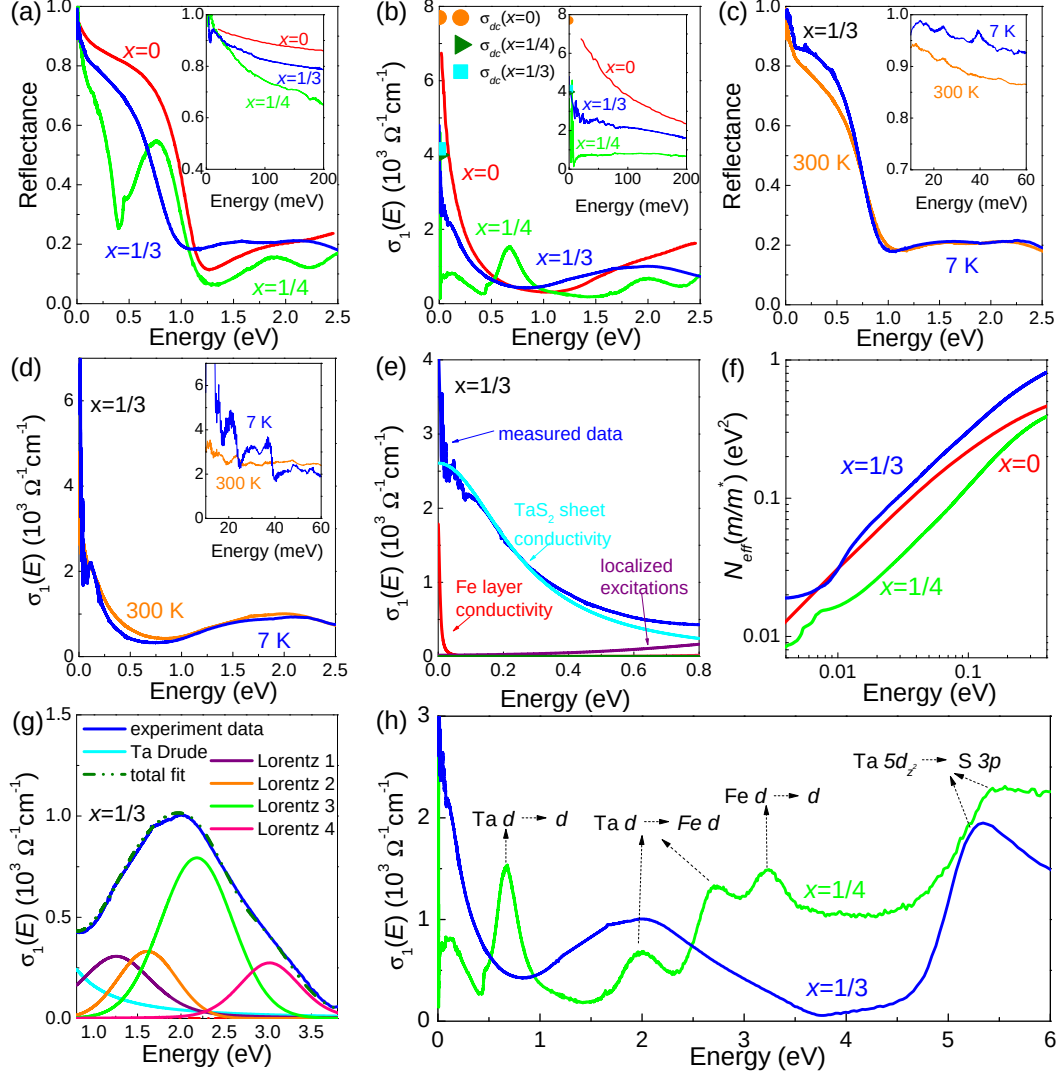
Figure 4.1: (a) Reflectance of \text{Fe}_{1/4}\text{TaS}_2 , \text{Fe}_{1/3}\text{TaS}_2 , and 2\text{H-TaS}_2 . The 2\text{H-TaS}_2 data is reproduced from Ref. 79. Inset: close-up view of the low energy response. (b) Optical conductivity of these materials. Literature values of the dc conductivity [184–186] are also plotted; \sigma_1(E) extrapolates to these values reasonably well. (c) Reflectance of \text{Fe}_{1/3}\text{TaS}_2 at 300 and 7 K. (d) Optical conductivity of the x=1/3 material at 300 and 7 K. Inset displays a close-up view of low energy response. (e) Close-up view of the two Drude oscillators needed to fit the response of \text{Fe}_{1/3}\text{TaS}_2 . (f) Oscillator strength sum rule for the x=0 , 1/4 , and 1/3 compounds. (g) Drude-Lorentz fit of the localized excitations in \text{Fe}_{1/3}\text{TaS}_2 . (h) Optical conductivity of \text{Fe}_{1/4}\text{TaS}_2 and \text{Fe}_{1/3}\text{TaS}_2 highlighting the difference in the localized excitations.
