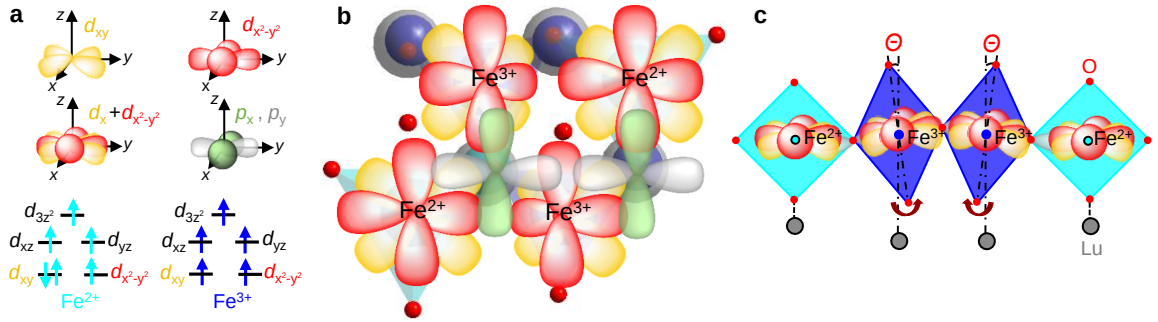
Figure 6.10: Schematic view of the in-plane orbital overlap and the consequences of Lu-layer distortion. a Schematic view of the Fe d_{xy} and d_{x^2-y^2} orbitals + the O p_x and p_y orbitals. The ground state energy diagrams for the \text{Fe}^{2+} and \text{Fe}^{3+} sites are shown as well. b Top view of the \text{LuFe}_2\text{O}_4 double layer in the self-doped structure showing how tilting of the \text{FeO}_5 trigonal bipyramids modifies hybridization. This changes the overlap of the in-plane orbitals. c Schematic side-on view of a hypothetical linear array of \text{FeO}_5 trigonal bipyramids and the rotation and elongation that result from Lu-layer distortion. The tilting and elongation is highly exaggerated in this rendering, and the O p_x and p_y orbitals are omitted for simplicity.
