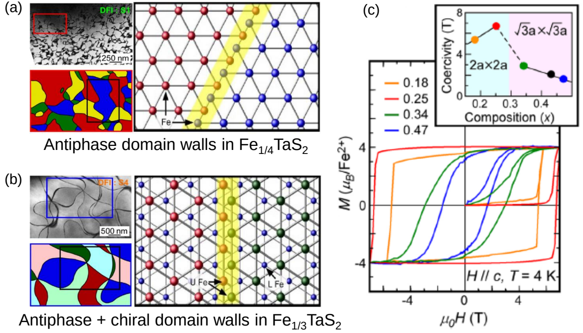
Figure 1.2: (a,b) Domain and domain wall patterns in \text{Fe}_{1/4}\text{TaS}_2 and \text{Fe}_{1/3}\text{TaS}_2 , respectively. (c) Magnetic hysteresis curves of x = 0.18, 0.25, 0.34 , and 0.47 . These curves were measured at 4 K in magnetic fields along the c axis. Note that x = 0.18 and 0.25 show the 2a \times 2a -type superstructure, whereas x = 0.34 and 0.47 exhibit the \sqrt{3}a \times \sqrt{3}a -type one. The inset shows the magnetic coercivity as a function of Fe composition [6].
