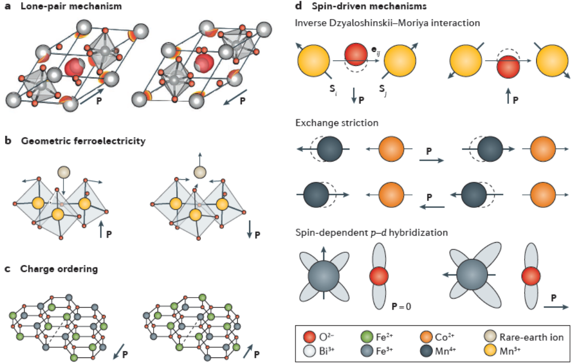
Figure 2.3: a , Lone-pair ferroelectricity in \text{BiFeO}_3 . The isosurface (red) of the electron localization function illustrates the lone-pair. b , A tilt and deformation of \text{MnO}_5 bipyramids induces geometric ferroelectricity in h\text{-RMnO}_3 . c , Charge ordering in \text{LuFe}_2\text{O}_3 creates alternating layers with \text{Fe}^{2+} / \text{Fe}^{3+} ratios of 2:1 and 1:2. This can create a spontaneous polarization between the two layers. d , Mechanisms for spin-induced ferroelectricity [37, 49]. Figure is taken from Ref 37.
