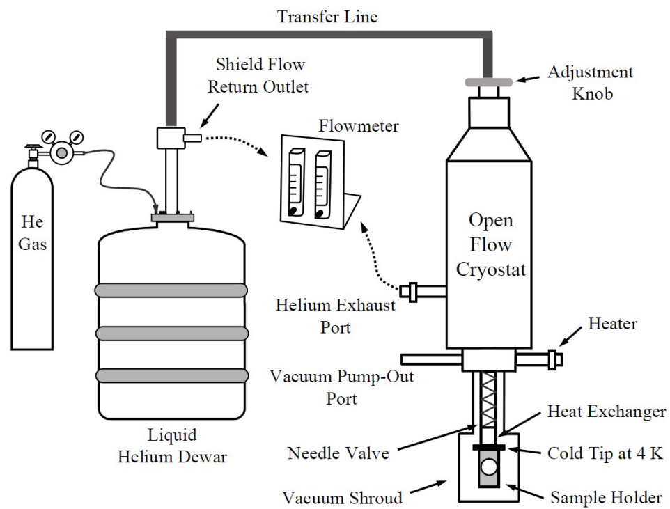
Figure 3.15: Set-up of LT-3-110 Heli-Tran liquid transfer line and cryostat [168].
