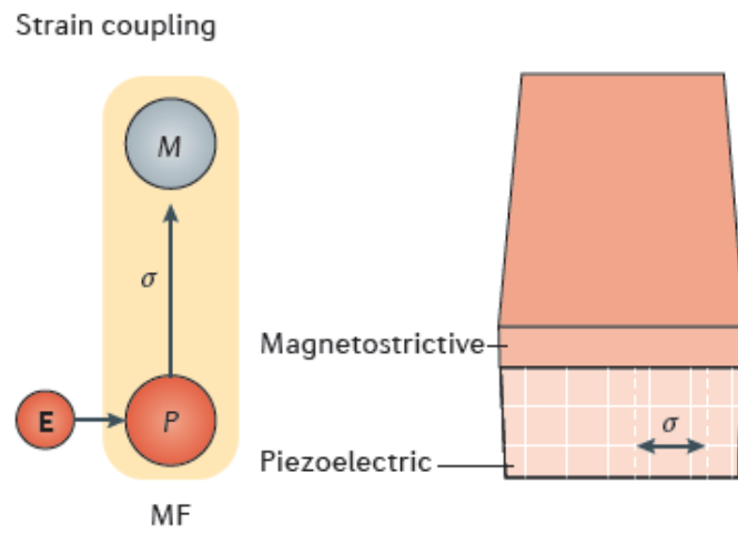
Figure 2.5: the magnetoelectric coupling between a piezoelectric and magnetostrictive constituent is established via strain \sigma [37].
