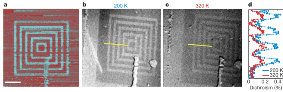
Figure 2.29: a , Out-of-plane piezoresponse force microscopy (PFM) image at 300K of the domain structure following electrical poling using a d.c. bias applied to the proximal tip. The “up” and “down” c -oriented domains appear in turquoise and red, respectively. Scale bar, 3 \mu\text{m} . b , c , X-ray magnetic circular dichroism (XMCD) PEEM ratio images from the Fe L_3 edge acquired at 200 K ( b ) and 320 K ( c ). The correlation between the electrical poling and magnetic imaging demonstrates electric-field control of ferrimagnetism at 200 K. d , Comparison of the dichroic signals along the yellow lines in b and c . Figure is taken from ref. 1
