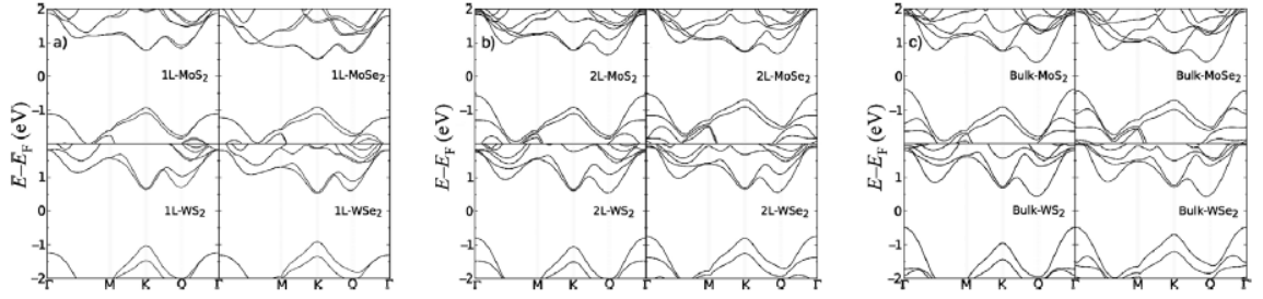
Figure 2.14: Band structure of single layer, (a), bilayer (b), and bulk (c) of MoS 2 , MoSe 2 , WS 2 , and WSe 2 obtained from density functional theory calculations [84, 105]. Dashed vertical lines indicate the position of the Q point in the Brillouin zone [84, 105]. Figure is taken from ref 105.
