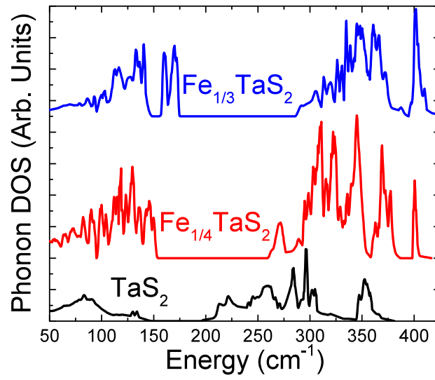
Figure 3.17: The calculated phonon DOS for \text{TaS}_2 (black), \text{Fe}_{1/4}\text{TaS}_2 (red), and \text{Fe}_{1/3}\text{TaS}_2 (blue). The curves have been offset for clarity.
