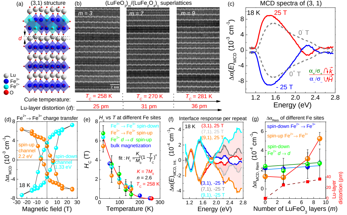
Figure 1.7: (a) Crystal structure of the (3, 1) superlattice. d represents the Lu-layer distortion. (b) STEM images of the (3, 1), (7, 1), and (9, 1) superlattices. Below displays the magnetic Curie temperatures and the amplitude of Lu-layer distortion for each superlattice. (c) Magnetic circular dichroism spectra of the (3, 1) superlattice at \pm 25 \text{ T} and 0 \text{ T} . (d) Optical hysteresis loop of the spin-up and spin-down channel \text{Fe}^{2+} \rightarrow \text{Fe}^{3+} charge transfer excitations. (e) Extracted coercivity vs temperature trend for all types of Fe-related excitations. (f) Extracted magnetic circular dichroic spectra of interfaces. (g) Remnant dichroic intensity as a function of superlattice periodicity ( m ) for different types of Fe-related excitations. The Lu-layer distortion vs m is also plotted to show the correlations.
