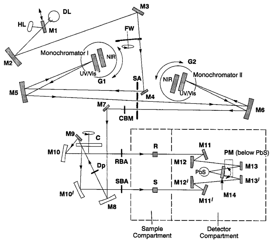
Figure 3.13: Optical layout of Perkin-Elmer λ-900 or -1050 [168].
