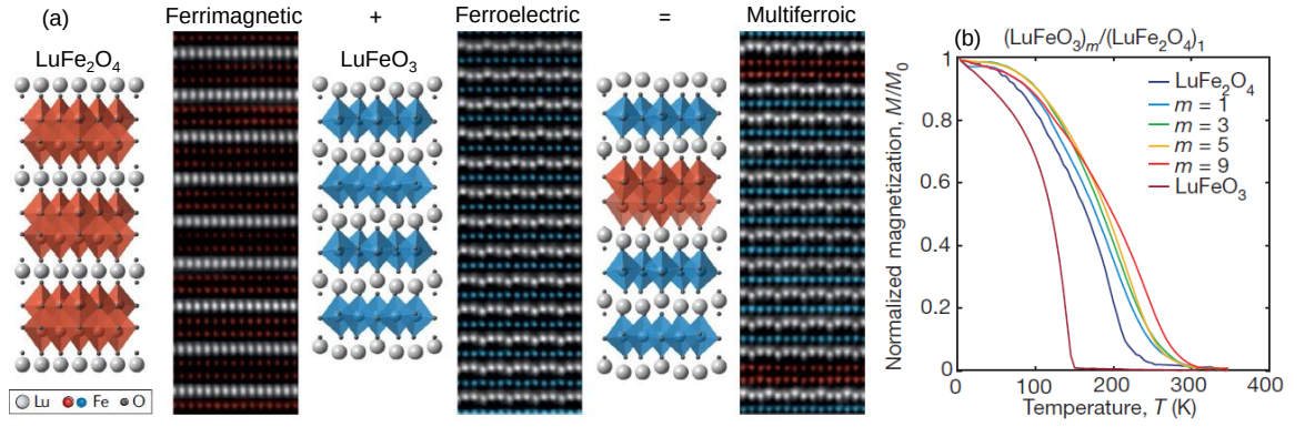
Figure 1.3: (a) crystal structures and STEM images of LuFe 2 O 4 (left), LuFeO 3 (middle), and (\text{LuFeO}_3)_m/(\text{LuFe}_2\text{O}_4)_n superlattices (right), respectively [15]. (b) Magnetization vs temperature for different superlattices [1].
