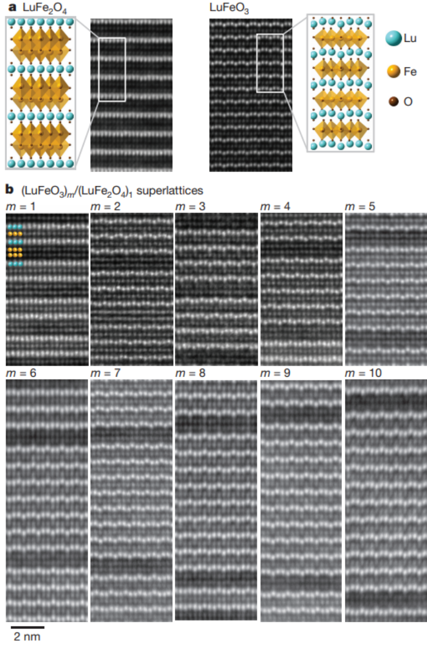
Figure 2.27: a , End-members \text{LuFe}_2\text{O}_4 (left) and \text{LuFeO}_3 (right). b , (\text{LuFeO}_3)_m/(\text{LuFe}_2\text{O}_4)_1 superlattice series for 1 \leq m \leq 10 . Samples are imaged along the \text{LuFeO}_3 P6_3cm [100] zone axis. \text{LuFe}_2\text{O}_4 is imaged down the equivalent zone axis, which, owing to the primitive unit cell of \text{LuFe}_2\text{O}_4 , is the [120] zone axis. Schematics of the \text{LuFe}_2\text{O}_4 and \text{LuFeO}_3 crystal structures are shown in a with lutetium (Lu), iron (Fe) and oxygen (O) in turquoise, yellow and brown, respectively. Figure is taken from Ref. 1
