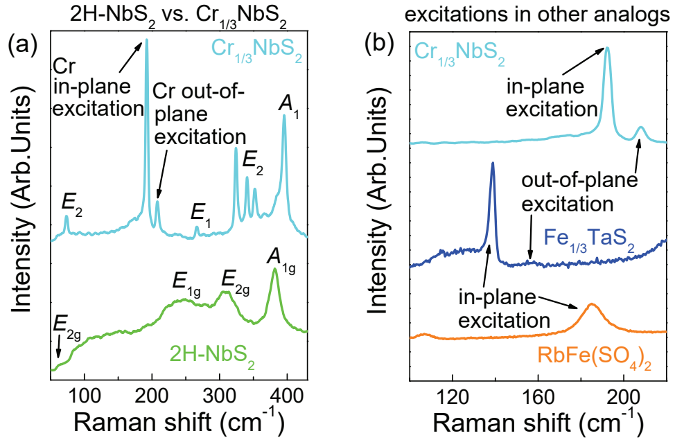
Figure 5.4: (a) Raman scattering spectra of the Cr x NbS 2 family of materials ( x = 0 and 1/3 ) at 300 K. (b) A close-up view of the in- and out-of-plane metal monolayer modes in Cr 1/3 NbS 2 , Fe 1/3 TaS 2 , and RbFe(SO 4 ) 2 .
