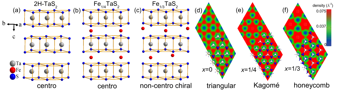
Figure 2.23: (a) Crystal structure of 2H-TaS 2 in the centrosymmetric P6_3/mmc space group [125]. Ta 4+ is at the center of a prism formed by six S 2- centers. (b) Fe 1/4 TaS 2 also belongs to the P6_3/mmc space group [6]. Each Fe center is octahedrally coordinated by six S 2- atoms. Stacking along c is AA type, yielding an expanded 2a \times 2a superlattice. (c) The structure of Fe 1/3 TaS 2 is non-centrosymmetric and chiral (space group P6_322 ) [6]. Stacking along c is alternating (AB) type, yielding a \sqrt{3}a \times \sqrt{3}a superlattice. (d, e, f) Projected charge density in the Fe plane for 2H-TaS 2 , Fe 1/4 TaS 2 , and Fe 1/3 TaS 2 .
