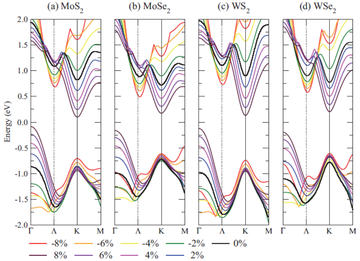
Figure 2.15: The change of highest valence band and lowest conduction band of (a) \text{MoS}_2 (b) \text{MoSe}_2 (c) \text{WS}_2 and (d) \text{WSe}_2 under compressive and tensile biaxial strains [106].
