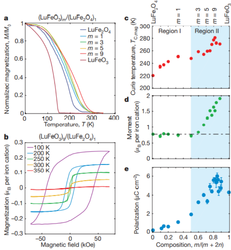
Figure 2.28: a , M–T curves for a series of (\text{LuFeO}_3)_m/(\text{LuFe}_2\text{O}_4)_1 superlattices cooled in a 1-kOe field. b , Loops of the magnetization as a function of the magnetic field for the (\text{LuFeO}_3)_9/(\text{LuFe}_2\text{O}_4)_1 superlattice, at various temperatures. c , The ferromagnetic Curie temperatures T_{C,\text{mag}} extracted from the M–T curves (some of which are shown in a) plotted as a function of the fraction of iron ions that sit in the \text{LuFeO}_3 layers, m/(m+2n) . Regions I and II show data for the (\text{LuFeO}_3)_1/(\text{LuFe}_2\text{O}_4)_n and (\text{LuFeO}_3)_m/(\text{LuFe}_2\text{O}_4)_1 series, respectively. The Curie temperature reaches a maximum of 281K for the (\text{LuFeO}_3)_9/(\text{LuFe}_2\text{O}_4)_1 compound. d , The total moment per iron cation in \text{LuFe}_2\text{O}_4 at 50K assuming the moment of \text{LuFeO}_3 remains constant. The measured moment of end-member \text{LuFe}_2\text{O}_4 is displayed as a horizontal line for reference. e , Average polarization from HAADF-STEM for superlattice layering plotted as a function of composition. Ferroelectric distortions are observed for the (\text{LuFeO}_3)_m/(\text{LuFe}_2\text{O}_4)_1 superlattices with m \geq 2 ( m/(m+2n) \geq 0.5 ). Figure is taken from Ref. 1.
