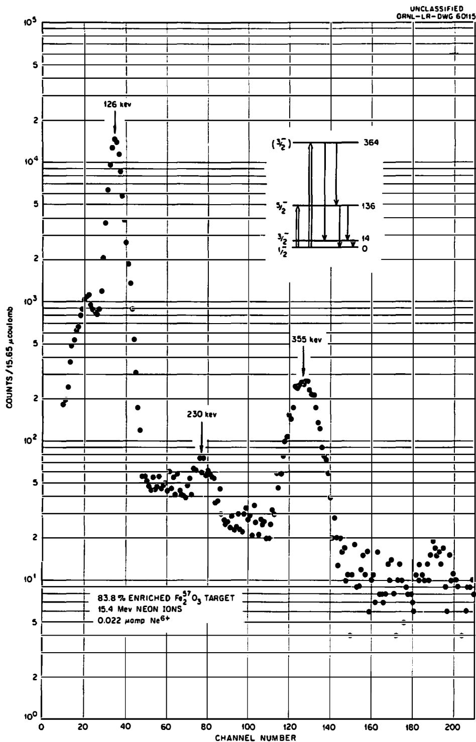
Fig. 27. Scintillation Pulse-Height Spectrum Produced by Bombardment of an \text{Fe}^{57}\text{O}_3 Target With Neon Ions.
