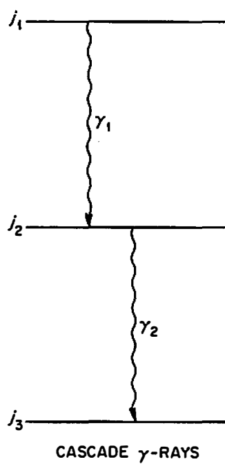
Fig. 3. Analogy Between Cascade \gamma -Ray and Coulomb Excitation Angular Distributions.
