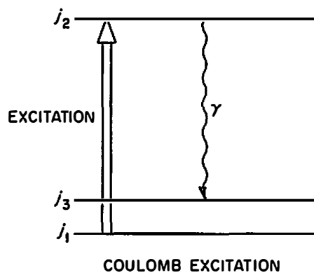
Fig. 3. Analogy Between Cascade \gamma -Ray and Coulomb Excitation Angular Distributions.
