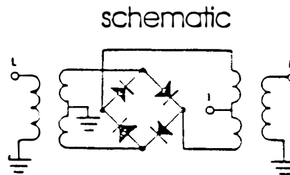
Figure 17. Double balanced mixer schematic.
