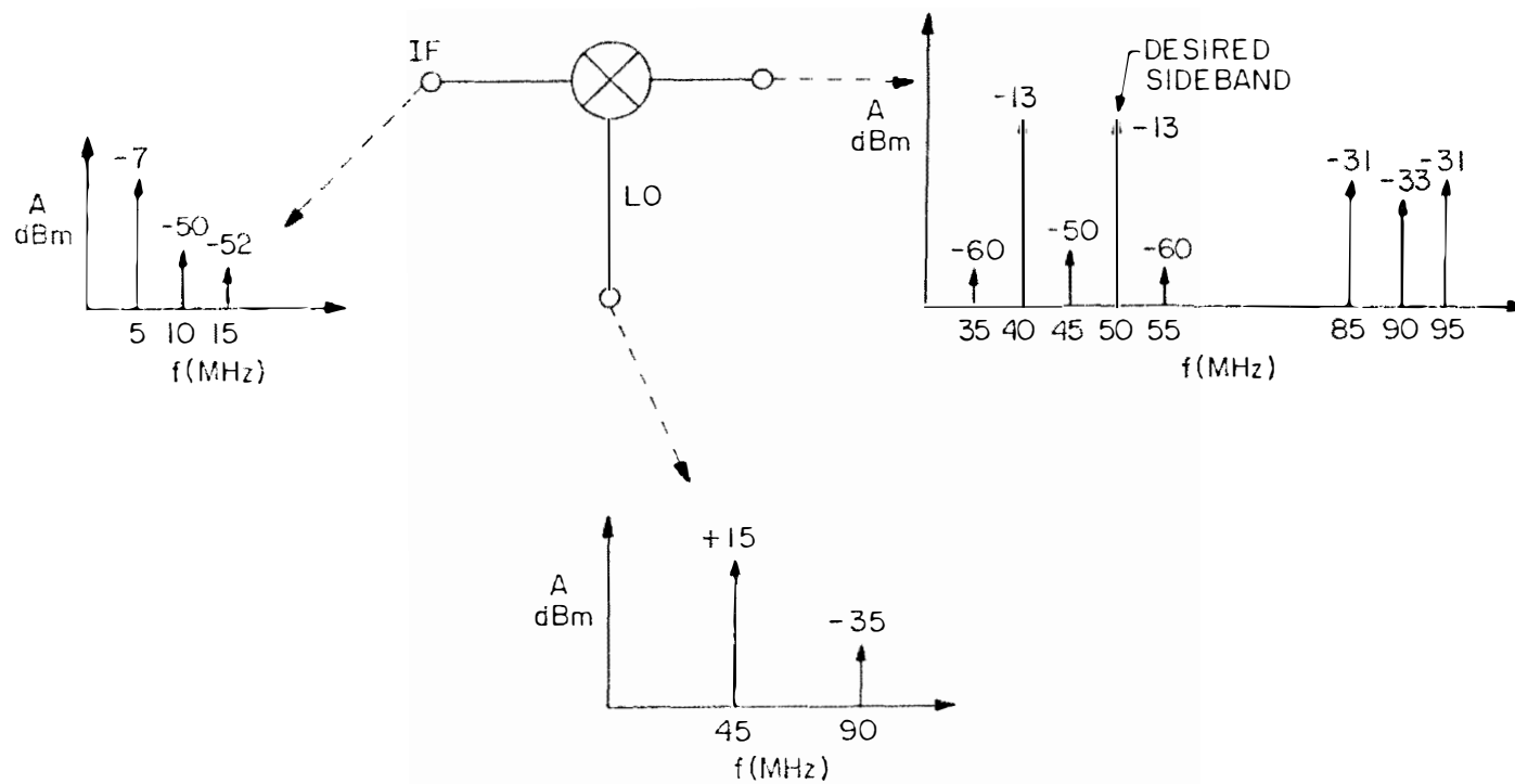
(a) 45 MHz Local Oscillator Spectrum
