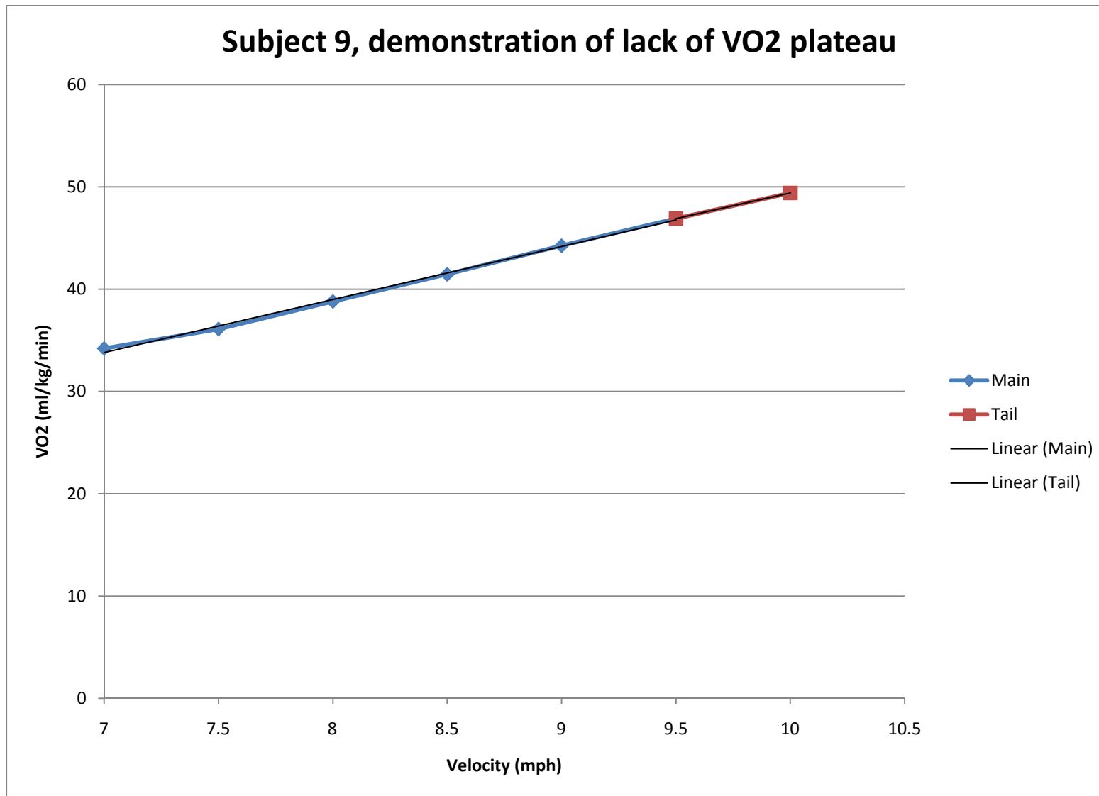
Figure 2, Demonstration of Lack of VO 2 Plateau
