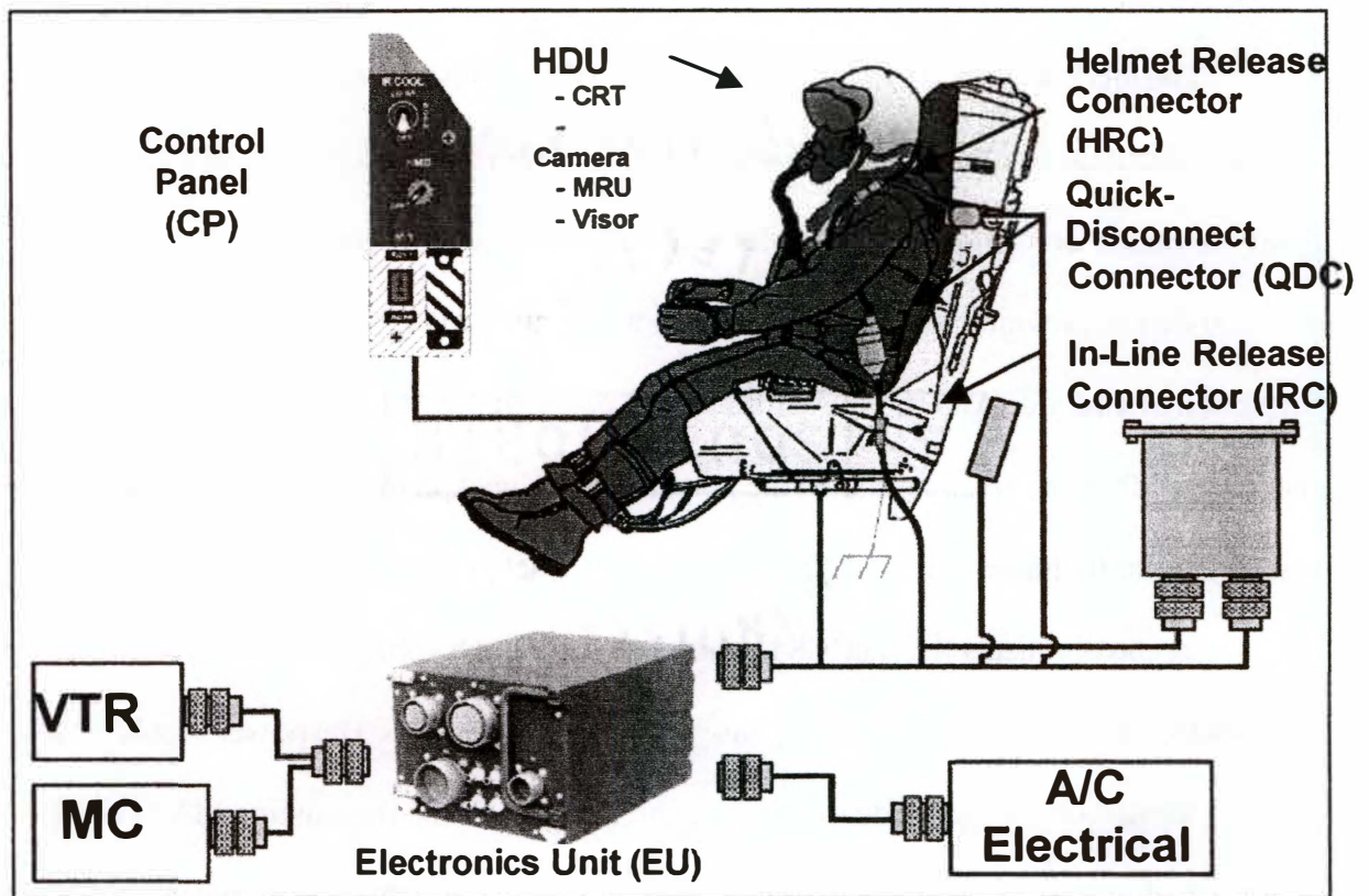
Figure 3 Overall Schematic
