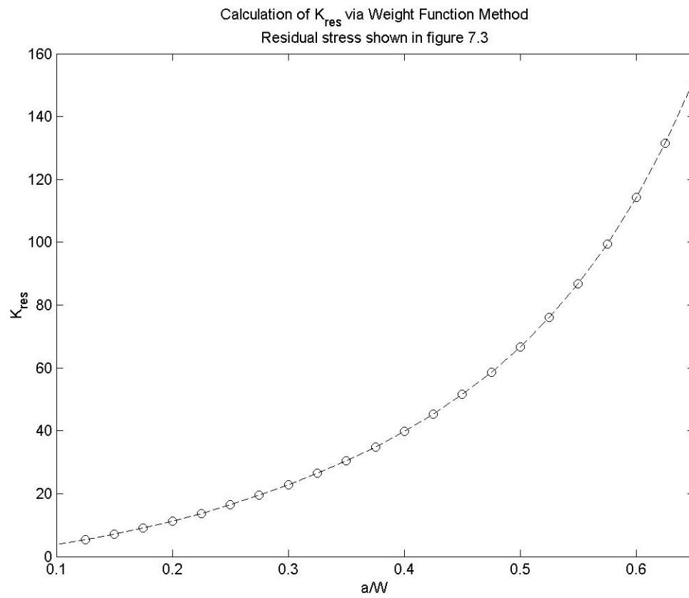
Figure 7.4: K_{res} Calculated Via Weight Function Method
