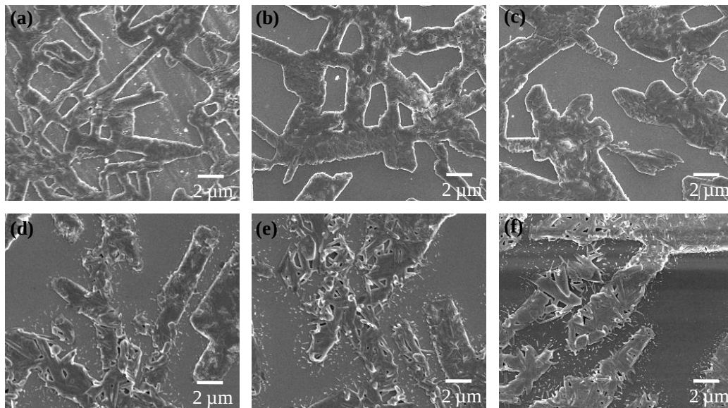
Figure 5.4. SEM images of a perovskite films coated using DMSO on \text{TiO}_2/\text{ITO}/\text{glass} substrates at substrate temperature of (a) 60^\circ\text{C} (b) 75^\circ\text{C} , (c) 90^\circ\text{C} , (d) 105^\circ\text{C} , (e) 120^\circ\text{C} , and (f) 130^\circ\text{C} .
