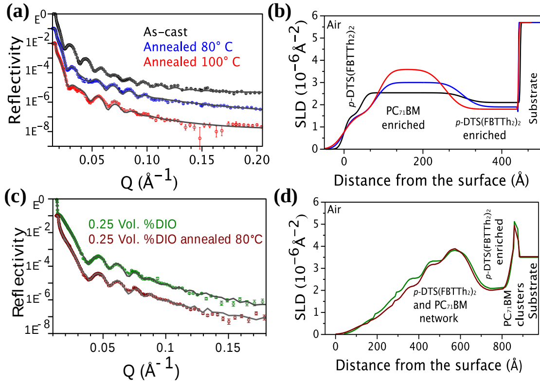
Figure 4.2. a) Experimental (shown as symbols) and modeled (solid lines) NR curves for as-cast and annealed (80 and 100 °C) Al 2 O 3 /p-DTS(FBTTh 2 ) 2 :PC 71 BM films without DIO. b) The SLD profiles as a function of distance from the surface obtained after fitting the experimental data shown in (a). c) Experimental (shown as symbols) and modeled (solid lines) NR curves for as-cast and annealed (80 °C) SiO 2 /p-DTS(FBTTh 2 ) 2 :PC 71 BM films with 0.25 vol% DIO. d) The SLD profiles as a function of distance from the surface from fitting the experimental data of (c).
