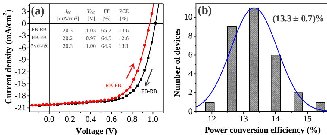
Figure 6.2. J-V curve of a typical device with furnace-annealed TiO 2 layer scanned at different directions under standard illumination (100 mW/cm 2 ). (b) Histogram of PCEs measured for 30 devices, fabricated with furnace annealed (500 °C) compact TiO 2 as electron transport layer.
