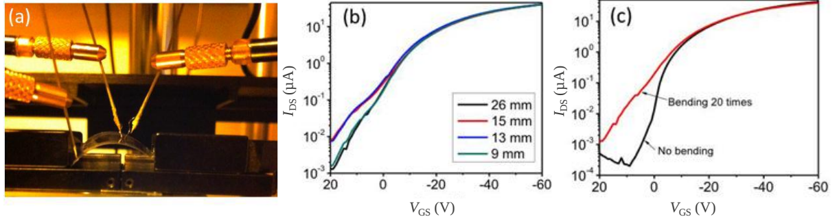
Figure 7.9. (a) A digital camera image of the OFET devices on a PET substrate in a bent configuration during electrical measurement. (b) No significant change of transfer characteristics of OFET with different bend radius values, R (26 mm, 15 mm, 13 mm, 9 mm). (c) No significant change of transfer characteristics of OFET after 20 cycles bending ( R = 9 mm) are observed (before: black line, after: red line). The transfer curves are measured in the saturation regime at a drain bias of -40 V.
