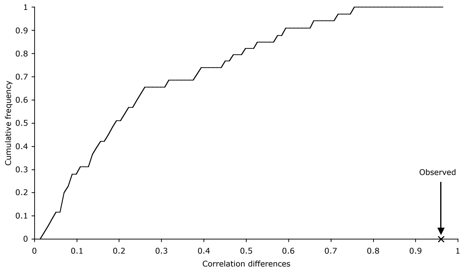
Figure 1.1 Example of null distribution of pairwise differences between correlation coefficients. “Observed” is the actual difference for the species pair Bathyphanes pallida and Gea heptagon associated with NMS axis 1 (S1) in the sloped field.
