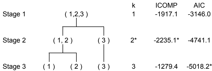
Figure C.2 Optimal decision tree classifier for habitat architecture data. ICOMP and AIC values for stages two and three are based on the model with varying means and varying variance/covariance (Model 1).
