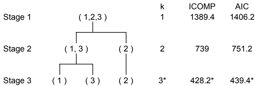
Figure C.1 Optimal decision tree classifier for plant species data. ICOMP and AIC values for stages two and three are based on the model with varying means and varying variance/covariance (Model 1).
