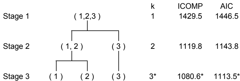
Figure C.3 Optimal decision tree classifier for spider species data. ICOMP and AIC values for stages two and three are based on the model with varying means and varying variance/covariance (Model 1).
