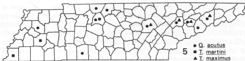
Figure 5. Known distribution in Tennessee of selected stunt nematodes ( Quin- isulcius , Tylenchorhynchus spp.).
