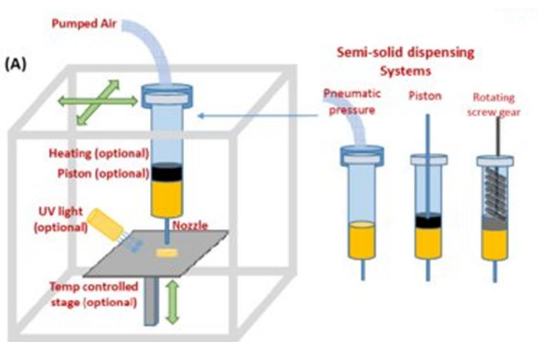
Figure 1. Direct Ink Write Additive Manufacturing schematic [42].
