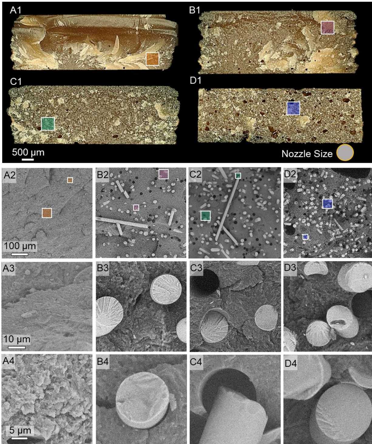
Figure 26. Micrographs of fracture surfaces from flexure testing of axially printed samples. (A) 0 vol% GF, (B) 10 vol% GF, (C) 20 vol% GF, and (D) 30 vol% GF. Set X1) is taken using optical Keyence microscopy at 50x while X2-4) are from SEM at 500x, 5,000x, and 10,000x respectively. The highlighted boxes in X2 correlate to X3 (larger) and X4 (smaller) of the same series.
