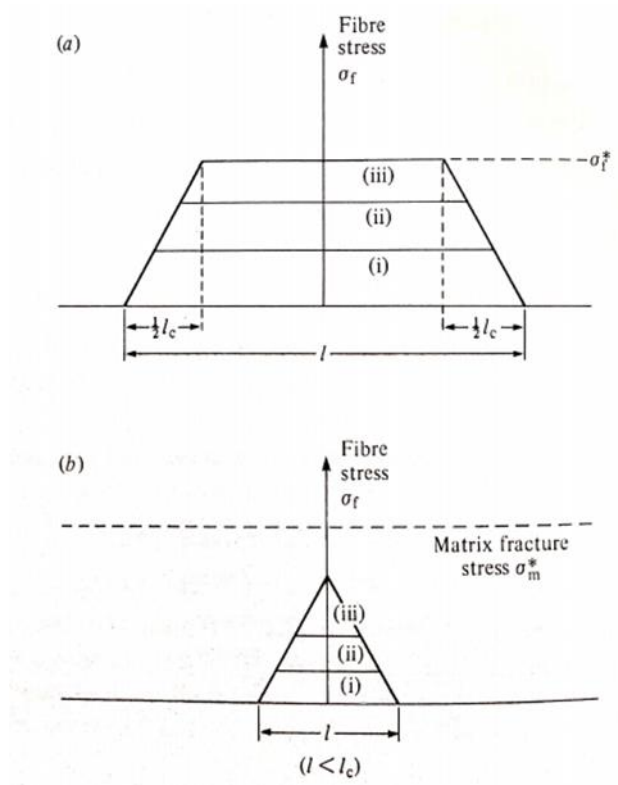
Figure 9. Load transference and fiber length. The critical fiber length, when applied force is primarily carried by the fibers, is determined by the fiber strength, diameter, and fiber-matrix interface [73].
