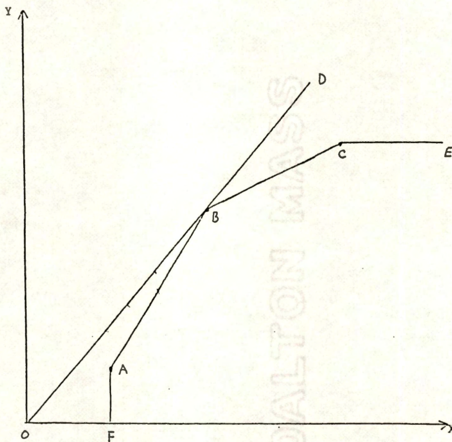
Figure 2. Example of the Changes in the Shape of the Production Frontier as the Scale Properties of the Frontier Become Less Restrictive.
