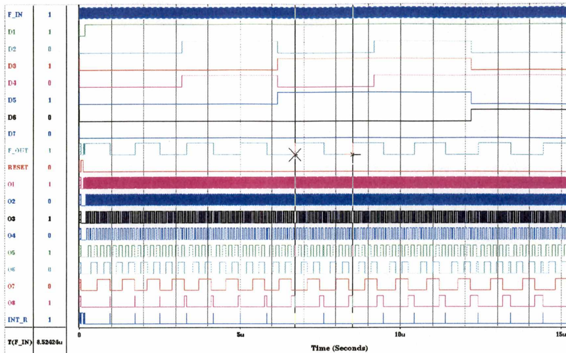
Figure 4.2: Pre-layout simulation of programmable divider Source files: Appendix A.2, A.3
