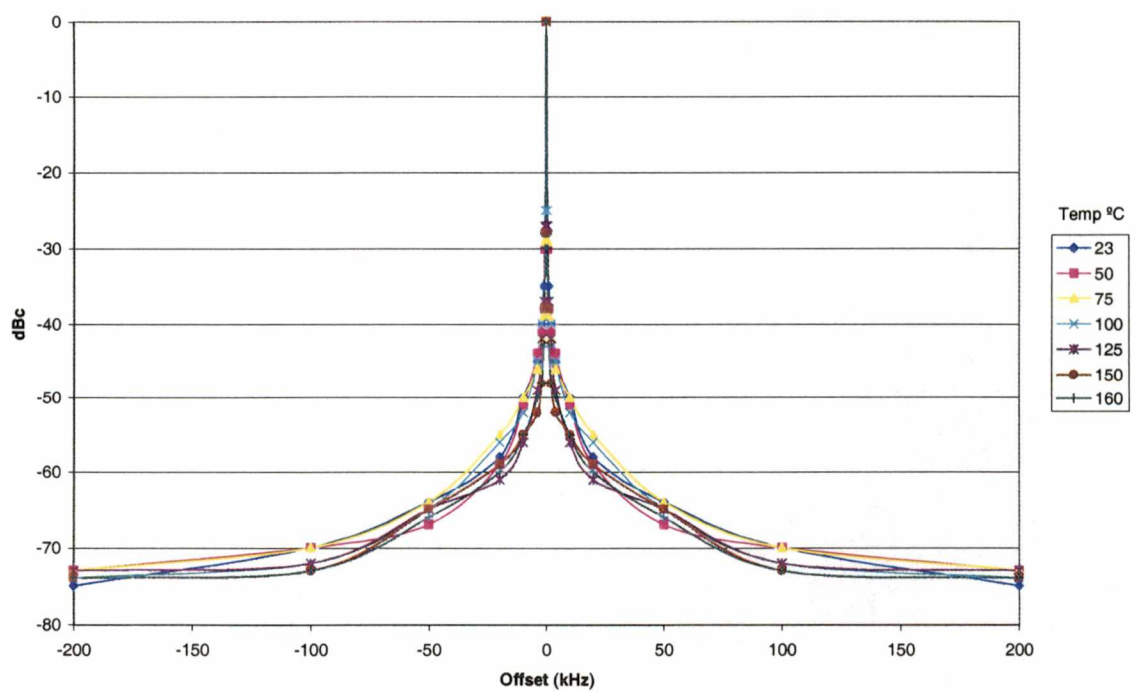
Figure 5.36: PLL 300 MHz output spectrum over temperature
