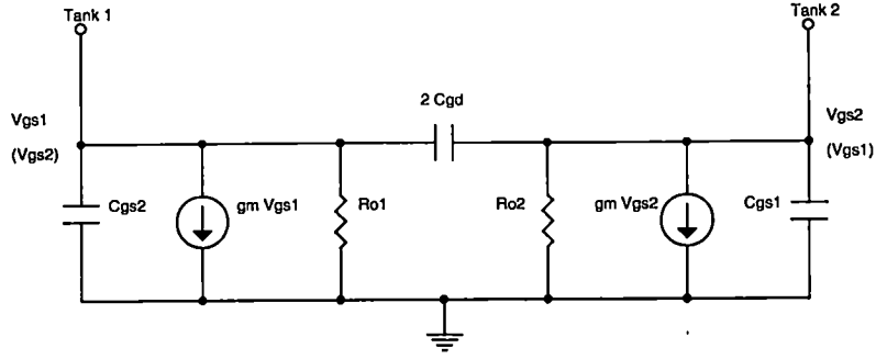
Figure 3.5: Hybrid-PI model for cross-coupled differential transistor pair
